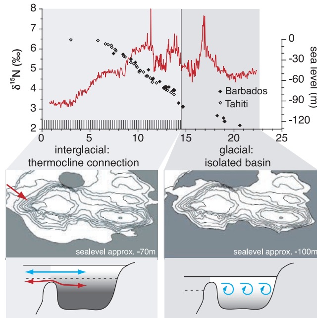
Figure 5. Deglacial change of the local conditions in Cariaco Basin due to sea level rise. Sea level data are from Fairbanks [1989] and Bard et al. [1990] (Barbados) and Bard et al. [1996] (Tahiti). The hatched bar indicates laminated sediments, reflecting the prevalence of anoxic bottom water.
