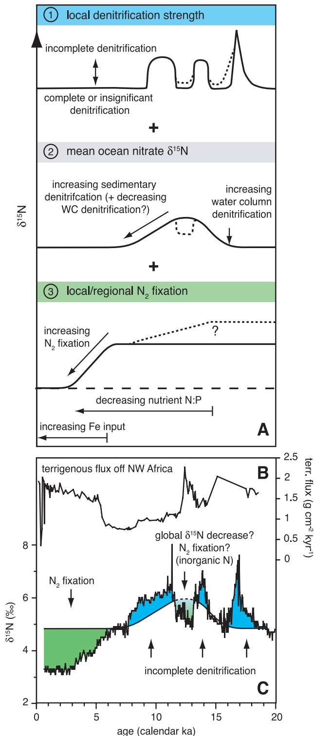
Figure 8. (a) Conceptual drawing of the effects thought to cause the observed \delta^{15}N trends in Cariaco Basin during terminations. Because of the variety of influences, the shape of different signals is not always clear: Potential inorganic N input would cause overestimation of the denitrification effect (dashed lines in 1); the timing and shape of the mean ocean nitrate signal (2) as well as potentially rapid changes in thermocline nitrate \delta^{15}N are currently not well constrained; if N_2 fixation increased before the mid-Holocene (dashed line in 3), processes 1 and 2 would have obscured this signal. (b) Excess ^{230}Th normalized terrigenous flux off NW Africa (ODP core 658C) [Adkins et al. , 2006], potentially representing Fe input to the tropical North Atlantic and the Caribbean. (c) Graphic representation of proposed influences on Cariaco Basin \delta^{15}N , subject to the uncertainties outlined above.
