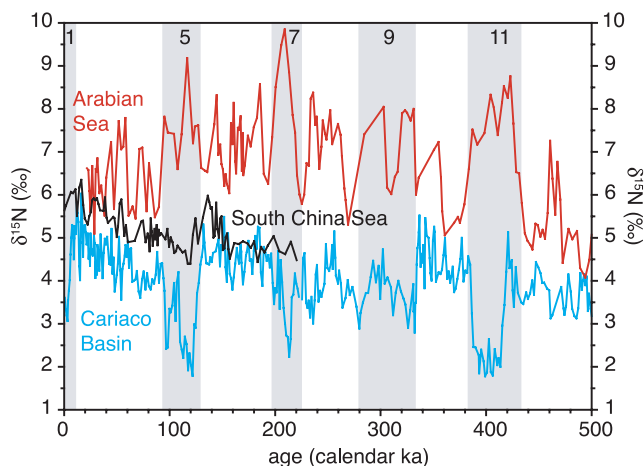
Figure 4. The long \delta^{15}\text{N} record from Cariaco Basin [Haug et al. , 1998] in comparison with records from the Arabian Sea (ODP core 722) [Altabet et al. , 1999] and the South China Sea (core 17954) [Kienast, 2000]. Shaded bars indicate interglacials, and numbers are marine isotope stages.
