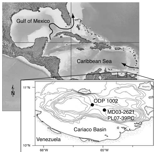
Figure 1. Map of the Cariaco Basin, located off Venezuela in the Caribbean Sea. Arrows depict major surface currents. Closed symbols correspond to the locations of the cores used for this study. Isobaths are in meters below sea level with spacing of 200 m except for upper 300 m where spacing is 100 m.
