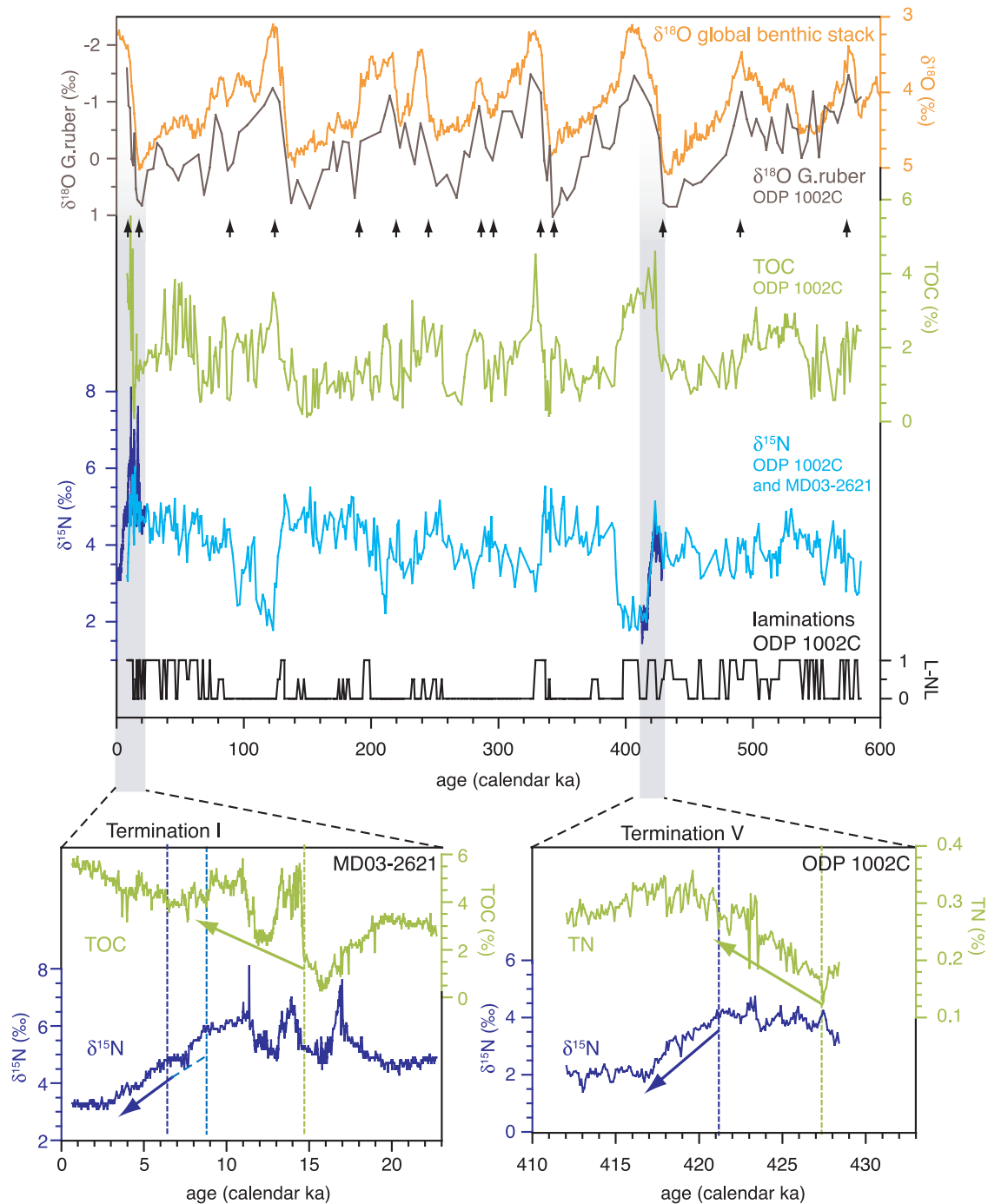
Figure 3. Cariaco Basin low- and high-resolution records. (top) The \delta^{18}\text{O} of G. ruber [Peterson et al., 2000] and global benthic \delta^{18}\text{O} stack [Lisiecki and Raymo, 2005] used for tuning (black arrows are tie points). Low-resolution TOC and \delta^{15}\text{N} records and lamination data (1 = laminated) are from Haug et al. [1998]. (bottom) High-resolution data from core MD03-2621 and ODP core 1002C. Dashed lines indicate onset of deglacial change (ambiguous for \delta^{15}\text{N} during Termination I).
