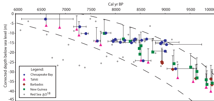
Figure 3. Chesapeake sea level curve compared to those from Tahiti [Bard et al., 1996], Barbados [Fairbanks, 1989; Fairbanks et al., 2005], and New Guinea [Ota and Chappell, 1999], all corrected for tectonic and isostatic adjustment; and isotopically-derived sea level from Red Sea isotope record [Siddall et al., 2003]. Horizontal bars signify 2- \sigma age range for CB samples. Vertical bars represent coral depth range (7 m), CB marsh and oyster facies (1–2 meters \approx thickness of the symbol), Red Sea isotopic uncertainty \pm 12 m not shown for clarity. Dashed lines qualitatively bracket first-order sea level curve.
