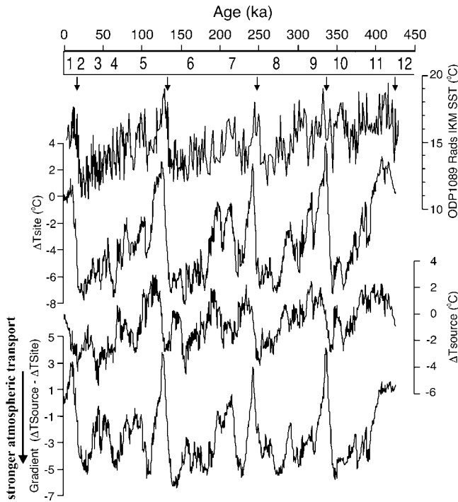
Figure 5. Comparison between SST record of Site 1089 and \Delta T_{\text{source}} , \Delta T_{\text{site}} and their gradient from the Vostok ice core, as derived [Vimeux et al. , 2002] from deuterium and oxygen isotopes. Vostok data are plotted on the EPICA Dome C (EDC) timescale [EPICA Community Members, 2004]. Arrows mark the approximate position of cooling rebounds at glacial terminations.
