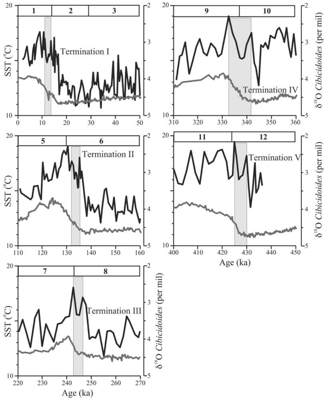
Figure 4. Detail of the SST (in black, this paper) and \delta^{18}\text{O} Cibicoides (in gray [Hodell et al. , 2003a]) evolution at Site 1089 during last five terminations. Cooling events at terminations are highlighted (gray boxes), while Marine Isotopic Stage numbers, according to the Lisiecki and Raymo [2005] chronology, are indicated in bold.
