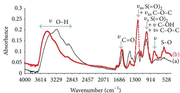
FIGURE 3: ATR FT-IR spectra of GY785 DR (a) and GY785 DRS sulfated in BMIImCl medium (b).
