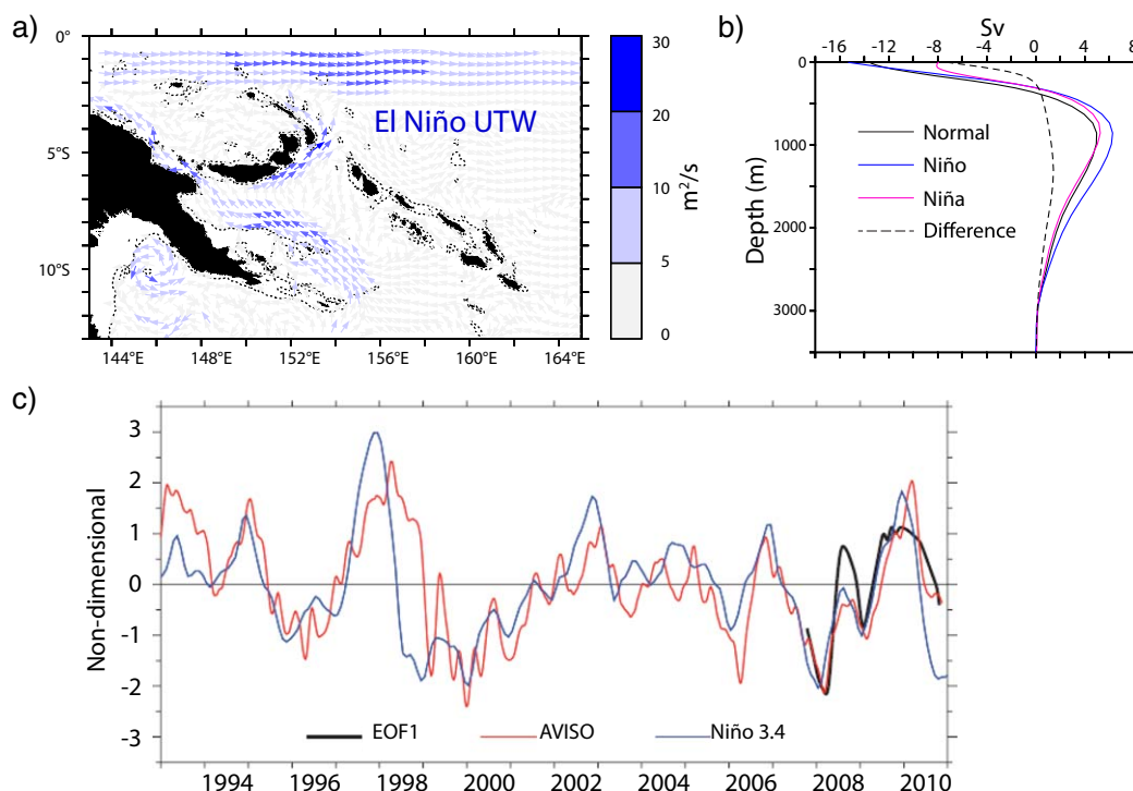
Figure 13. Interannual variability of the Solomon Sea circulation. (a) Circulation anomalies vertically integrated in the upper thermocline ( 23.3 < \sigma_\theta < 25.7 \text{ kg m}^{-3} ) during El Niño, from composites in the 1/12^\circ simulation. (b) Depth cumulated transport (Sv from 3500 m) during the winter (November–February) at the Solomon Sea southern entrance ( 9.8^\circ\text{S} ) for the mean state (black line), El Niño state (blue line), and La Niña state (magenta line). The difference between El Niño and La Niña is plotted as a black-dashed line [see Melet et al. , 2013]. (c) Time series of the smoothed Solomon Sea equatorward geostrophic surface transport per unit depth from Aviso altimetric data (red line), and the equatorward transport per depth by the dominant EOF of upper layer transport computed from glider data (black line). The Niño 3.4 sea surface temperature anomalies are also shown (blue line) to indicate variability associated with ENSO. [adapted from Davis et al. , 2012].
