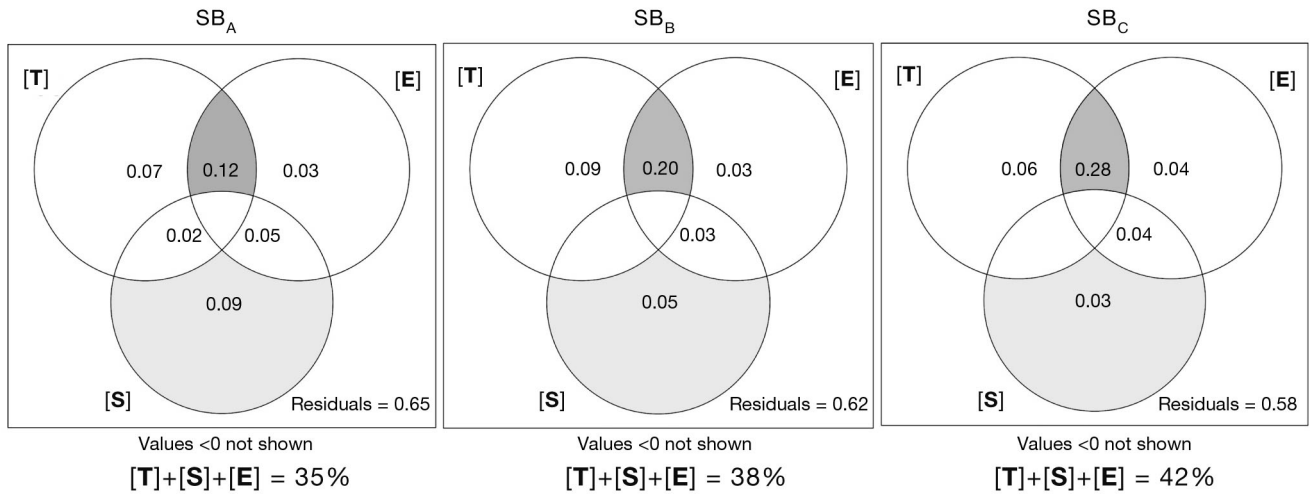
Fig. 8. Venn diagrams illustrating the result of variance partitioning of the macrofauna time series at SB A , SB B , and SB C with respect to environmental (physical and biological variables), spatial (location along shore), and temporal (distance-based Moran's eigenvector maps [dbMEMs]) explanatory variables. Variation explained is expressed as a percentage (%) based on adjusted R 2 . [T]: selected temporal variables, [S]: spatial location, [E]: environmental variables, Residuals: unexplained variation
