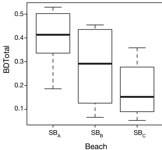
Fig. 6. Total \beta -diversity (BDTotal) across space and time at the 3 beaches (SB A , SB B and SB C ). Box plots show the median (line in box), the first and third quartiles (hinges), and the most extreme data points which are 1.5 times the interquartile range from the box (whiskers)
