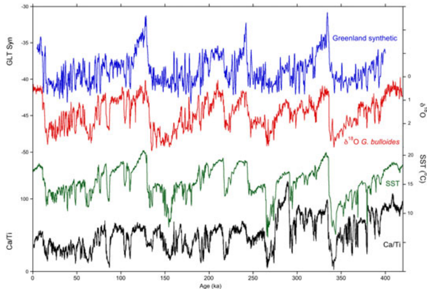
Figure 3. Ca/Ti (black; log scale), alkenone sea surface temperature ( Uk'_{37} ; green) [ Martrat et al., 2007 ], \delta^{18}O of G. bulloides (red) [ de Abreu et al., 2005; Vautravers and Shackleton, 2006 ] from the combined record of Core MD01-2444 (0–194 ka) and MD01-2443 (194–420 ka), and the Greenland synthetic \delta^{18}O record (blue) [ Barker et al., 2011 ]. There are strong similarities of the orbital and suborbital variations among the records.
