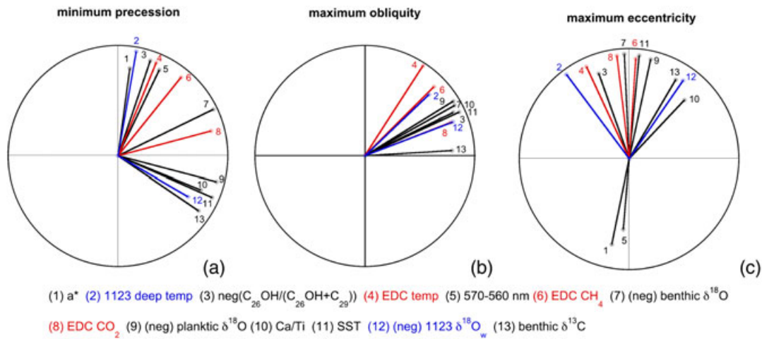
Figure 11. Phase wheels for proxy records with respect to (a) minimum precession, (b) maximum obliquity, and (c) maximum eccentricity. The length of the vector is the coherency from 0 (center) to 1 (circle). Numerical values of coherency and phase values are given in Table 1. Iberian Margin proxies are black, ice cores are blue, and Site 1123 is red. The signs of oxygen isotopes records and alcohol index are inverted.
