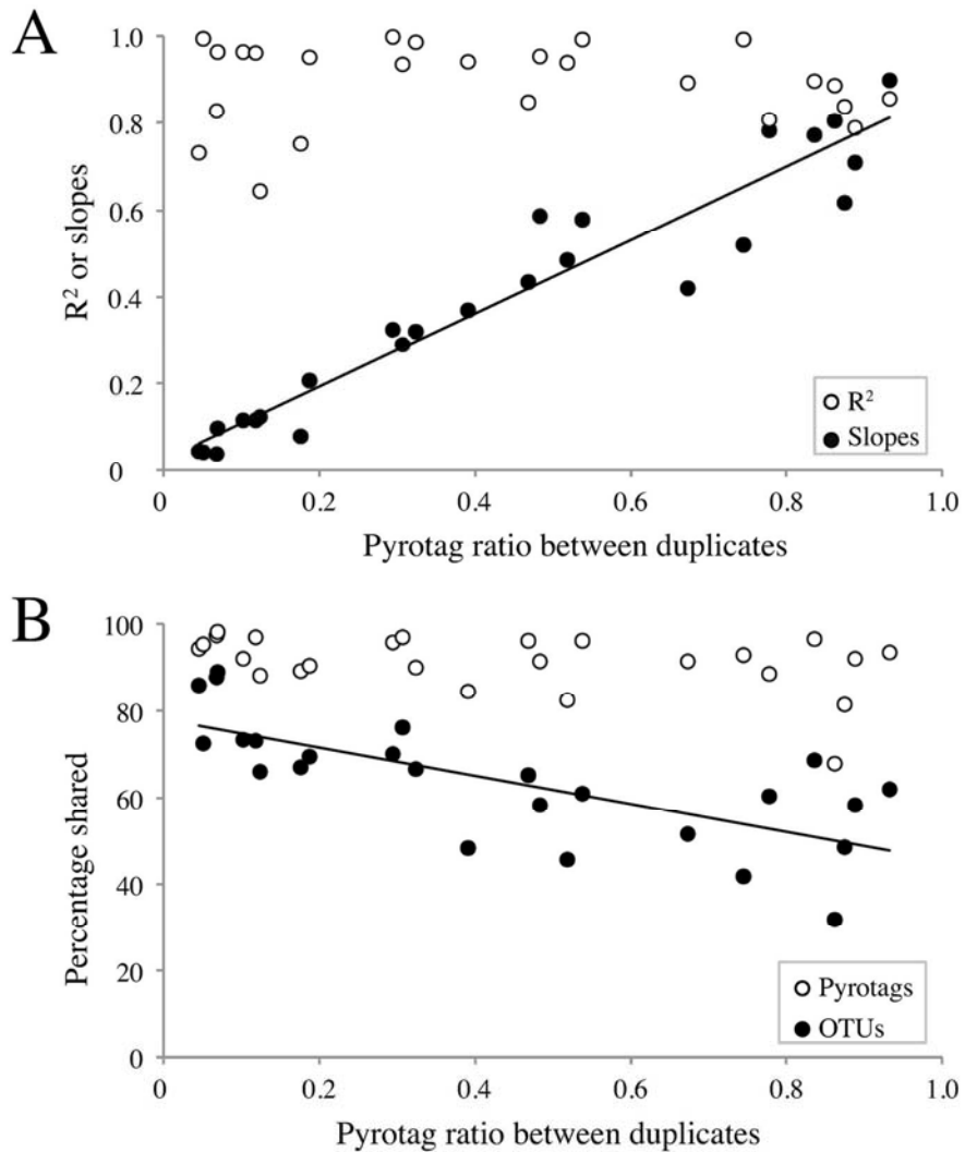
Fig. 1. Summary of the comparison of duplicated 454-samples ( n=25 ) shown in relation to the pyrotag ratio between duplicates. A. Statistics of the linear regressions between the OTU abundance in each duplicate: R^2 coefficients (white dots) and slope values (black dots; regression line shown). B. Percentage of OTUs shared in duplicate pairs (black dots; regression line shown) and percentage of pyrotags within these shared OTUs (white dots). These later percentages apply to the pair with less pyrotags. 133x141mm (300 x 300 DPI)
