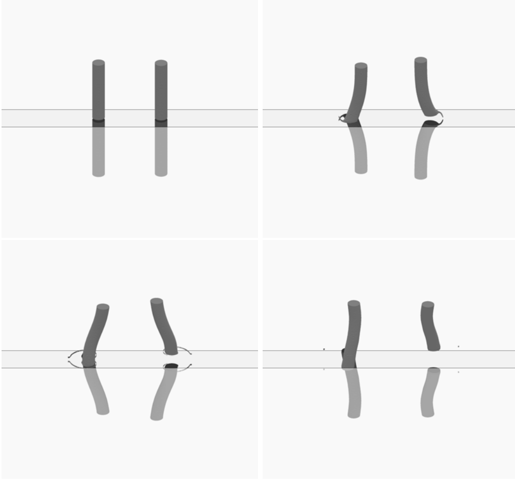
FIGURE 25. Flow evolution for symmetric finite core hetons with \varrho = 0.1 , d_y = 0.1 , and \ell_z = 0.1 at t = 0, 10, 15 , and 25 .
