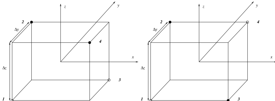
FIGURE 1. Geometry for head-on interactions: Symmetric configuration (left), Anti-symmetric configuration (right). Filled circles indicate the centre the positive pole, un-filled circles indicate the centre of the negative poles. \Delta z = 2z_{init} , \Delta y(t = 0) = 2y_{init} . Numbers are the poles labels.
