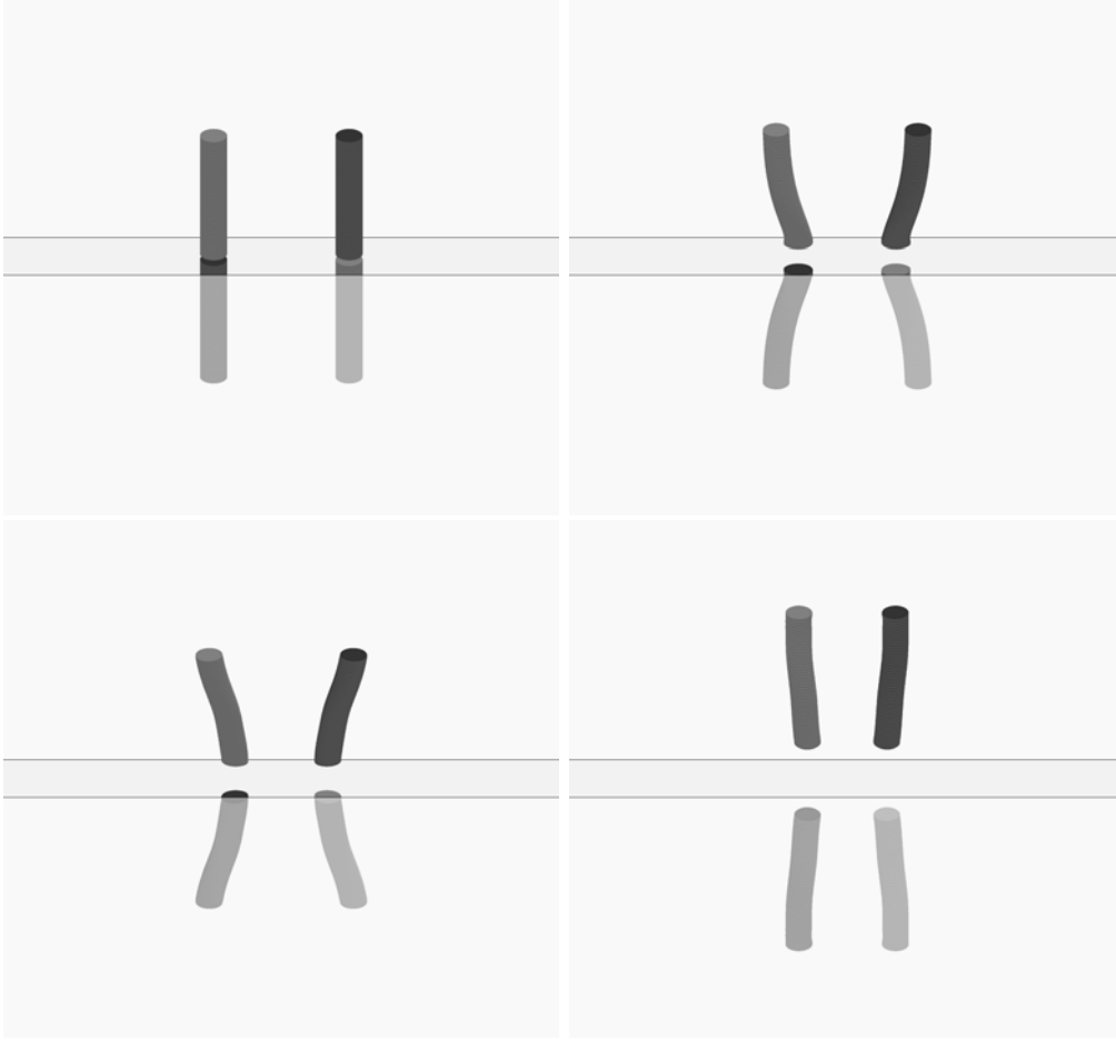
FIGURE 26. Flow evolution for anti-symmetric finite core hetons with \varrho = 0.1 , d_y = 0.1 , and \ell_z = 0.1 , at t = 0, 10, 15 and 40 .
