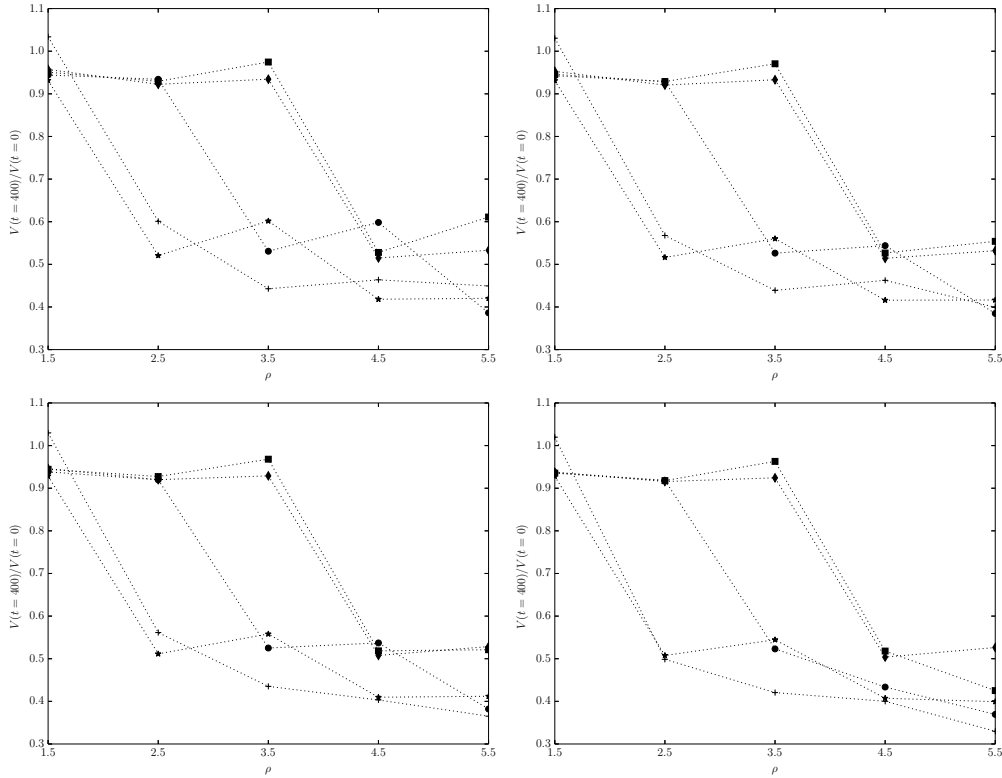
FIGURE 17. Ratio of the volume of the 4 biggest vortices at t = 400 over the initial volume for d_y = 0.1 , 1.5 \leq \rho \leq 5.5 and ell_z = 0.5 (+), 1 ( \star ), 1.5 ( \bullet ), 2 ( \blacksquare ), 2.5 ( \blacklozenge ) Figures are organised as follows. Top left: largest vortex. Top right: second largest vortex. Bottom left: third largest vortex. Bottom right: fourth largest vortex.
