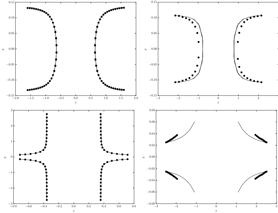
FIGURE 24. Top view of the trajectory of the poles centres for finite core hetons ( \bullet ) and point vortices (solid line). Top left: Symmetric case with \rho = 0.5 , \ell_z = 1.5 and d_y = 1 . Top right: Symmetric case with \rho = 1.5 , \ell_z = 1 and d_y = 0.5 . Bottom left: Anti-symmetric case with \rho = 0.5 , \ell_z = 1.5 and d_y = 1 . Bottom right: Anti-symmetric case with \rho = 1.5 , \ell_z = 1 and d_y = 0.1
