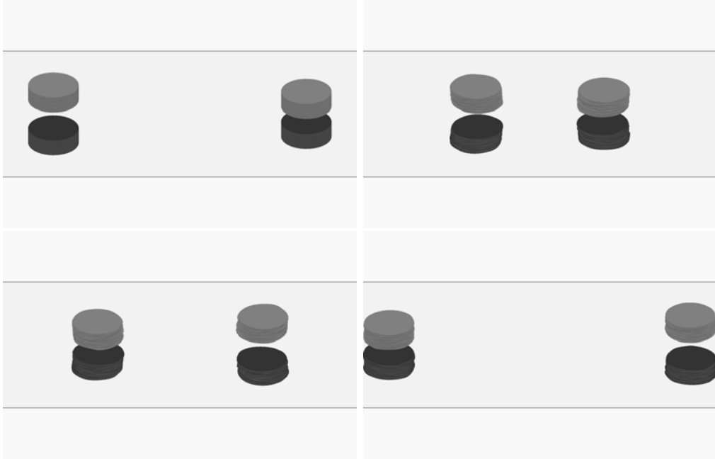
FIGURE 11. Flow evolution for symmetric finite core hetons with \rho = 1.5 , d_y = 0.5 , and \ell_z = 1.5 . Figure are ordered in increasing time top-left, top-right, bottom-left, bottom-right. Times displayed are t = 0 , t = 50 , t = 100 , and t = 150 . Vortices are viewed orthographically at an angle of 60^\circ from the vertical. The front and back panels indicate the side of a virtual viewing square box centred around the vortices. Hetons reverse velocity (label \triangleleft , in table 1).
