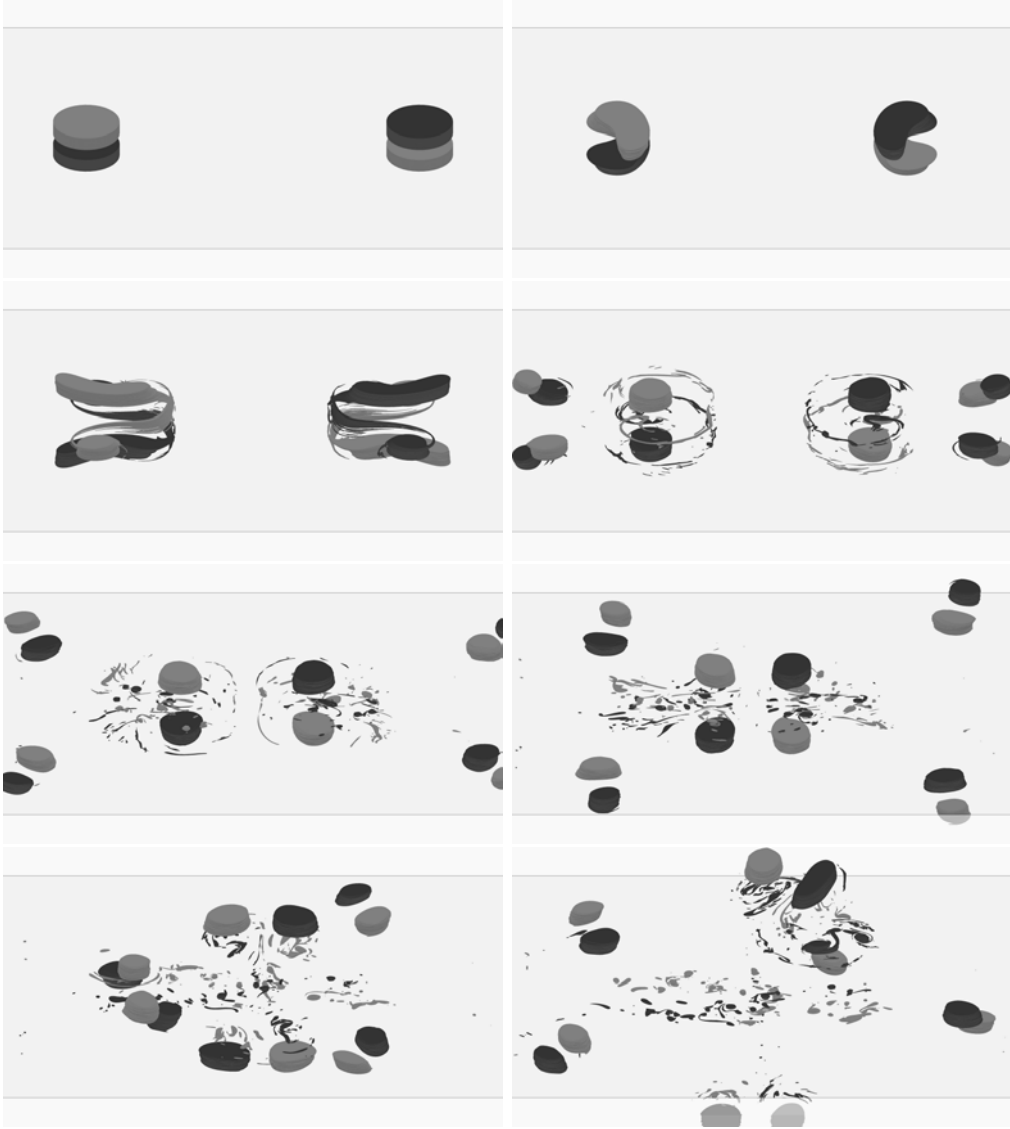
FIGURE 23. Flow evolution for anti-symmetric finite core hetons with \varrho = 5 , d_y = 0.25 , and \ell_z = 0.5 at t = 0, 12.5, 25, 50, 75, 100, 135.5 , and 190 . Hetons break baroclinically into 2 dipoles and 4 hetons. Dipoles eventually escape. (label \bar{\Delta} , in table 2).
