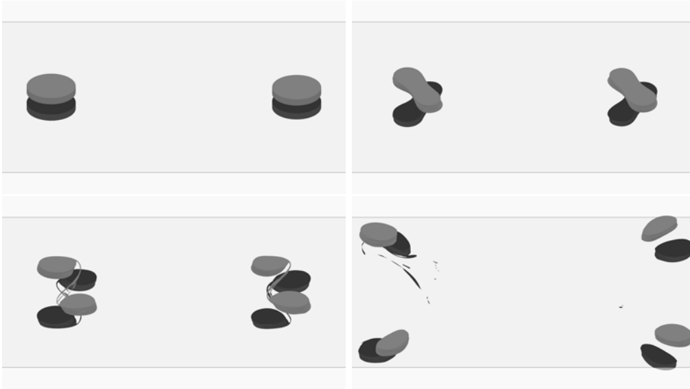
FIGURE 13. Flow evolution for symmetric finite core hetons with \varrho = 3.5 , d_y = 0.1 , and \ell_z = 1.5 . Times displayed are t = 0, 17.5, 50 , and 87.5 . Hetons break into 4 hetons which reverse trajectory (label \times , in table 1).
