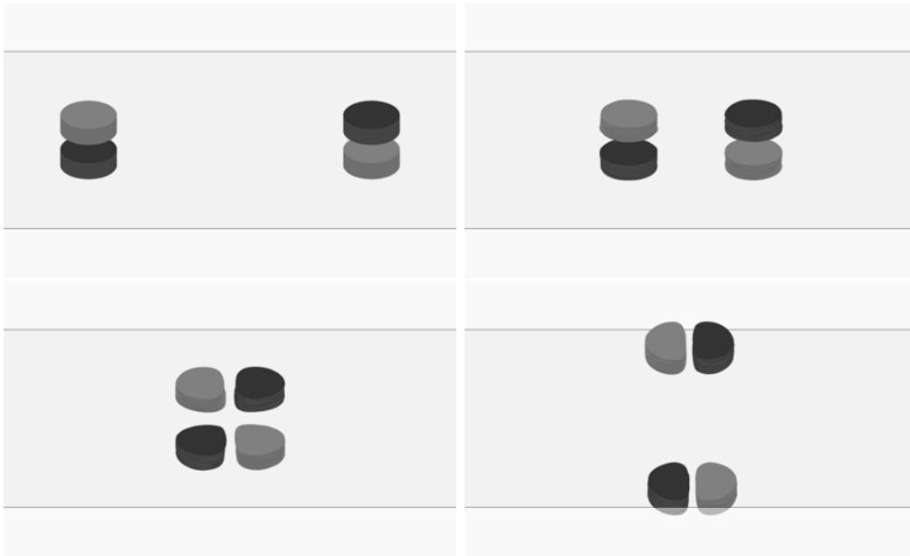
FIGURE 19. Flow evolution for anti-symmetric finite core hetons with \varrho = 1.5 , d_y = 0.1 , and \ell_z = 1 at t = 0 , t = 95 , 110 , and 120 . Hetons interact and poles escape as dipoles (label \square , in table 2).
