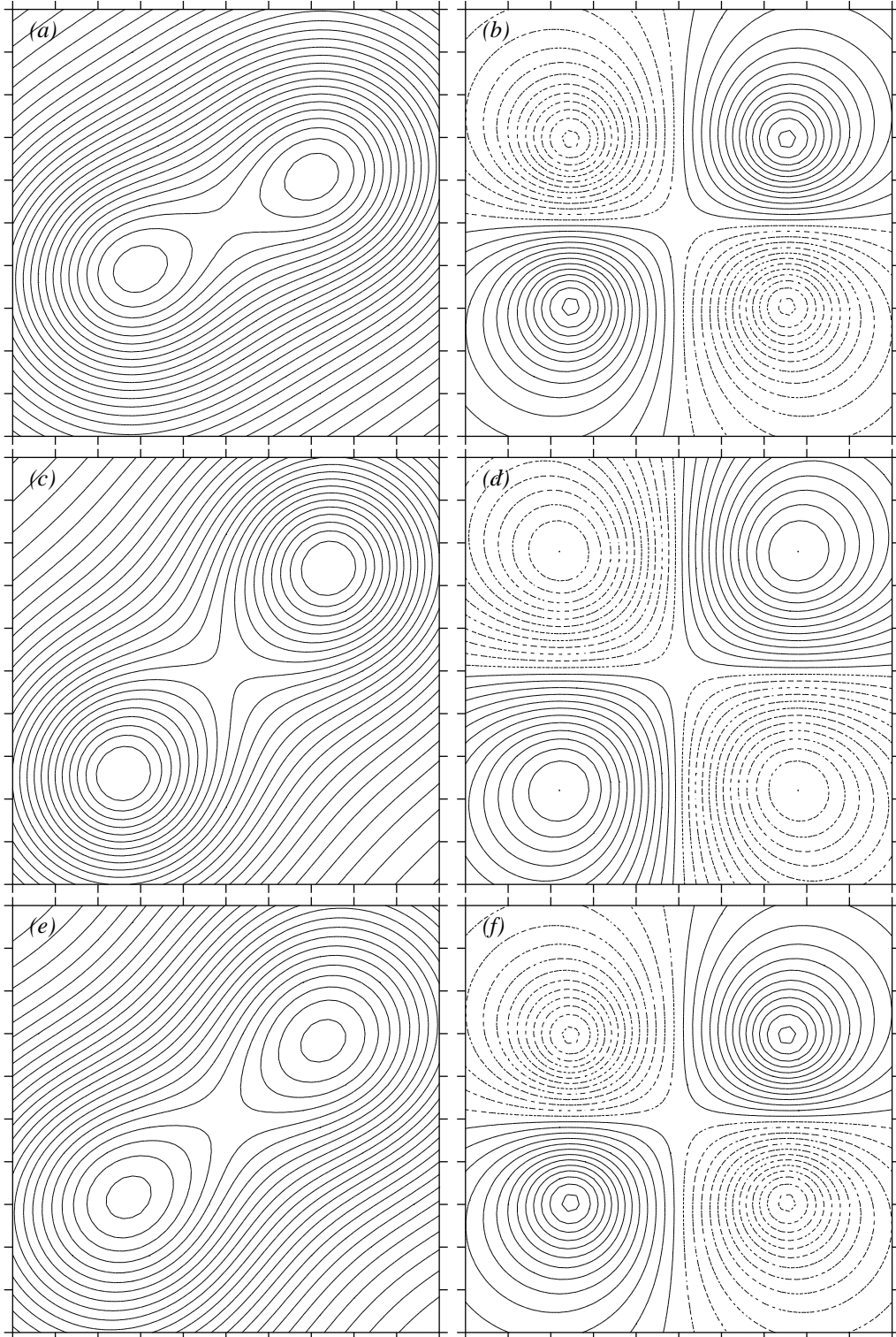
FIGURE 3. Streamlines for (a, b) : \Delta x = 2, \Delta y = 1, \Delta z = 1.5 and -2 \leq x, y \leq 2, z = -2 (a), and z = 0 (b). (c, d) : \Delta x = 1, \Delta y = 1, \Delta z = 1 and -1 \leq x, y \leq 1, z = -1 (c), and z = 0 (d). (e, f) : \Delta x = 2, \Delta y = 1.5, \Delta z = 1 and -2 \leq x, y \leq 2, z = -2 (e), and z = 0 (f).
