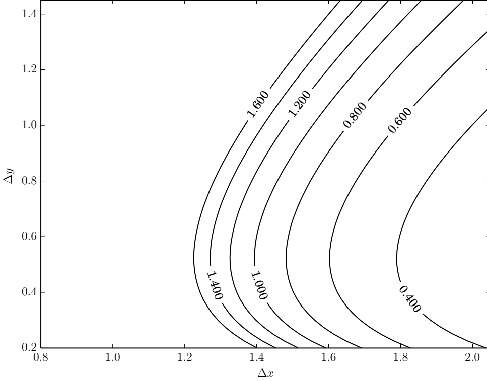
FIGURE 5. Iso-values of \left| \frac{v_1}{u_1} \right| for 0.8 \leq \Delta x \leq 2.05 and 0.2 \leq \Delta y \leq 1.45 .
