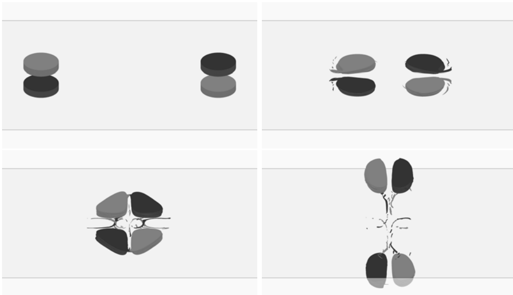
FIGURE 20. Flow evolution for anti-symmetric finite core hetons with \varrho = 2.5 , d_y = 1 , and \ell_z = 1 at t = 0 , 20 , 30 and 45 . Hetons sheds some debris and recombine as dipoles which escape. (label \times , in table 2).
