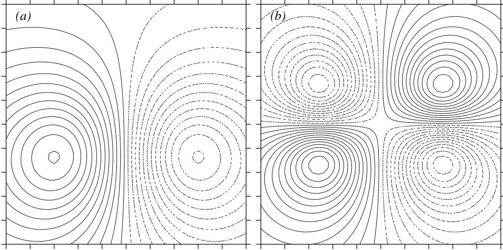
FIGURE 6. Streamlines for (a, b) : \Delta x = 2, \Delta y = 1, \Delta z = 1.5 and -2 \leq x, y \leq 2, z = -2(a) , and z = 0(b)
