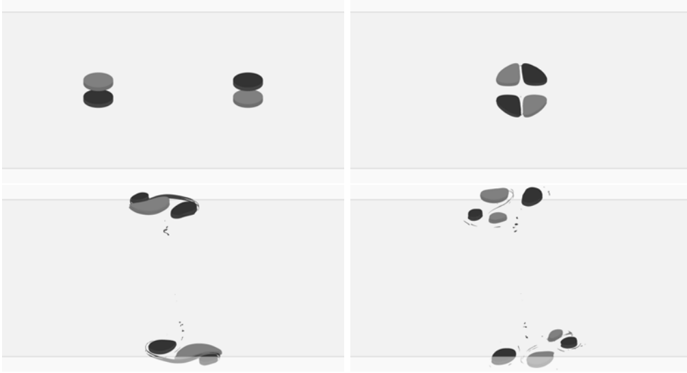
FIGURE 21. Flow evolution for anti-symmetric finite core hetons with \varrho = 3.5 , d_y = 0.75 , and \ell_z = 2 at t = 0, 50, 100 , and 125 . Hetons interact, poles escape as dipoles which undergo a destructive interaction (label \bar{\triangleleft} , in table 2).
