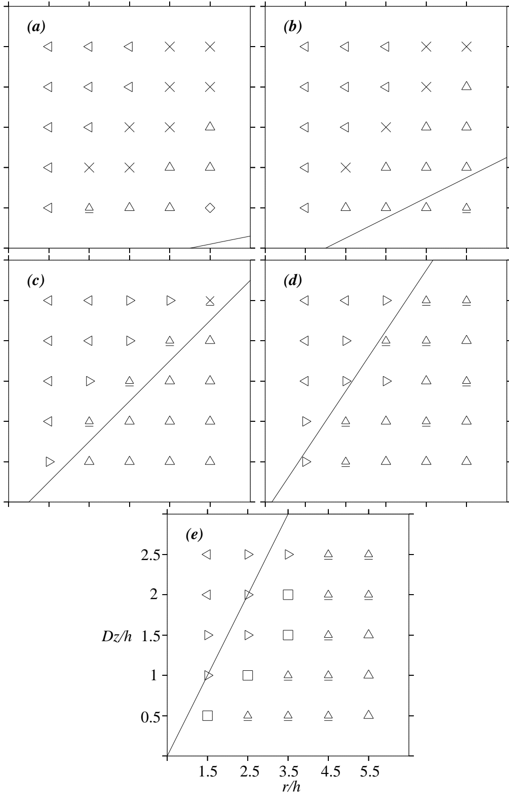
FIGURE 10. Finite core, symmetric hetons. Regimes in the plane \rho - \ell_z for (a), d_y = \Delta y / r = 0.1 , (b) 0.25, (c) 0.5, (d) 0.75, and (e) 1. The solid lines indicate the threshold \Delta y / \Delta z = 1 . Legends and axis-labels are all identical are defined in figure (e). The meaning of all symbols is defined in table 1. An underlined symbol indicates that the vortices produced by the first main interaction experience further strong interaction as they reverse velocity or escape.
