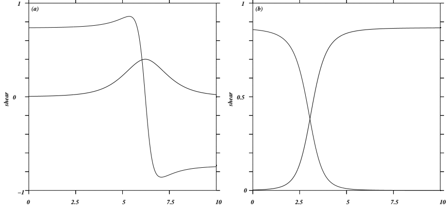
FIGURE 27. Shear experienced by pole 1 versus time for a symmetric pair of point vortex hetons with, at t = 0 , (a) : \Delta x = 5 , \Delta y = 0.75 and \Delta z = 1 and (b) : \Delta x = 5 , \Delta y = 1 , \Delta z = 0.5 . The thin solid line represents \partial u/\partial z while the thick solid line represents \partial v/\partial z .
