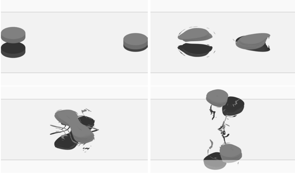
FIGURE 15. Flow evolution for symmetric finite core hetons with \varrho = 2.5 , d_y = 1 , and \ell_z = 1 at t = 0, 17.5, 40 , and 62.5 . Hetons shed some debris and escape. (label \square , in table 1).
