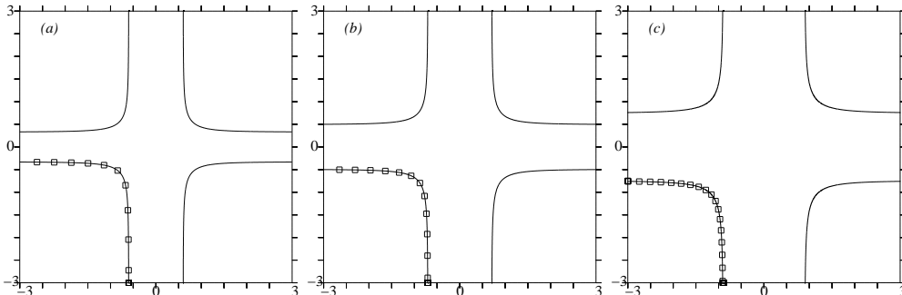
FIGURE 4. Top view of the trajectories of the ‘anti-symmetric’ vortices for: y_{init}/z_{init} = 2/3 (left), y_{init}/z_{init} = 1 (centre), y_{init}/z_{init} = 2 (right). The square symbols label time by indicating the location of the pole 1 every \Delta t = 1 .
