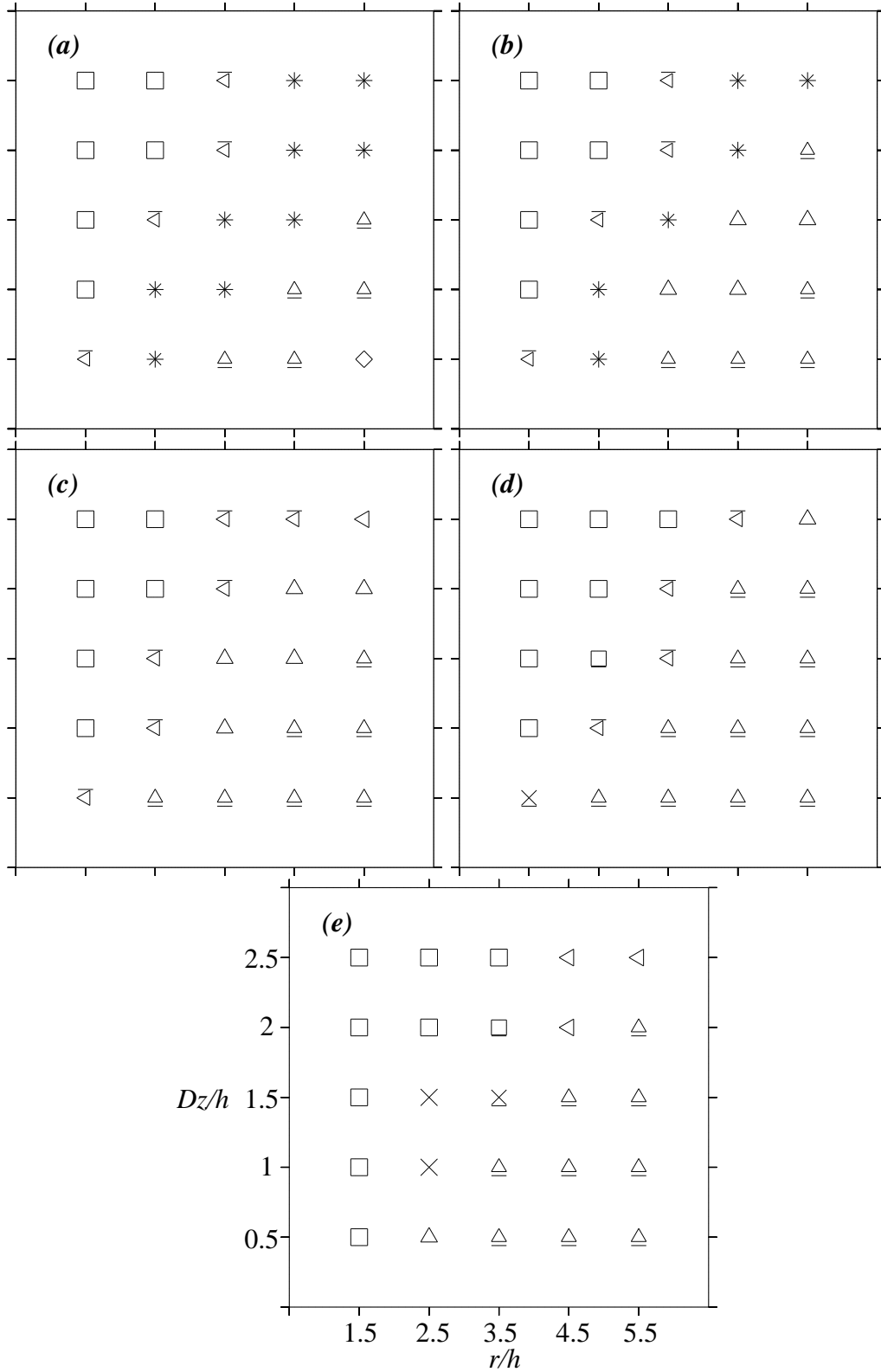
FIGURE 18. Finite core, anti-symmetric hetons. Regimes in the plane \varrho - \ell_z for (a), d_y = \Delta y/r = 0.1 , (b) 0.25, (c) 0.5, (d) 0.75, and (e) 1. The meaning of all symbols is defined in table 2. An underlined symbol indicates that the vortices produced by the first main interaction experience further strong interaction as they escape. A barred symbol indicates that the original baroclinic instability only produces small debris.
