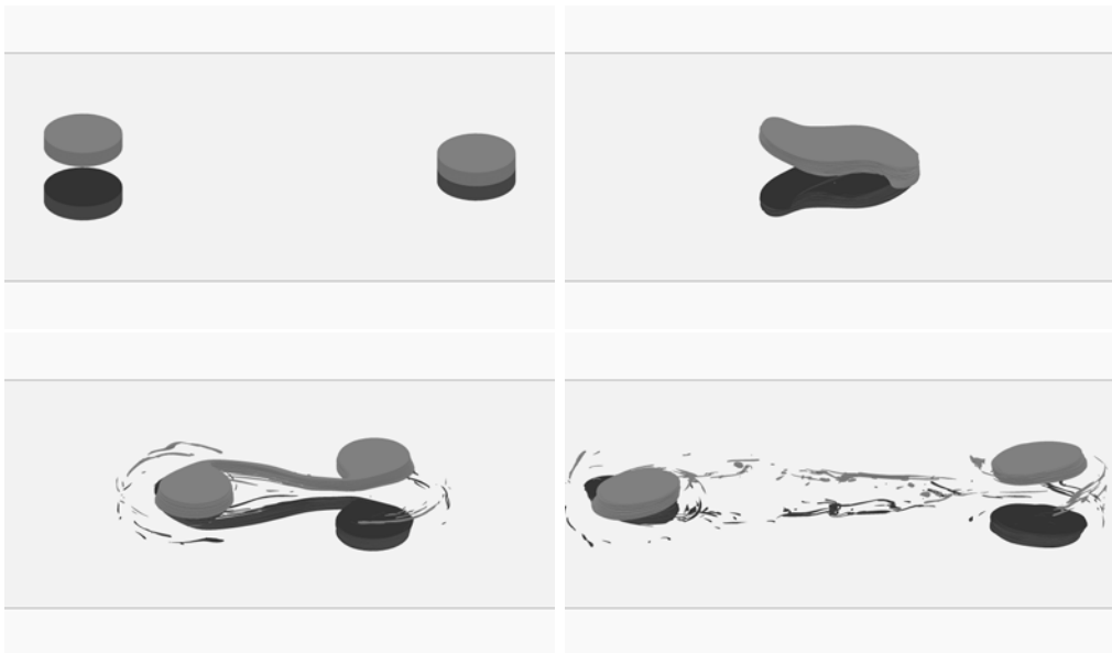
FIGURE 12. Flow evolution for symmetric finite core hetons with \rho = 2.5 , d_y = 1 , and \ell_z = 1.5 . Times displayed are t = 0 , t = 37.5 , t = 75 , and t = 100 . Hetons reverse velocity after temporary merger (label \triangleright , in table 1).
