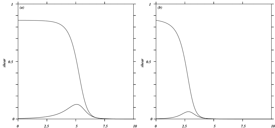
FIGURE 28. Shear experienced by pole 1 vs time for an anti-symmetric pair of point vortex hetons with, at t = 0 , (a) : \Delta x = 5 , \Delta y = 0.5 and \Delta z = 1 and (b) : \Delta x = 5 , \Delta y = 1 , \Delta z = 0.5 . The thin solid line represents \partial u/\partial z while the thick solid line represents \partial v/\partial z .
