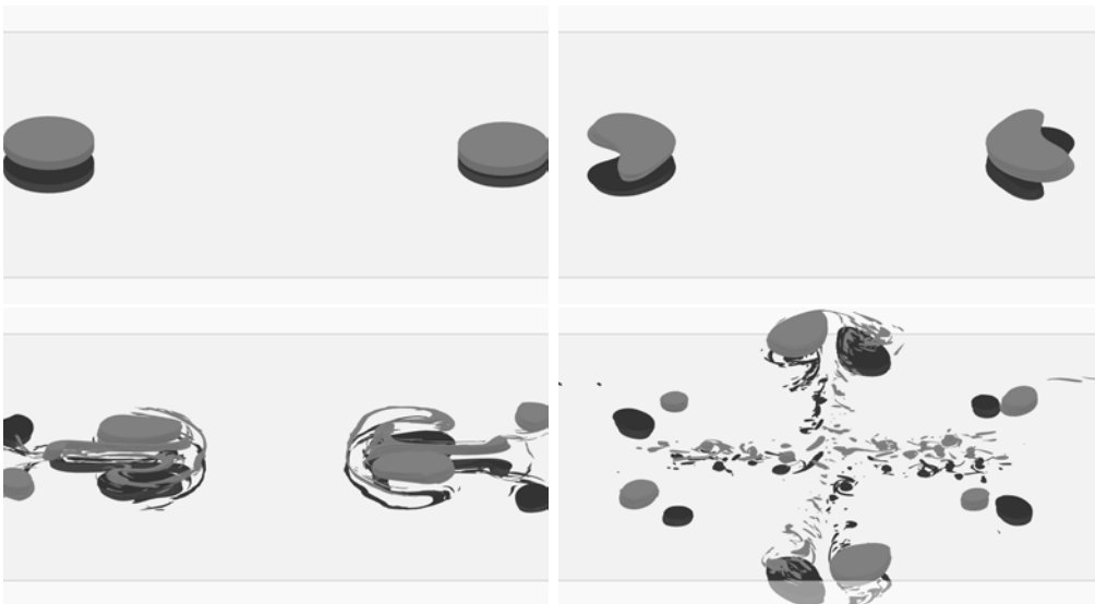
FIGURE 14. Flow evolution for symmetric finite core hetons with \varrho = 4.5 , d_y = 0.25 , and \ell_z = 1 at t = 0, 15, 50 and 162.5 . Hetons break into more than 4 hetons. The main two hetons escape. (label \triangle , in table 1).
