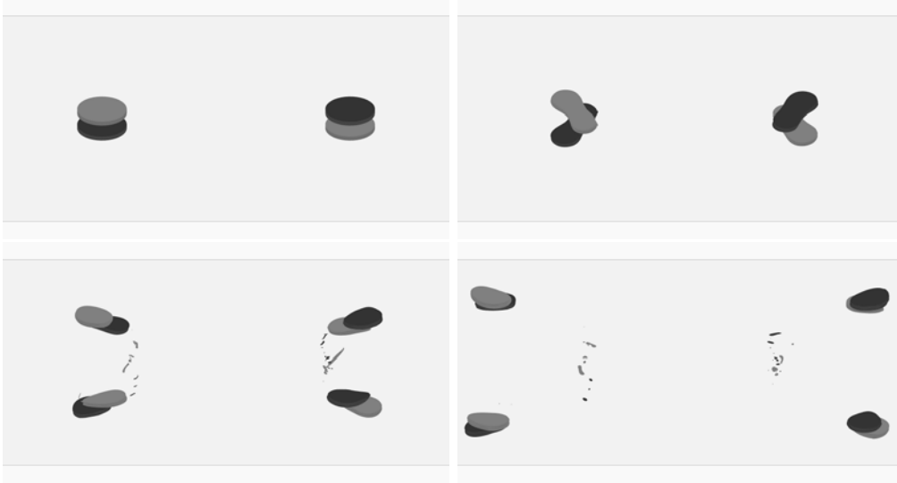
FIGURE 22. Flow evolution for anti-symmetric finite core hetons with \varrho = 5.5 , d_y = 0.1 , and \ell_z = 2.5 at t = 0, 50, 100, 150 . Hetons break baroclinically into 4 hetons then move away (label *, in table 2).
