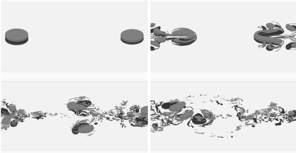
FIGURE 16. Flow evolution for symmetric finite core hetons with \varrho = 5.5 , d_y = 0.1 , and \ell_z = 0.5 at t = 0, 50, 125, 200 . (label \diamond , in table 1).
