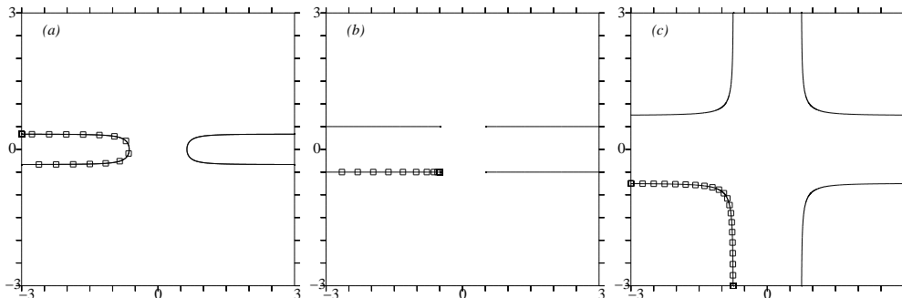
FIGURE 2. Top view of the trajectories of the ‘symmetric’ vortices for: y_{init}/z_{init} = 2/3 (left), y_{init}/z_{init} = 1 (centre), y_{init}/z_{init} = 2 (right). The square symbols label time by indicating the location of the pole 1 every \Delta t = 1 .
