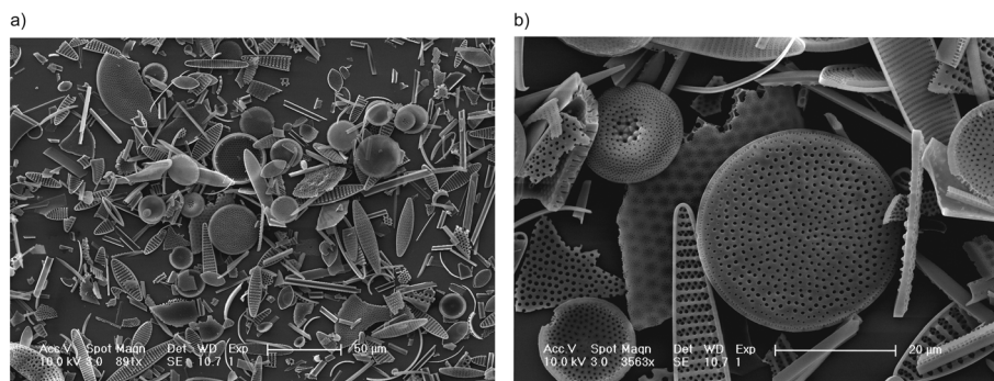
Figure 2. (a and b) SEM images showing the absence of lithogenic and organic particles in core samples of MD03-2601. Examples of samples used for stable isotope analyses of \delta^{30}\text{Si}_{\text{diat}} and \delta^{13}\text{C}_{\text{diat}} .
