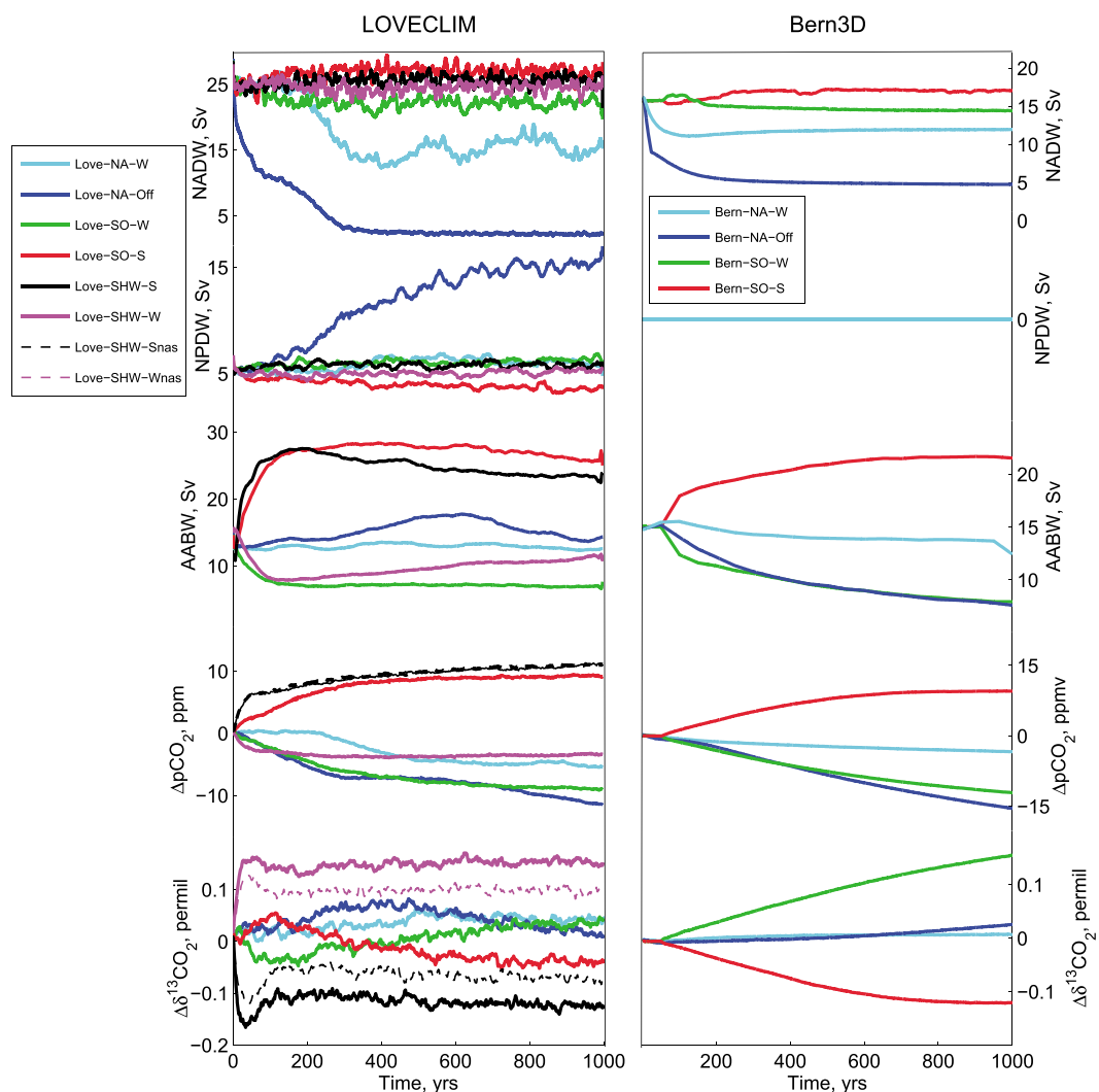
Figure 4. (top to bottom) Time series of NADW, NPDW, |AABW| (Sv), as well as pCO_2 (ppmv) and atmospheric \delta^{13}CO_2 (‰) anomalies for experiments performed with (left) LOVECLIM and (right) the Bern3D model. NADW and NPDW represent the maximum overturning stream function in the North Atlantic and the North Pacific, respectively. AABW is taken as the minimum of the global overturning stream function in the 80^\circ S - 60^\circ S region and its absolute value is shown. Experiments performed with both models and with weakened NADW (Love-NA-W and Bern-NA-W) are in cyan, NADW cessation (Love-NA-Off and Bern-NA-Off) are in blue, weakened AABW (Love-SO-W and Bern-SO-W) are in green, and strengthened AABW (Love-SO-S and Bern-SO-S) are in red. Experiments performed with LOVECLIM only: weaker (Love-SHW-W, magenta) and stronger (Love-SHW-S, black) Southern Hemispheric westerlies as well as experiments in which the CO_2 air-sea gas exchange is not impacted by the wind stress changes (Love-SHW-Snas, dashed black and Love-SHW-Wnas, dashed magenta).
