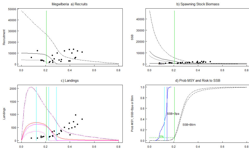
Figure 5.4.6.10. Megrim, long-term projections from EqSim including stochastic annual recruitment: (a) recruitment vs. F, (b) SSB vs. F, (c) yield (i.e. landings) vs. F, (d) probability of SSB < B_{lim} and B_{pa} vs. F (for this plot it is assumed B_{lim}=650 t , and B_{pa}=1.4 B_{lim} ). In all panels, the green vertical line is at F=0.21 (the F value that gives 5% probability of SSB < B_{lim} ). The left-most vertical line in panel (c) is at F=0.12 (the F value that maximizes long-term average landings). Historical estimates from the benchmark assessment are represented as dots in panels (a), (b), (c).
