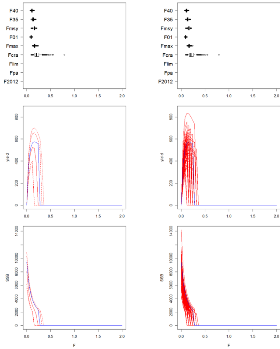
Figure 5.4.6.6. Megrim: results for Hockey-stick stock-recruitment function.
