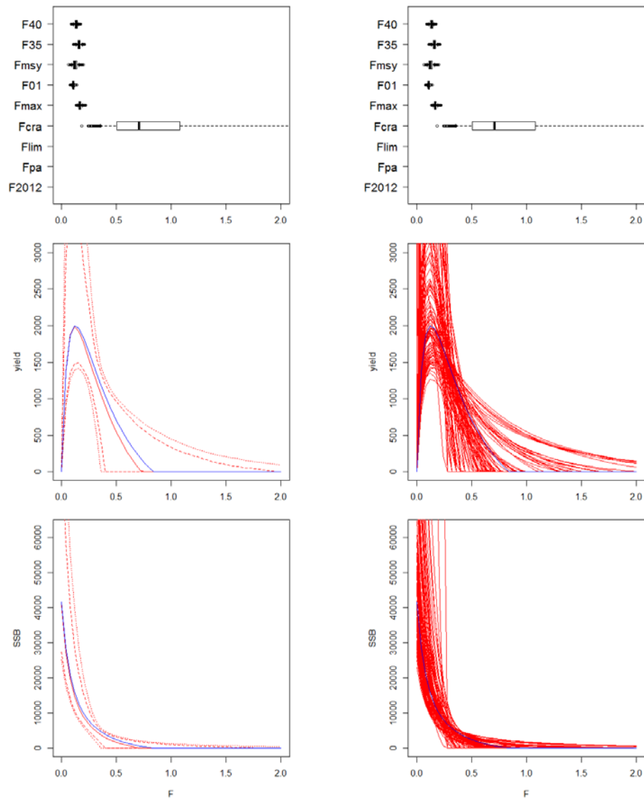
Figure 5.5.6.5. Four-spot megrim: results for Beverton–Holt stock-recruitment function.
