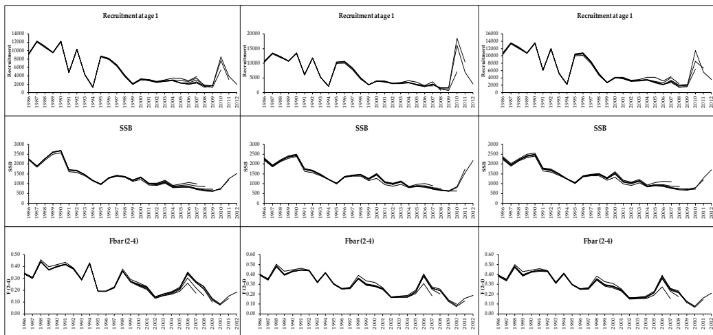
Figure 5.4.4.7. Megrim ( L. whiffiagonis ) (Divisions VIIIc and IXa). Retrospective patterns of WGMM2013 assessment and sensitivity analysis to catchability independent of stock size and catchability dependent on stock size for ages <3.
