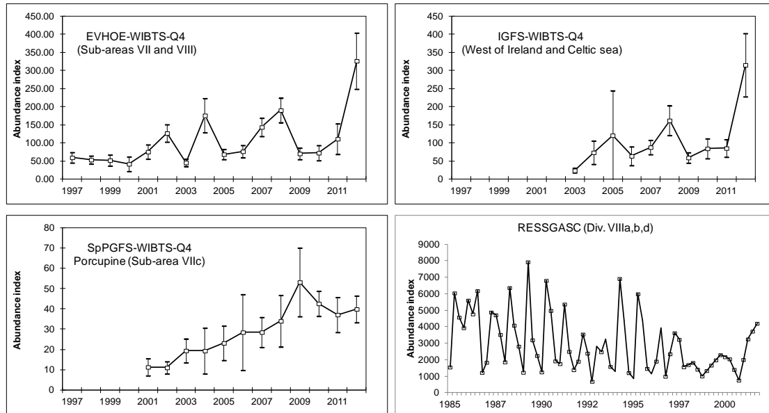
Figure 4.4.3.2.1. Hake in Division IIIa, Subareas IV, VI and VII and Divisions VIIIa,b,d (Northern stock) abundance indices from surveys.
