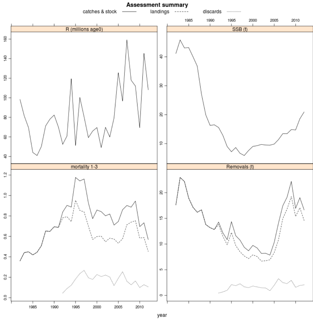
Figure 4.5.9. Summary plot. SSB and removals (catch, landings and discards) in '000 t. Recruitment in '000000 individuals.
