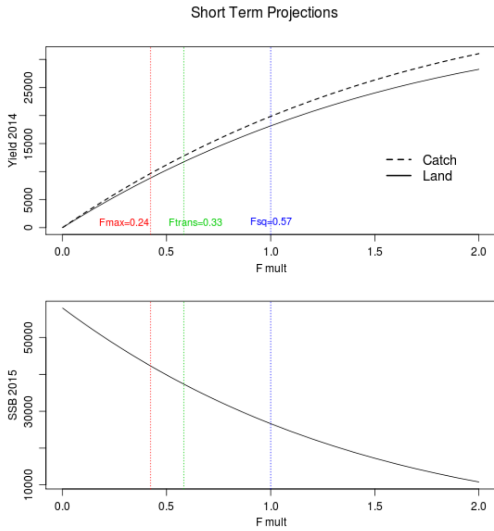
Figure 4.5. 11. Short-term advice
