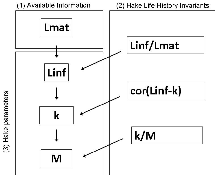
Figure 1. Hake meta-analysis
