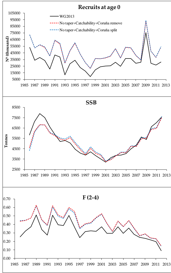
Figure 5.5.4.9. Four spot megrim ( L.boscii ) (Divisions VIIIc and IXa). Sensitivity analysis to different tuning fleet options.
