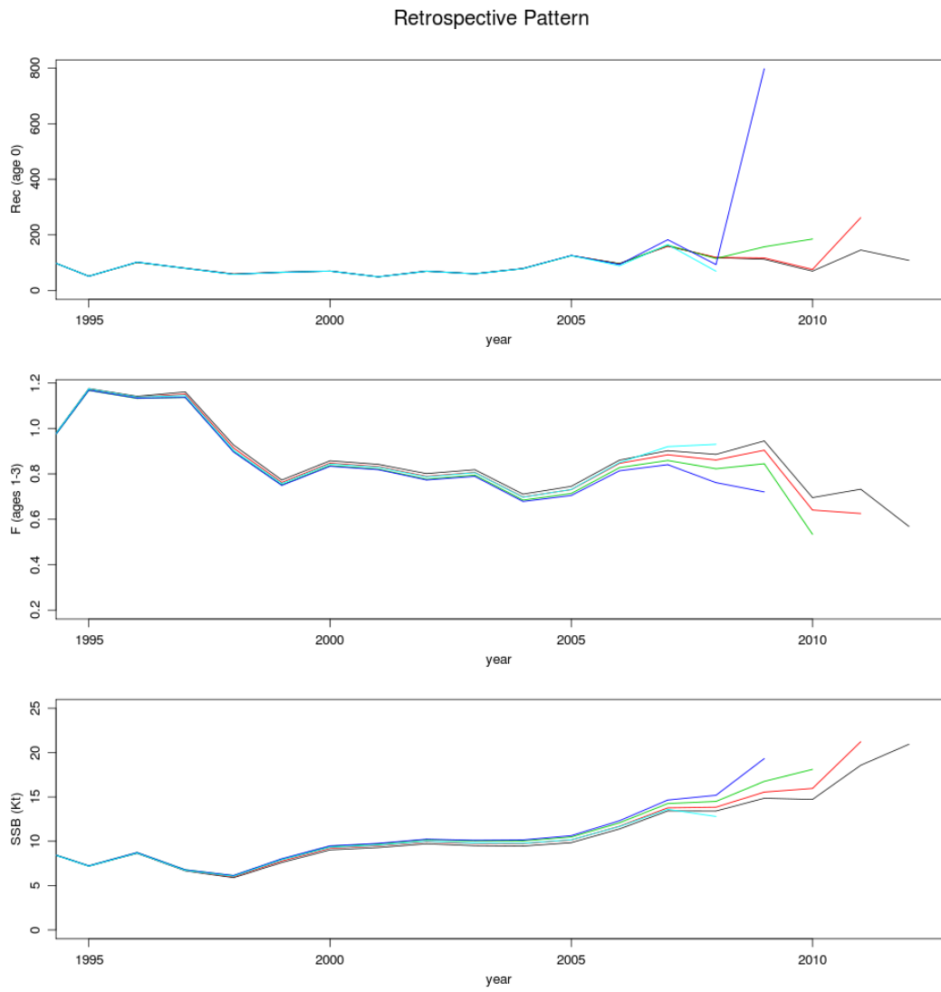
Figure 4.5.10. Retrospective plot
