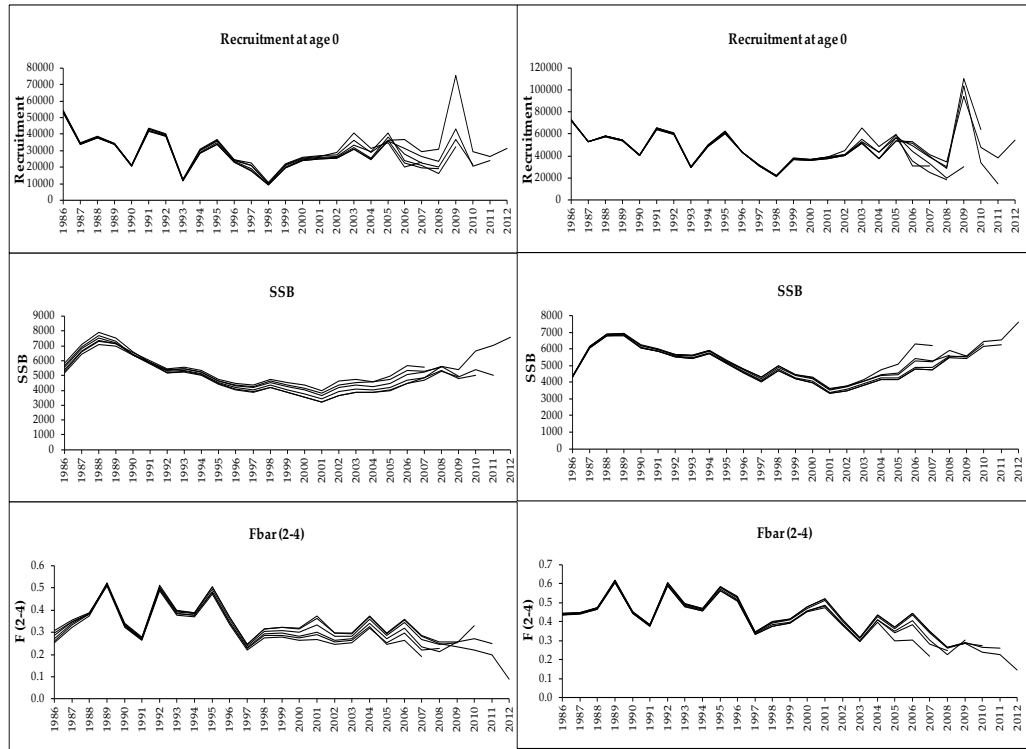
Figure 5.5.4.13. Four spot megrim ( L. boscii ) (Divisions VIIIc and IXa). Retrospective patterns of WGMM2013 assessment and final assessment configuration.
