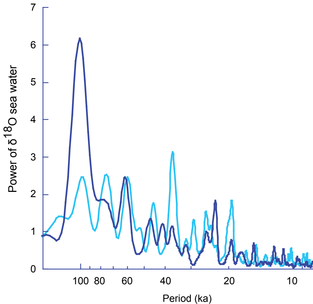
Figure S2. Blackman Tukey spectral analysis of \delta^{18}\text{O} sea water. Light blue for G. ruber sensu stricto and dark blue for G. ruber sensu lato
