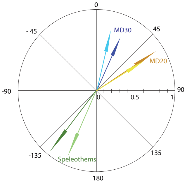
Figure S3. Coherence and phase angle (°) with daily insolation in June at the Equator of \delta^{18}\text{O} of speleothems from China (green), MD05-2930 SST from T. G. ruber sensu stricto (blue) and of MD05-2920 SST (yellow). Dark shades correspond to the 23ka band and light shades to the 19ka band.
