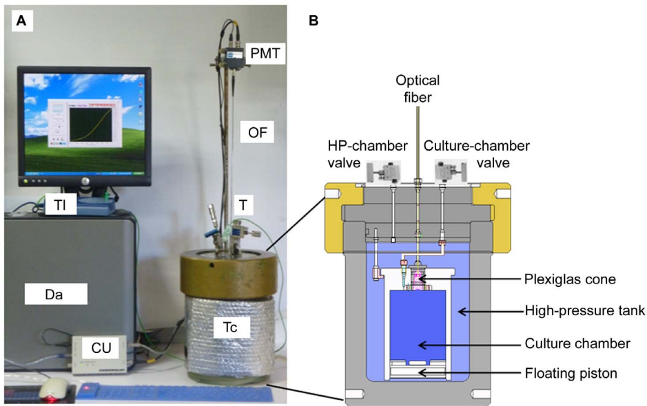
Figure 1. High-pressure bioluminescence system. (A) Photograph of the high-pressure bioluminescence system and (B) schematic section diagram of the high-pressure bioluminescence tank. PMT: photomultiplier tube; OF: optical fiber; CU: photomultiplier counting unit; T: high-pressure temperature sensor; Tc: Tubing around tank for temperature control connected to a thermo chiller (not shown); TI: Data logger for temperature sensor; Da: PC for data acquisition of bioluminescence and temperature; doi:10.1371/journal.pone.0066580.g001
