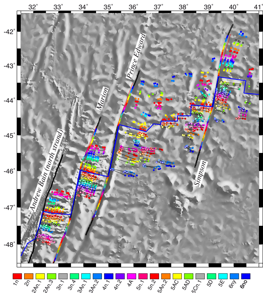
Figure 14. Best-fitting reconstructions of Lwandle–Antarctic magnetic lineations. Solid circles show unrotated magnetic reversal crossings identified from shipboard and airborne data (also shown in Fig. 2). Open circles show Lwandle plate reversal crossings rotated onto the Antarctic plate. Black lines show great circle segments that best fit the reconstructed reversal crossings, which define paleospreading segments. The blue line shows the present plate boundary. See Fig. 2(A) for the map location.
