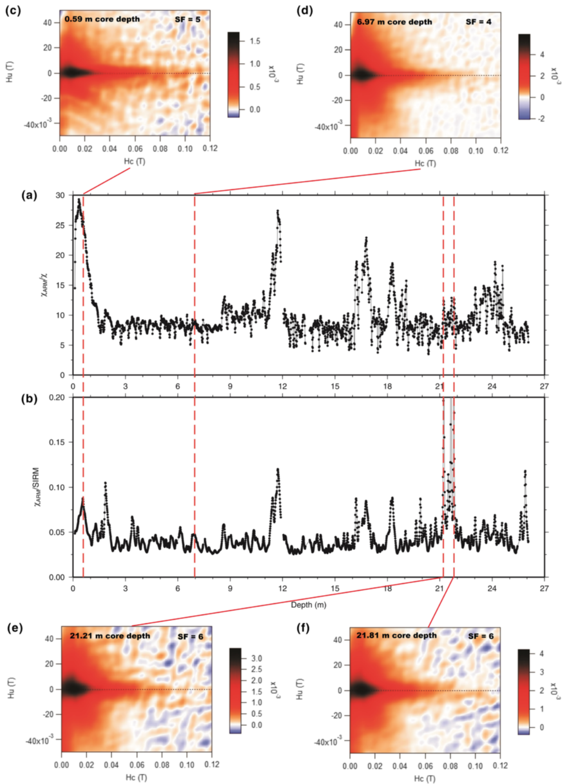
Fig. 3 a, b Variations of the two ratios, \chi_{ARM}/\chi and \chi_{ARM}/SIRM (in depth). c–f The FORC diagrams of the studied samples which obtained at 0.59, 6.97, 21.21, and 21.81 m core depth. The red lines mark the locations where the four samples were selected and the smoothing factors (SF) are given in the diagrams, respectively
