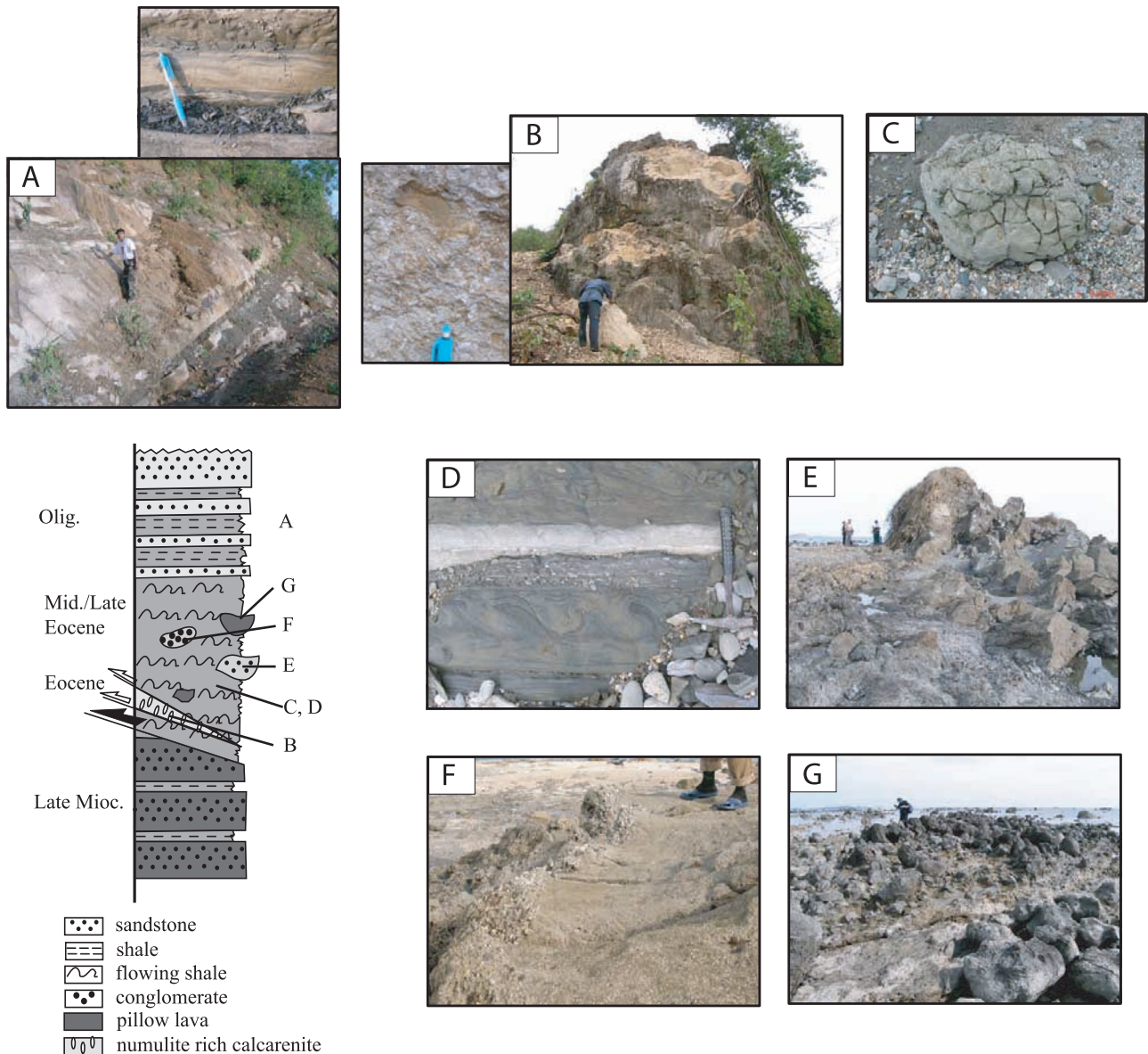
Figure 8. Approximate stratigraphic column of Ramree area and pictures illustrating these various stratigraphic units (see text for a detailed description of the units).
