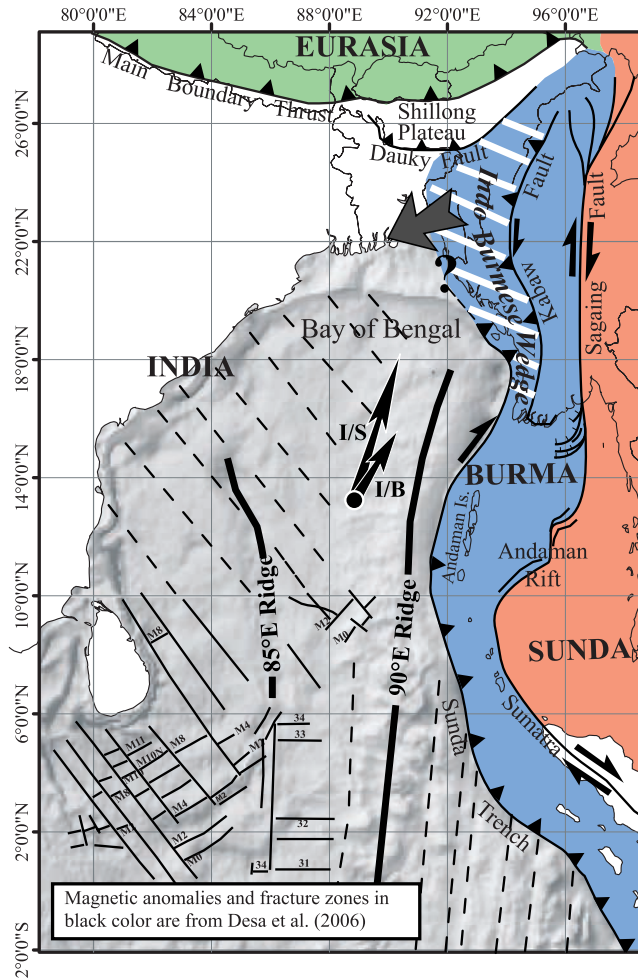
Figure 1. Structural fabric of the Bay of Bengal with its present kinematic setting. Shaded background is the gravity map from Sandwell and Smith [1997]. Fractures and magnetic anomalies in black color are from Desa et al. [2006]. Dashed black lines are inferred oceanic fracture zones which directions are deduced from Desa et al. in the Bay of Bengal and from the gravity map east of the 90°E Ridge. We have flagged particularly the 90°E and the 85°E ridges (thick black lines). Gray arrow shows the Indo-Burmese Wedge (indicated as a white and blue hatched area) growth direction discussed in this paper. For kinematics, black arrows show the motion of the India Plate with respect to the Burma Plate and to the Sunda Plate (I/B and I/S, respectively). The Eurasia, Burma, and Sunda plates are represented in green, blue, and red, respectively.
