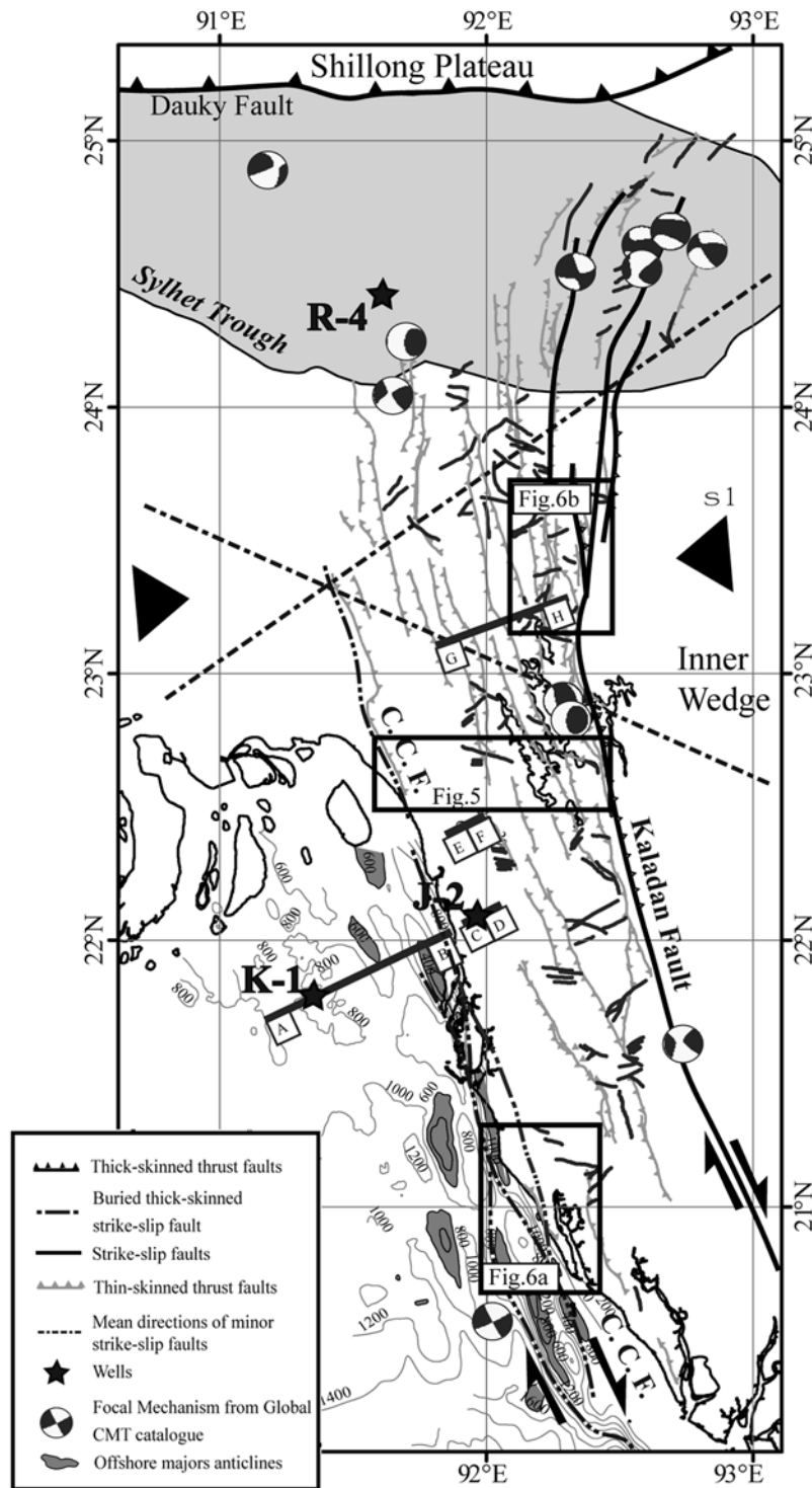
Figure 3. Structural map of the northern outer wedge. Dashed lines are the two mean directions of conjugated minor faults affecting the outer wedge. Dark gray faults are thin-skinned tectonic structures. The dash-dotted line is the buried incipient Chittagong Coastal Fault (CCF). Offshore contours are time contours (200 ms) of a latest Pliocene horizon interpreted on industrial multichannel seismic lines. Major anticlines are filled in gray. Focal mechanisms are from the global CMT catalog ( http://www.globalcmt.org/CMTsearch.html ). Seismic lines AB, CD, EF, and GH interpreted in Figure 4 are located as thick black lines. Black stars show the location of wells Kutubdia-1 (K-1), Rashdpur-4 (R-4), and Jaldi-2 (J-2) used for seismic interpretation.
