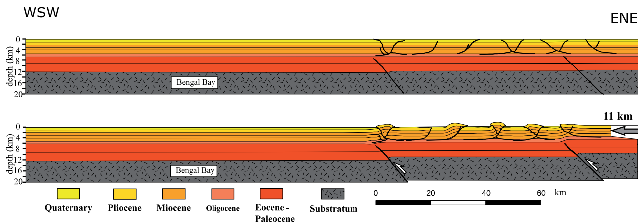
Figure 11. Forward modeling constructed with the Paradigm software GeoSec 2D. Best fit is controlled visually with the cross section presented in Figure 8a. Only fault-related deformation is modeled. See text for initial model constrains.
