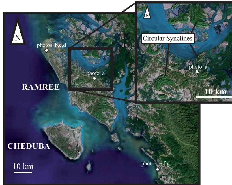
Figure 7. Landsat image of the Ramree and Cheduba islands. The area is located in the larger-scaled Figure 2. The locations of photos from Figure 8 are flagged as white stars. Insert at top right shows a close-up on the typical circular synclines.
