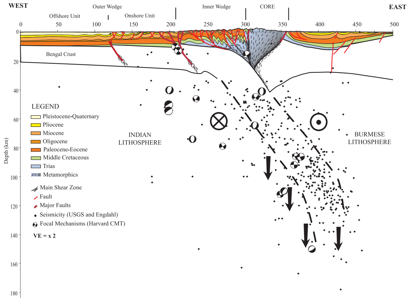
Figure 15. Present cross section based on industrial multichannel seismics and field observations. The seismicity from USGS catalog and Engdahl [2002] is represented as black dots. Focal mechanisms from Global CMT ( http://www.globalcmt.org/CMTsearch.html ) catalog are also represented.
