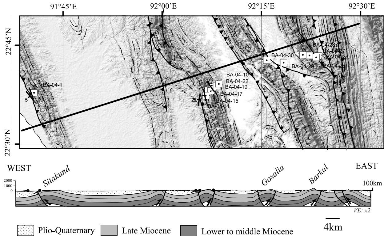
Figure 5. Synthetic field cross section through the outer Indo-Burmese Wedge. The sample list is provided in Table 1.
