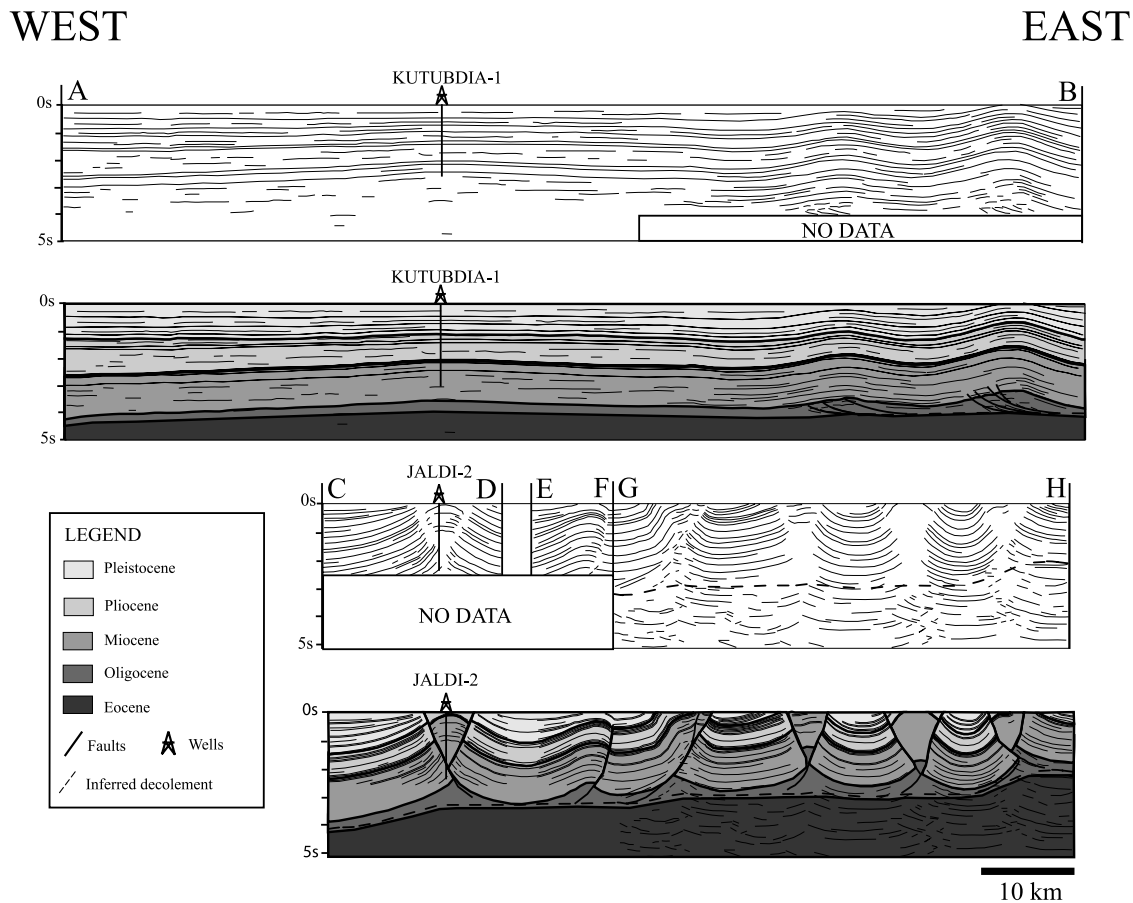
Figure 4. Line drawing and interpretation of seismic lines in the outer Indo-Burmese Wedge supported by two wells. Localization of these lines and wells are represented in Figure 3.
