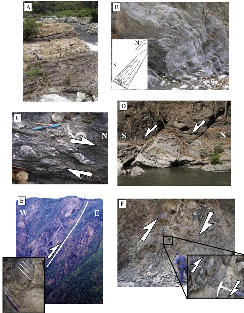
Figure 14. Pictures illustrating the structures observed on the inner most parts of the Indo-Burmese Wedge. (a) Unmetamorphosed Triassic sandstones. (b) Mica schists affected by mulion folds that indicate N-S extension. (c) Quartz exsolution that indicates top-to-the-north motion. (d) E-W striking normal faults affecting the Triassic sandstones. (e) Tight folds in the inner wedge with slickensides on S0 indicating a combined right-lateral and reverse motion. (f) Reverse right-lateral shear zone within the inner wedge.
