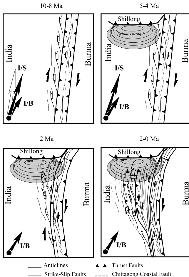
Figure 16. Cartoon showing the tectonic evolution of the Indo-Burmese Wedge from late Miocene to present.
