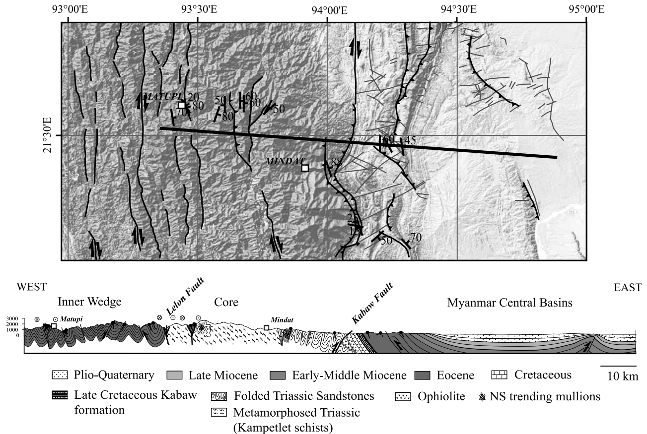
Figure 13. Synthetic field cross section through the inner Indo-Burmese Wedge (location in Figure 2).
