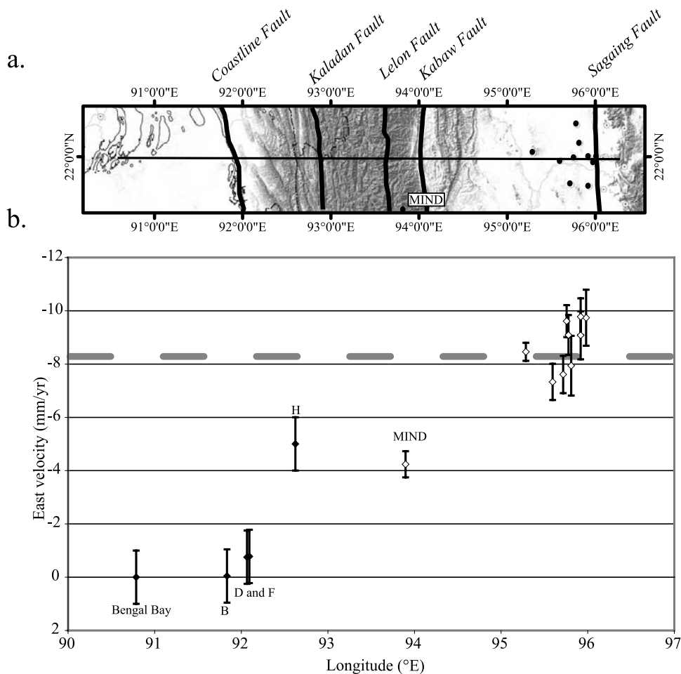
Figure 12. (a) Shaded SRTM image along the cross section at 22°N. Black lines represent the major faults. Black dots are the GPS sites within the Burma Plate. (b) Graphic representation of the E-W shortening rate with respect to India as a function of longitude, around 22°N. White diamonds are from geodetic measurements within the Burma Plate [Vigny et al. , 2003], and black diamonds are obtained from the four restored cross sections (this study) and have been projected parallel to the folds azimuth on an E-W cross section at 22°N. MIND is the Mindat GPS station. B, D, F, and H are the end points of cross sections CS-AB, CS-CD, CS-EF, and CS-GH, respectively. The thick dashed line shows the India/Burma E-W shortening rate (8.3 mm/a) calculated from Socquet et al. [2006] and Nielsen et al. [2004].
