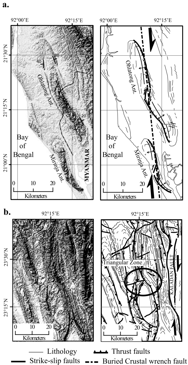
Figure 6. (a) Structural map of Olhatong and Mirinja anticlines (Ant.), based on SRTM image's interpretation. These two anticlines are interpreted as two right laterally wrenched folds along the Chittagong coast. (b) Structural map in the vicinity of the Kaladan Fault, based on SRTM image's interpretation, showing typical triangular zones.
