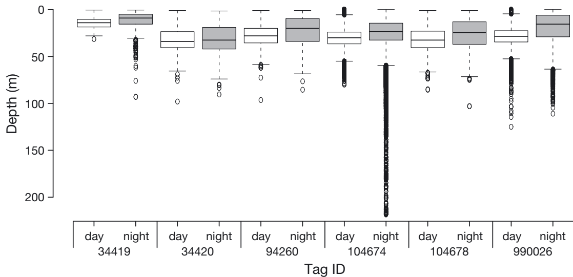
Fig. 7. Depth distributions during day and night obtained from PSAT and archival tags deployed on silky sharks Carcharhinus falciformis at drifting FADs in the western Indian Ocean. Lines within the boxes represent median values. Upper and lower ends of the boxes represent the 1st and 3rd quartiles, respectively; upper and lower whiskers indicate minimum and maximum values, respectively. (o) Outliers; white and grey shading: day and night distributions, respectively
