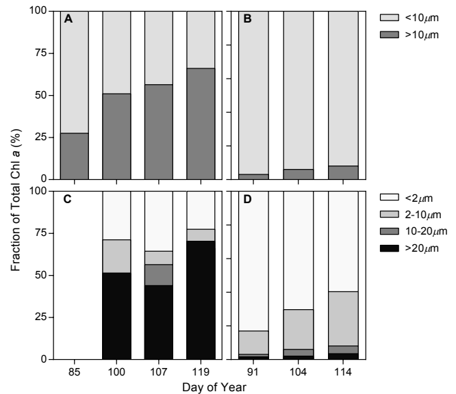
Figure 5. Size-fractionated Chl a for (a, c) the Iceland Basin, and (b, d) the Norwegian Basin. Plots (a) and (b) show the < 10 and > 10 μm fractions, (c) and (d) show the < 2, 2–10, 10–20 and > 20 μm fractions.
