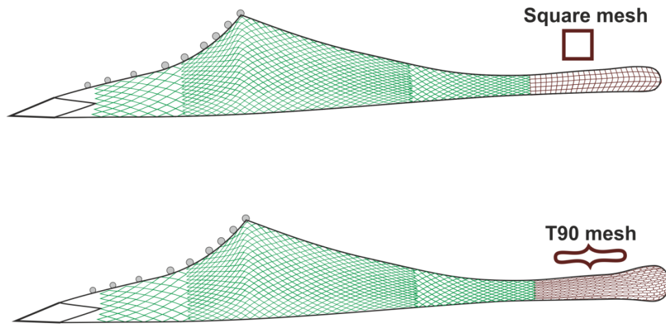
Figure 30. Investigation of square or T90 mesh in bottom trawl codends of Black Sea: different types of mesh in the bottom trawl codend
