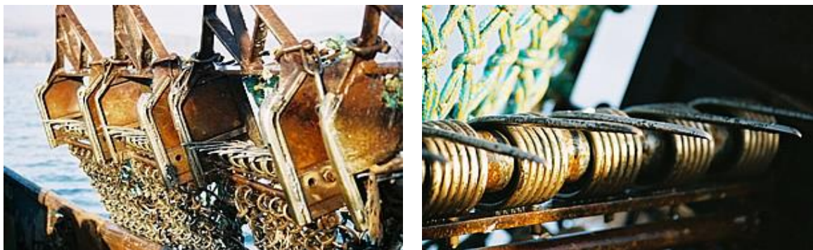
Figure 17. Enviro dredge showing detail of individually sprung teeth (tines).
