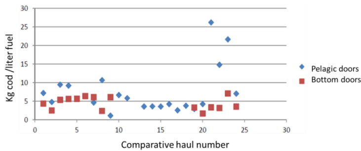
Figure 4. Cod catch weight (kg) per liter fuel consumption for the same trawl and sweep lengths fished with pelagic doors (blue diamonds) and bottom doors (red squares) from the same vessel, but on different trips (Gemba, 2011).
