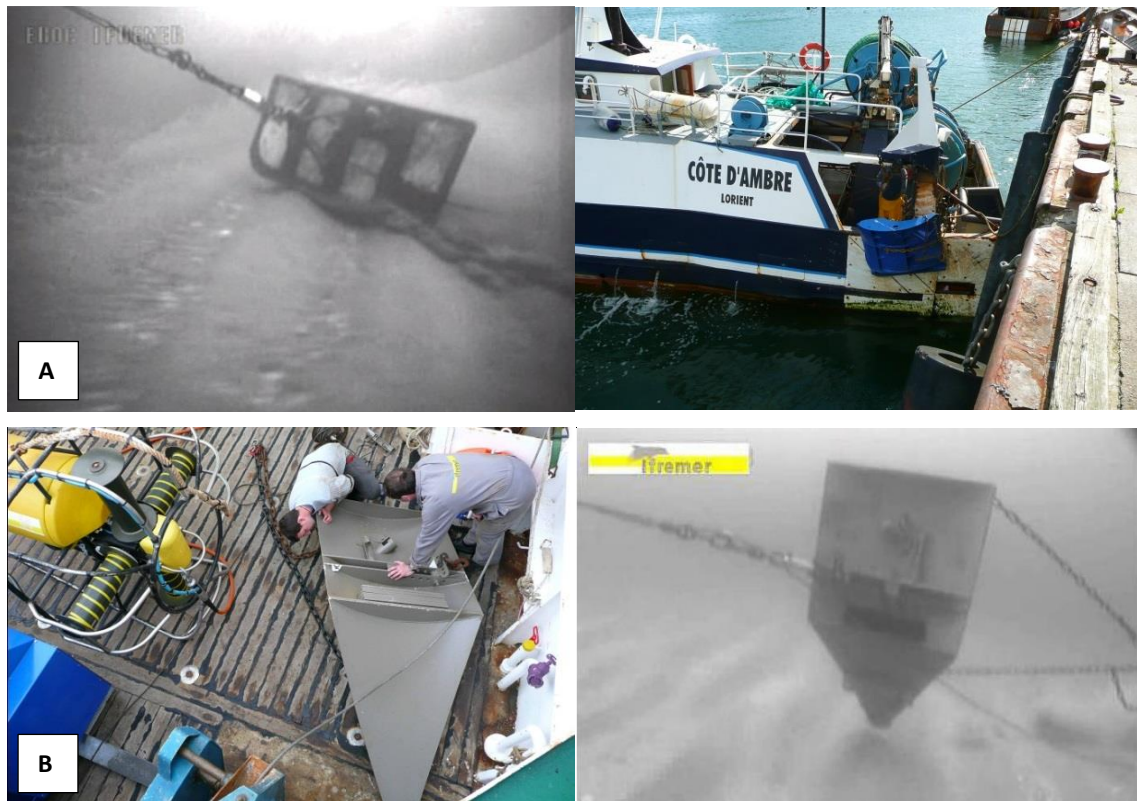
Figure 13. Illustrations of A) traditionally utilized otter board for twin trawls, submarine view of plan-shaped board (left picture) and more recent otter board onboard partner fishing vessel (picture on the right) and B) prototype of the jumper board tested during Optipeche project (Vincent et al. 2010) and that will be tested in the Nephrops fishery during Benthis project.
