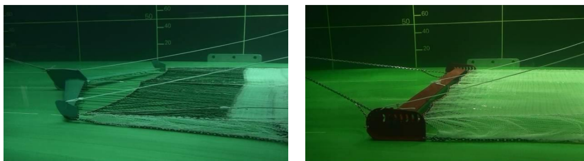
Figure 11. (A) Model of a “Jack Wing” in the flume tank of IFREMER in Boulogne-sur-Mer; (B) Model of a “Delmeco Wing” in the flume tank of IFREMER in Boulogne-sur-Mer.
