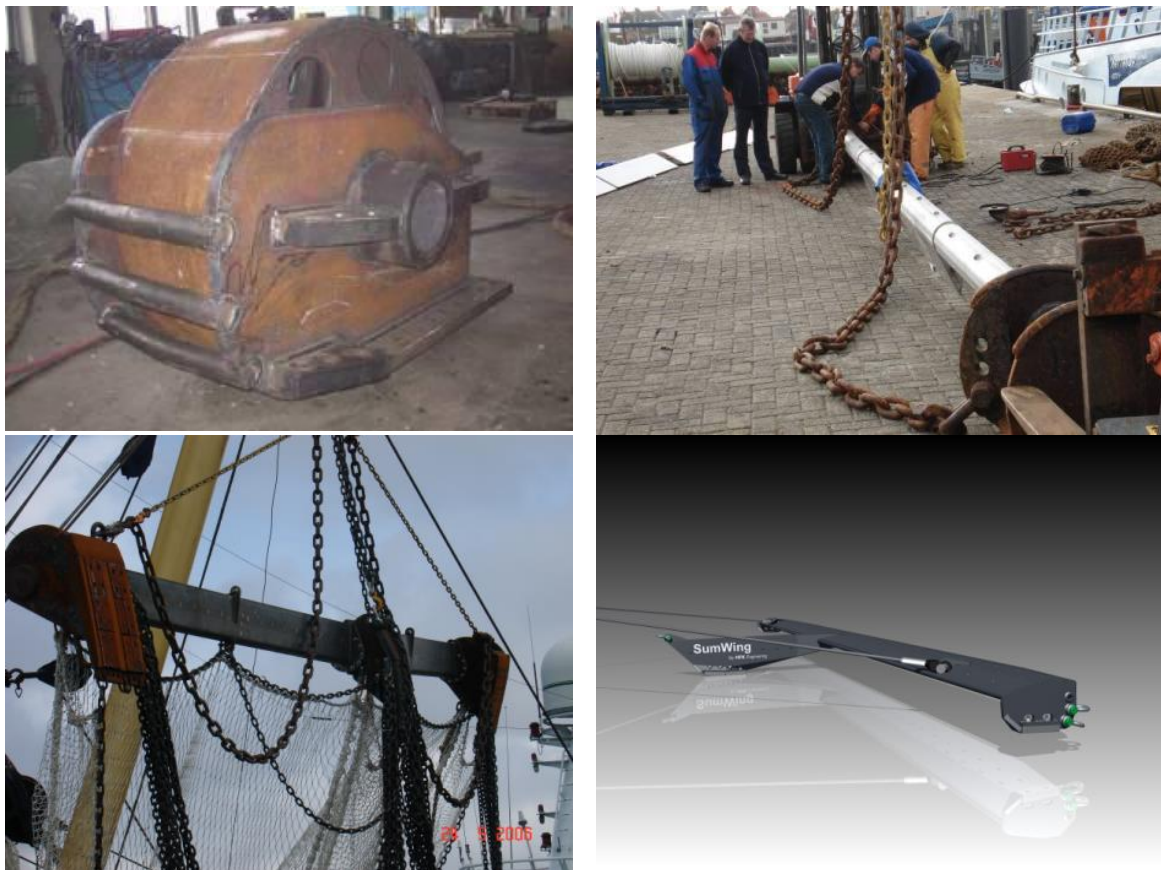
Figure 10. (A) Wheel to replace beam trawl shoe; (B) Spoiler; (C) Fly-beam and (D) SumWing with front runner.
