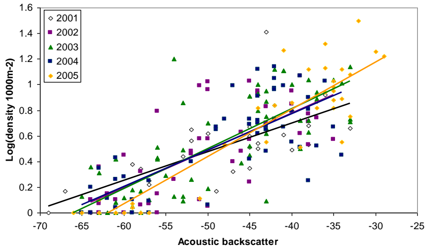
Figure 16. Relationships between multibeam acoustic backscatter and catch rates of scallop in annual surveys, 2001-2005, in the Celtic Sea. Higher catches occur on harder ground (gravels).
