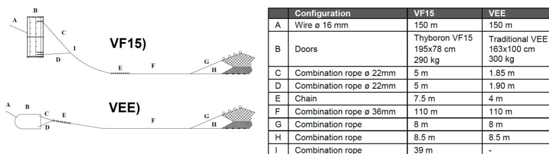
Figure 21. Main details of the gear rigging adopted during the sea trials. Configurations with the Thyboron type VF15 (VF15) and with the traditional VEE door (VEE).
