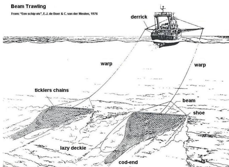
Figure 9. Beam trawling (From: E.J. de Boer en C. Vermeulen, 1976)
