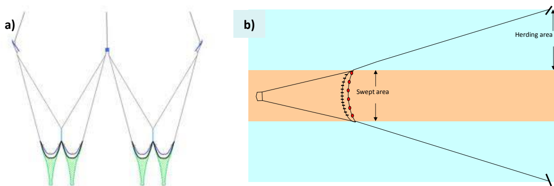
Figure 5. A) Four trawl (codend) system and B) scheme of bridles or sweeps shortening in Nephrops Fishery in Kattegat.
