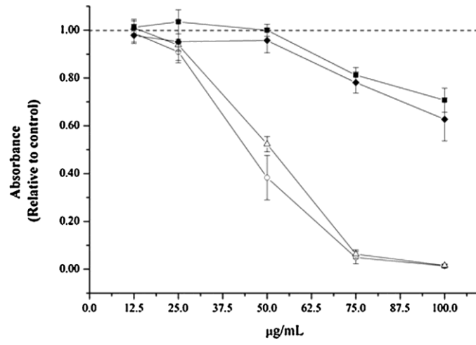
Fig. 4. HT-29 cell viability upon treatment for 24 h with different concentrations of N1 (circle), N2 (triangle), P1 (square) and P2 (diamond) extracts. Error bars are given as 95% confidence interval.
