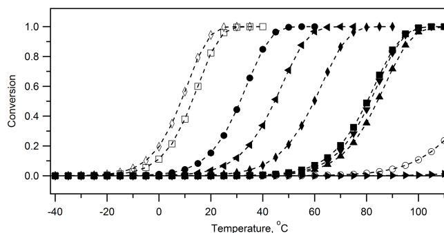
Figure 8. Thermal decomposition profiles of IONO 2 , \blacklozenge ; BrONO 2 , \circ ; ClONO 2 , \blacktriangleright ; HO 2 NO 2 , \bullet ; N 2 O 5 , \blacktriangleleft ; C 2 H 5 O 2 NO 2 , \diamond ; CH 3 C(O)CH 2 O 2 NO 2 , \square ; MPAN, \blacksquare ; PAN, \blacktriangle ; and PPN, \blacktriangledown . Calculated from IUPAC recommended kinetic data (Atkinson et al., 2004, 2006, 2007) using FACSIMILE kinetic modelling software (MCPA Software Ltd.) based on 1 s residence time. Note that CH 3 O 2 NO 2 is not shown but has the same profile as CH 3 C(O)CH 2 O 2 NO 2 .
