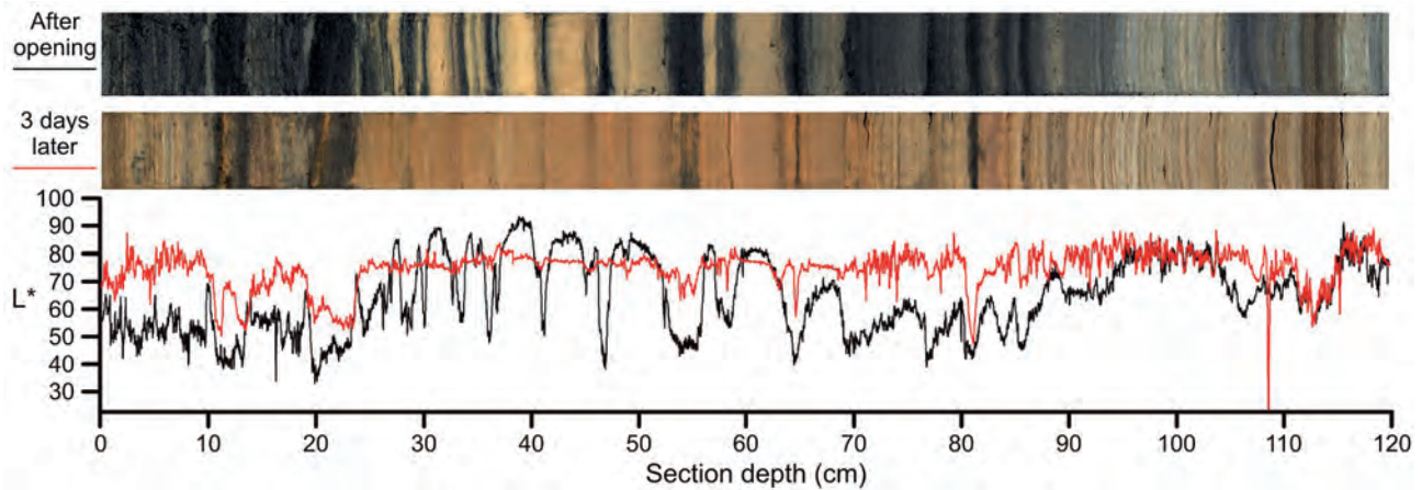
Figure 5. Digital images and colour data information of a varved sediment core from Montcortés Lake, Lérida (Spain), obtained with the colour line-scan camera of the AVAATECH XRF core scanner at two different moments: immediately after opening, and 3 days later (Corella et al. , 2014). Oxidation of the organic matter by contact with the air produced a significant change in the appearance of sediments. c) Colour data, here expressed as reflectivity ( L^* ), allows a quantitative identification of colour changes in the sediment at 70 \mu\text{m} resolution. Differences in reflectivity of both records denote the great impact that oxidation has on the sediment.
