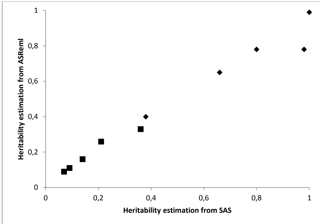
Figure S1: Correlations between SAS and ASReml heritability estimates for survival in C. gigas when exposed to OshV-1 or V. aestuarianus under controlled laboratory conditions in Spat1, Spat2, Juvenile1, Juvenile2 and Adult. Black squares represents V. aestuarianus challenge and black diamonds represents OshV1 challenge.
