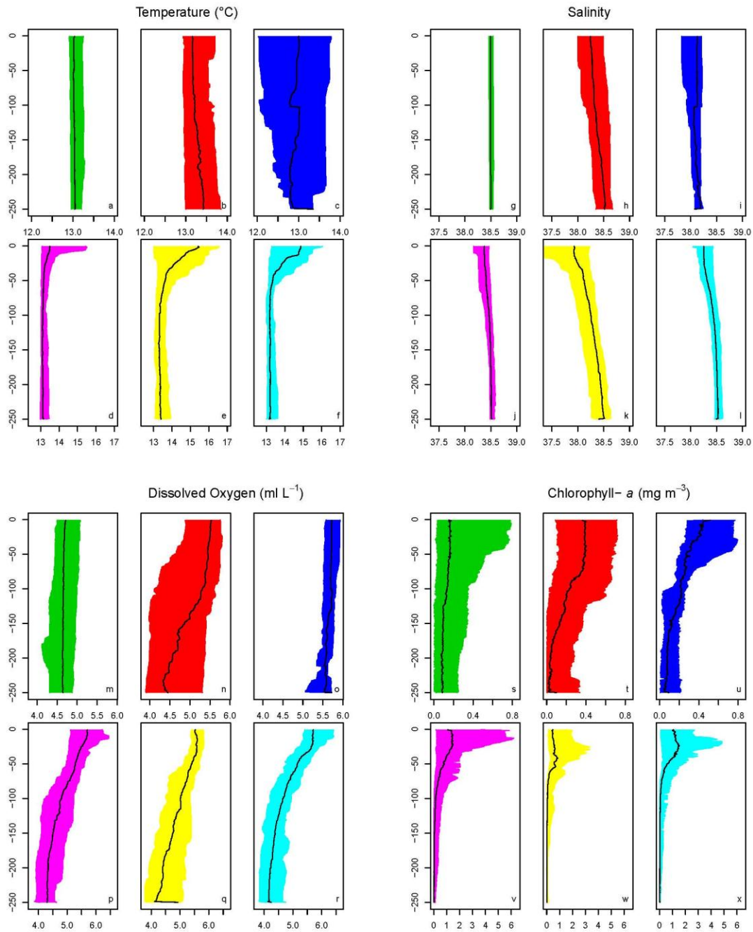
Figure S1. Average vertical profile, for temperature, salinity, dissolved oxygen and chlorophyll-a, black line corresponds to the median value for each cluster, colors correspond to quantiles (0.025 to 0.975 range) and clusters of Figure 2.
