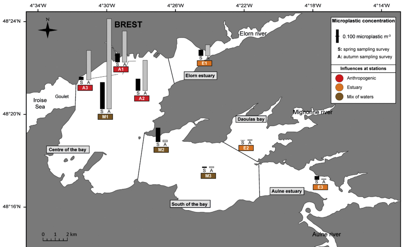
Fig. 2. Microplastic concentration (particles \text{m}^{-3} ) in surface water samples (9 locations; the 5 areas are separated by black lines) in spring and autumn 2014 in the Bay of Brest. Bars on the chart are proportional to microplastic concentration.
