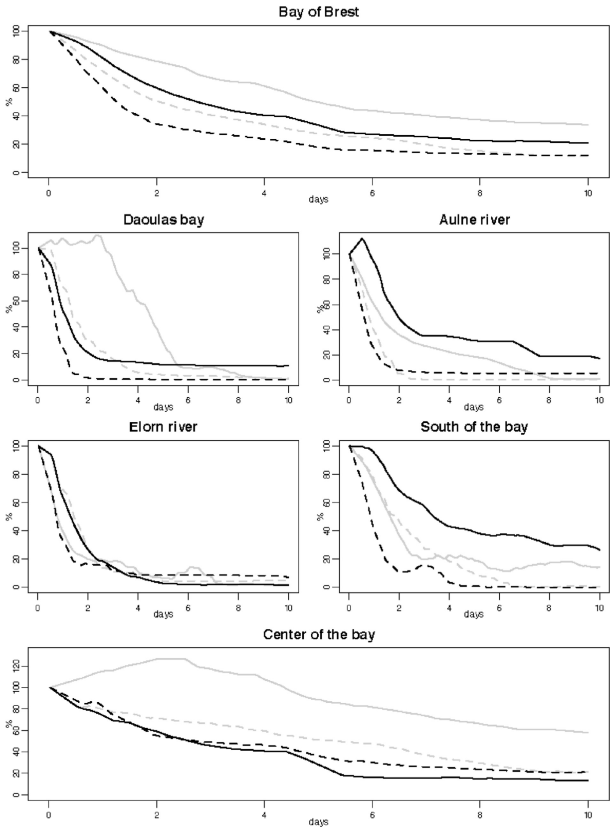
Fig. 4. Particle distribution in the Bay of Brest and in each of the 5 tracking zones for 10 days after the release of the particles (25 particles per 50 \times 50 m) based on hydrodynamic characteristics for releases at neap tide (solid black line) and spring tide (dashed black line) periods during a flood period, and for releases at neap tide (solid grey line) and spring tide (dashed grey line) during a low water period (2013).
