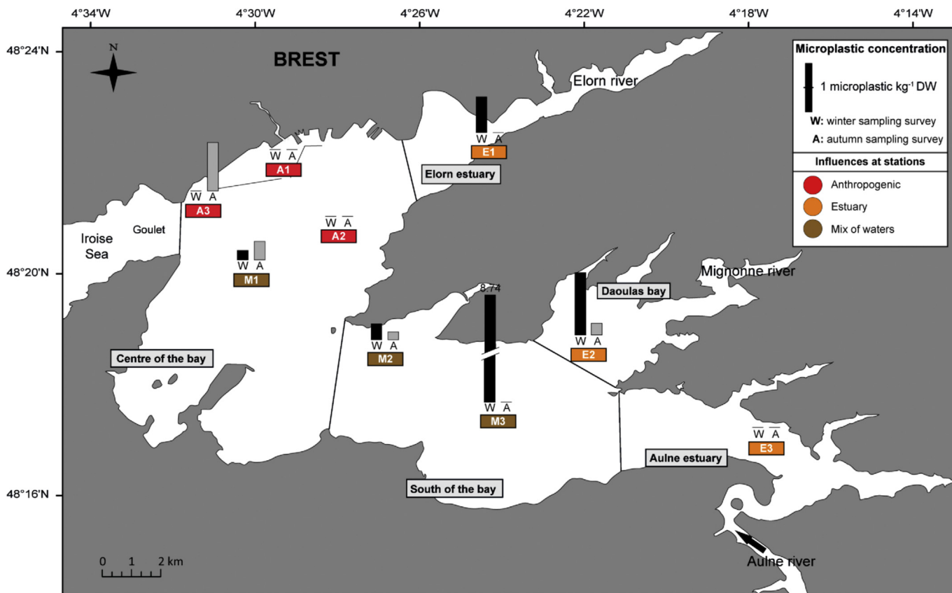
Fig. 3. Microplastic concentration (particles \text{kg}^{-1} \text{ DW} of sediment) in sediment samples (9 locations; the 5 areas are separated by black lines) in winter and autumn 2014 in the Bay of Brest. Bars on the chart are proportional to microplastic concentration.
