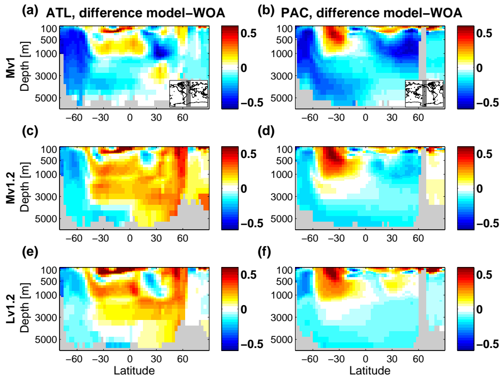
Figure 2. As Fig. 1 but for salinity.
