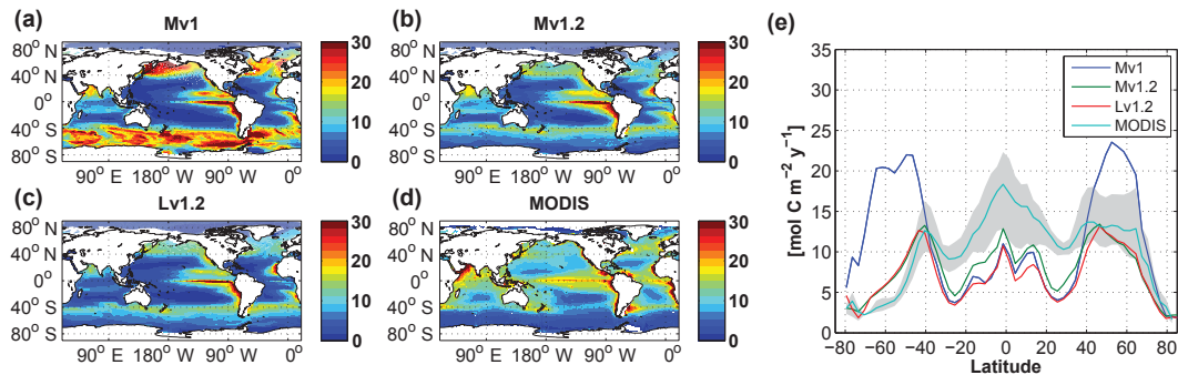
Figure 6. Vertically integrated primary production ( \text{mol C m}^{-2} \text{yr}^{-1} ) averaged over the years 2003–2012 for model configurations (a) Mv1, (b) Mv1.2, and (c) Lv1.2, and (d) the mean of three satellite-based climatologies (derived from MODIS retrievals; see text). Panel (e) displays the zonal means of each field presented in panels (a–d). The grey shaded area represents the range of the zonal means of the three satellite-based climatologies.
