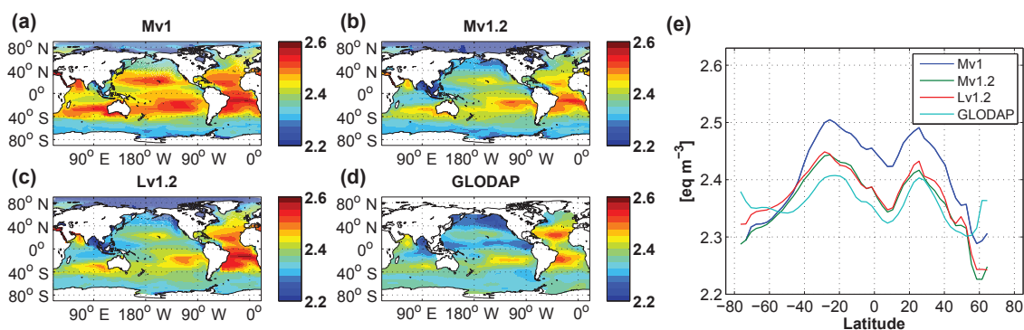
Figure 18. As Fig. 17 but for surface total alkalinity ( \text{eq m}^{-3} ).
