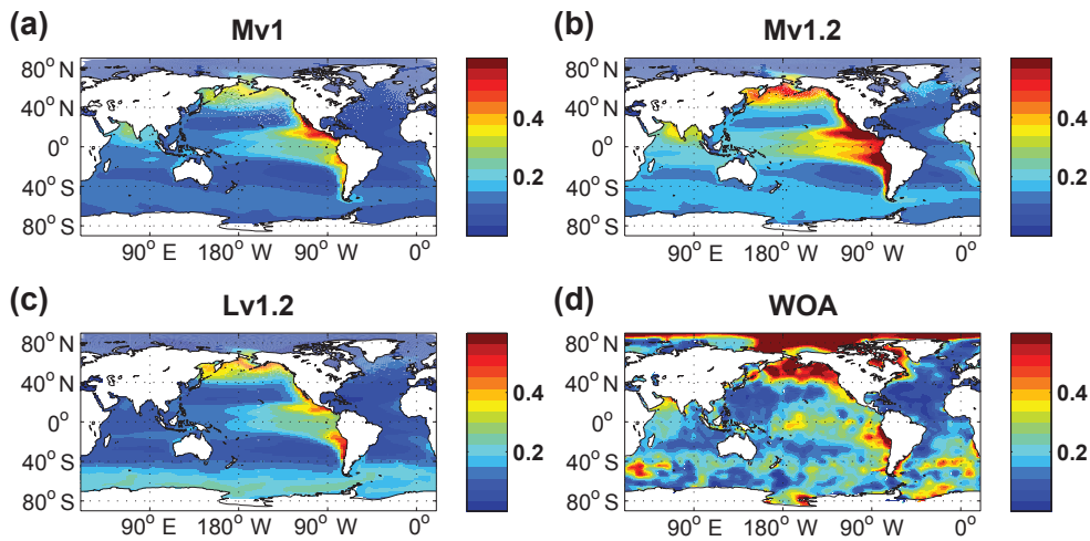
Figure 13. Difference [\text{PO}_4] - [\text{NO}_3]/16 ( \text{mmol m}^{-3} ) at the surface averaged over the years 1965 to 2007 for model configurations (a) Mv1, (b) Mv1.2, (c) Lv1.2, and (d) surface [\text{PO}_4] - [\text{NO}_3]/16 as calculated from the World Ocean Atlas gridded data set.
