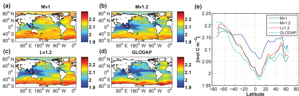
Figure 17. Surface concentration of dissolved inorganic carbon ( \text{mol m}^{-3} ) averaged over the years 1988 to 1998 for the model configurations (a) Mv1, (b) Mv1.2, and (c) Lv1.2, and (d) corresponding surface DIC from the observation-based GLODAP climatology. Panel (e) displays the zonal mean of each field presented in panels (a–d).
