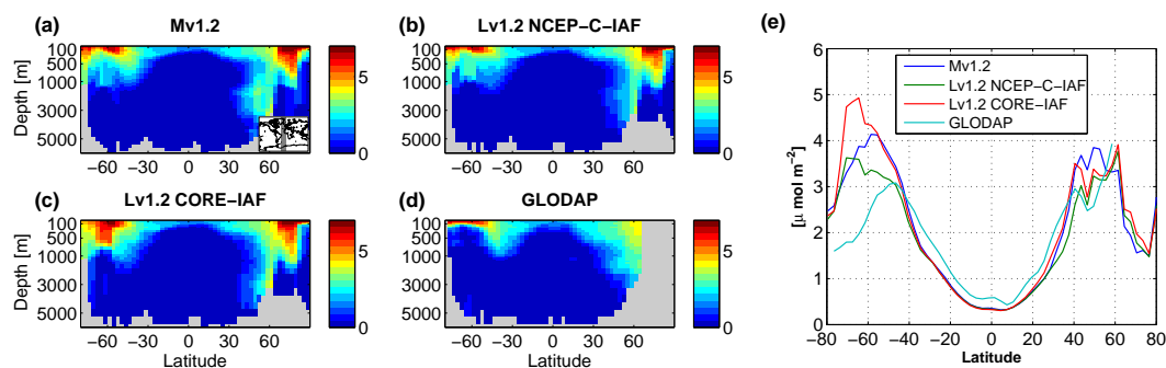
Figure 5. Zonal mean CFC-11 concentrations ( \text{nmol m}^{-3} ) along a section through the Atlantic/Southern Ocean (as indicated by the grey shaded area in panel a) averaged over the years 1988 to 1998 for the model configurations (a) Mv1.2, (b) Lv1.2 forced with NCEP-C-IAF, (c) Lv1.2 forced with CORE-IAF, and (d) CFC-11 concentration taken from the GLODAP gridded data set. Panel (e) displays the global zonal mean CFC-11 column content ( \mu\text{mol m}^{-2} ).
