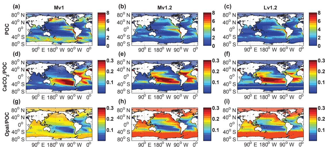
Figure 9. Export production of POC averaged over the years 2003–2012 for the model configurations (a) Mv1, (b) Mv1.2, and (c) Lv1.2; corresponding \text{CaCO}_3 to organic carbon ratio in exported matter for (d) Mv1, (e) Mv1.2, and (f) Lv1.2; corresponding opal to organic carbon ratio in exported matter for (g) Mv1, (h) Mv1.2, and (i) Lv1.2.
