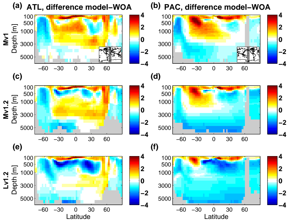
Figure 1. Temperature difference model–WOA averaged over 1965–2007 along zonal mean sections through the Atlantic/Southern Ocean (a, c, e) and the Pacific/Southern Ocean (b, d, f) for model configurations Mv1 (a, b), Mv1.2 (c, d), and Lv1.2 (e, f). The regions covered by the zonal mean calculations are indicated by the grey shaded area in the insets of panels (a) and (b).
