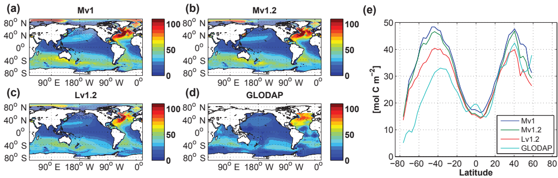
Figure 22. Vertically integrated anthropogenic carbon ( \text{mol m}^{-2} ) for the year 1994 for model configurations (a) Mv1, (b) Mv1.2, and (c) Lv1.2, and (d) corresponding \text{DIC}_{\text{ant}} from the observation-based GLODAP climatology (Sabine et al., 2004). Panel (e) displays the zonal mean of each field presented in panels (a–d).
