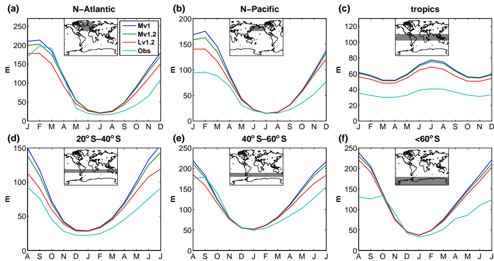
Figure 4. Mean seasonal cycle of mixed layer depth over the years 1961–2008 for the (a) North Atlantic, (b) North Pacific, (c) tropics (20° S to 20° N), (d) southern subtropics (20 to 40° S), (e) latitudes between 40 and 60° S, and the (f) Southern Ocean south of 60° S. Shown are results for model configurations Mv1 (dark blue), Mv1.2 (green), and Lv1.2 (red). The light blue line is the observation-based climatology of de Boyer Montégut et al. (2004), which uses a density threshold criterion of 0.03 \text{ kg m}^{-3} to define MLD.
