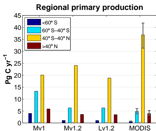
Figure 7. Mean values of total primary production over the years 2003–2012 simulated by the three model configurations and an estimate of PP based on satellite data (mean of three climatologies derived from MODIS retrievals; see text) for the regions indicated in the inset. The grey bars indicate the range of observation-based estimates.
