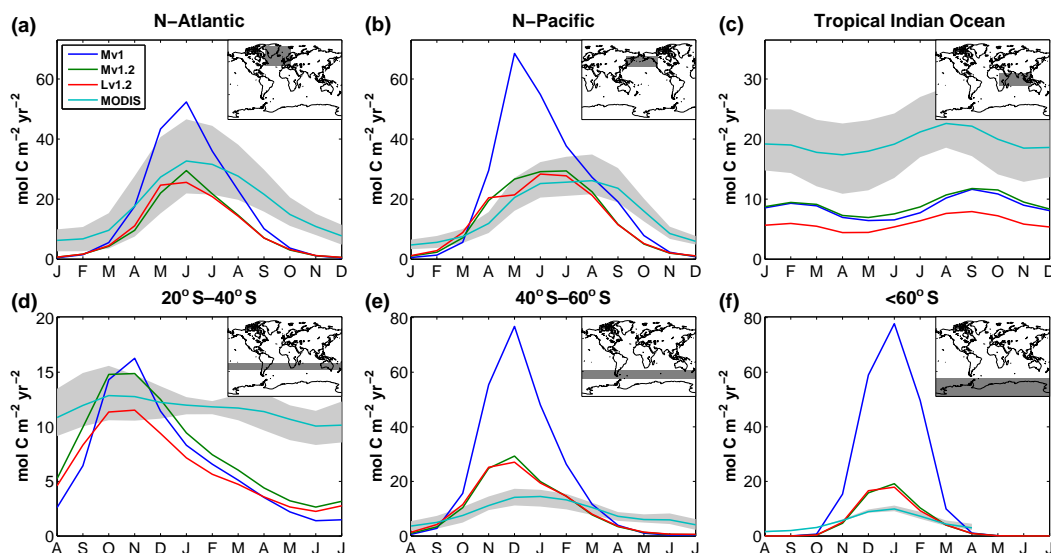
Figure 8. Mean seasonal cycle of vertically integrated primary production over the years 2003–2012 for the (a) North Atlantic, (b) North Pacific, (c) tropical Indian Ocean (Indian Ocean between 20° S and 20° N), (d) southern subtropics (40 to 20° S), (e) latitudes between 60 and 40° S, and the (f) Southern Ocean south of 60° S. Shown are the results for model configurations Mv1 (dark blue), Mv1.2 (green), and Lv1.2 (red) and the mean and range of the satellite-derived seasonal cycle (light blue and grey shaded areas).
