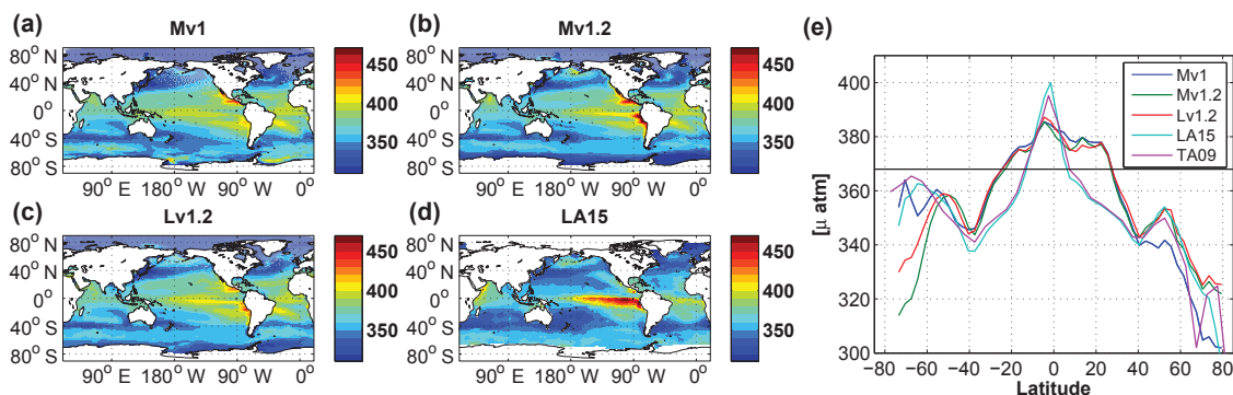
Figure 19. Surface partial pressure of \text{CO}_2 ( \mu\text{atm} ) averaged over the years 1995 to 2005 for model configurations (a) Mv1, (b) Mv1.2, (c) Lv1.2, and (d) the observation-based surface p\text{CO}_2 data set of Landschützer et al. (2015a). Panel (e) displays the zonal mean of each field presented in panels (a–d) and additionally the zonal mean of the data product by Takahashi et al. (2009). The black line indicates the mean atmospheric p\text{CO}_2 over the averaging period.
