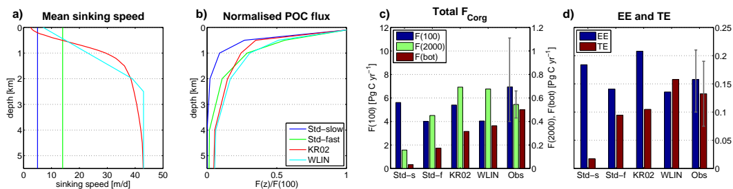
Figure 23. (a) Mean profiles of sinking speed with depth for the four experiments STD-slow (dark blue), STD-fast (green), KR02 (red), and WLIN (light blue); (b) as panel (a), but for mean profiles of POC fluxes (averaged over areas with water depth > 4000 m) normalised to the flux at 100 m depth; (c) globally accumulated fluxes of particulate organic carbon (POC) at 100 m depth (dark blue), at 2000 m depth (green), and the downward POC flux at the ocean bottom for depths larger than 1000 m (brown); (d) export efficiency (EE, dark blue) and transfer efficiency (TE, brown). The observation-based estimates (“Obs”) in panels (c) and (d) are derived from Henson et al. (2012), Honjo et al. (2008), and Laws et al. (2000) for POC flux at 100 m and EE, from Henson et al. (2012) and Honjo et al. (2008) for POC flux at 2000 m and TE, and from Seiter et al. (2005) for the bottom POC flux. The coloured bars indicate the mean of the observation-based estimates, while the grey error bars give the maximum and minimum estimates. Note that the Honjo et al. (2008) EE and TE are calculated as ratios of total PP, total export, and total flux at 2000 m, and not as the mean of gridded EE and TE values as the rest of the values presented here. We include these data nevertheless since the differences between the two methods of calculation are small compared to the spread of the observation-based data.
