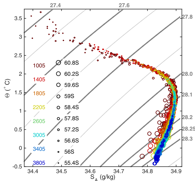
Figure 5. Conservative temperature \Theta plotted against absolute salinity S_A from the 21 occupations of SR1b, at a range of pressure levels deeper than 1000 dbar (colors, as marked on plot) and latitudes (circle sizes, as marked on plot), for the 21 occupations, with neutral density \gamma_n contours at 2000 dbar (dark gray, as marked, with pale gray at intervening 0.1 \text{ kg m}^{-3} intervals).
