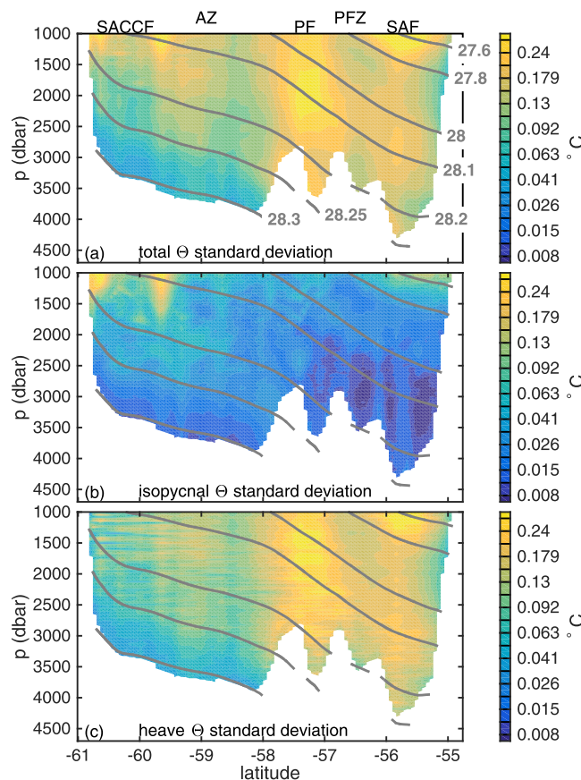
Figure 3. Standard deviations of time series of (a) \Theta and its (b) isopycnal and (c) heave components, with mean \sigma_n contours in dark gray as marked in Figure 3a. The color scale is nonlinear.
