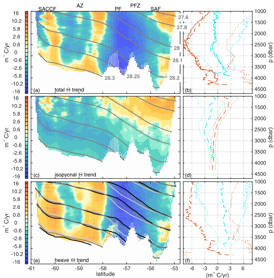
Figure 4. Trends in (a) conservative temperature \Theta and in its (c) isopycnal and (e) heave components, with mean \gamma_n contoured in dark gray (at levels marked in Figure 4a). The color scale is nonlinear. In Figure 4e, the \gamma_n trend over 20 years is indicated by movement from light gray to black contours. Trends in average temperature or component at each depth south (cyan) and north (orange) of 58^\circ\text{S} are plotted in Figures 4b, 4d, and 4f, with dotted lines indicating 95% confidence intervals (in Figures 4b and 4f the lower bounds of the confidence intervals for the northern region fall outside the horizontal axis limits of the plot). In Figure 4b, the dashed lines are the sum of the components shown in Figures 4d and 4f, while the solid lines are the original total temperature trend. Trends in Figures 4a, 4c, and 4e are shown for all grid points where equation (3) produces values in at least 50% of occupations, with the white shading (as in Figure 1b) marking points where it is not defined in the initial and/or final occupations; these areas are not included in spatial averages (e.g., Figures 4b, 4d, and 4f).
