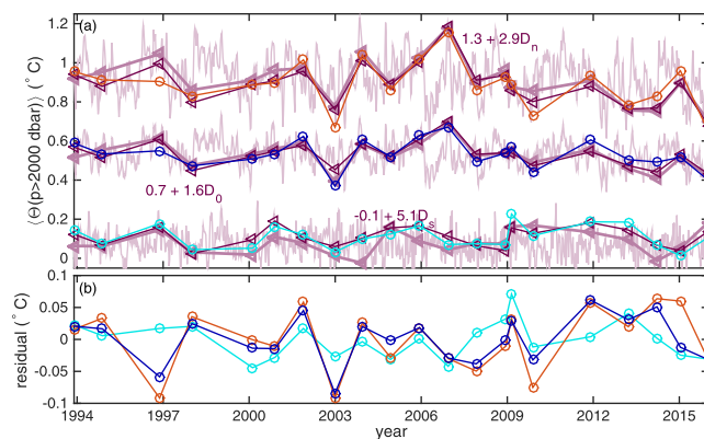
Figure 7. (a) Time series of \Theta deeper than 2000 dbar (dark blue: section-averaged \langle\Theta\rangle , cyan: \langle\Theta\rangle_S , orange: \langle\Theta\rangle_N ), with frontal position proxies D_0 , D_S , and D_N (dark purple, triangles) scaled and offset to best fit \langle\Theta\rangle , \langle\Theta\rangle_S , and \langle\Theta\rangle_N , respectively (with coefficients indicated by on-panel text). Time series of altimeter frontal position proxy D^{sh} , with the same scale factors and offsets applied, are shown in pale purple, with values interpolated to SR1b section times marked by triangles connected by thick light purple lines. (b) Residuals: \Theta - (0.7 + 1.6D_0) (dark blue), \Theta_S - (-0.1 + 5.1D_S) (cyan), and \Theta_N - (1.3 + 2.9D_N) (orange).
