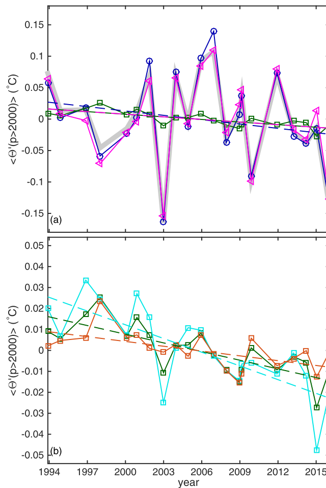
Figure 2. (a) Time series of the deviation (relative to the time mean, \bar{\Theta} ) in section-averaged \Theta deeper than 2000 dbar (dark blue, circles) and its isopycnal (dark green, squares) and heave (magenta, triangles) components, with the trends in each component shown by dashed lines. The reconstructed (isopycnal + heave) total is shown by the thick gray line. (b) Time series of the isopycnal component of \Theta deeper than 2000 dbar averaged across the section (dark green, as in Figure 2a), south of 58^\circ\text{S} (cyan) and north of 58^\circ\text{S} (orange), with trends as dashed lines.
