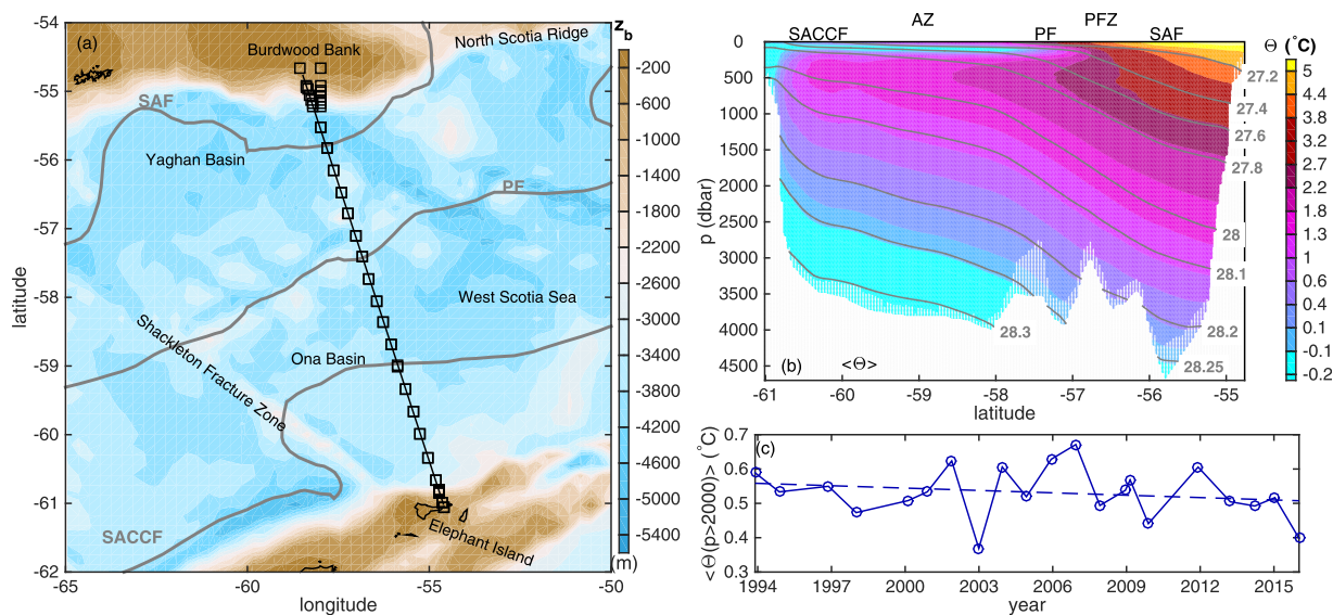
Figure 1. (a) Nominal SR1b hydrographic stations (squares) and line, with climatological locations (gray) of the Subantarctic Front (SAF), Polar Front (PF), and Southern ACC Front (SACCF) [Orsi et al., 1995] and bathymetry (color contours, [Arndt et al., 2013; Smith and Sandwell, 1997]). (b) Latitude-depth section of SR1b mean conservative temperature \bar{\Theta} (filled color contours) and mean neutral density \bar{\sigma}_\theta (dark gray contours), with indicative front locations based on the SR1b time-mean temperature and salinity sections marked at top along with the Antarctic Zone (AZ) and Polar Frontal Zone (PFZ). (c) Time series of \bar{\Theta} averaged over the area deeper than 2000 dbar (blue solid line and circles), with the linear trend (dashed line). The white shading near the bottom in Figure 1b marks the area where the isopycnal/heave decomposition does not produce values at certain times (see section 3); these areas are not included in the spatially averaged time series.
