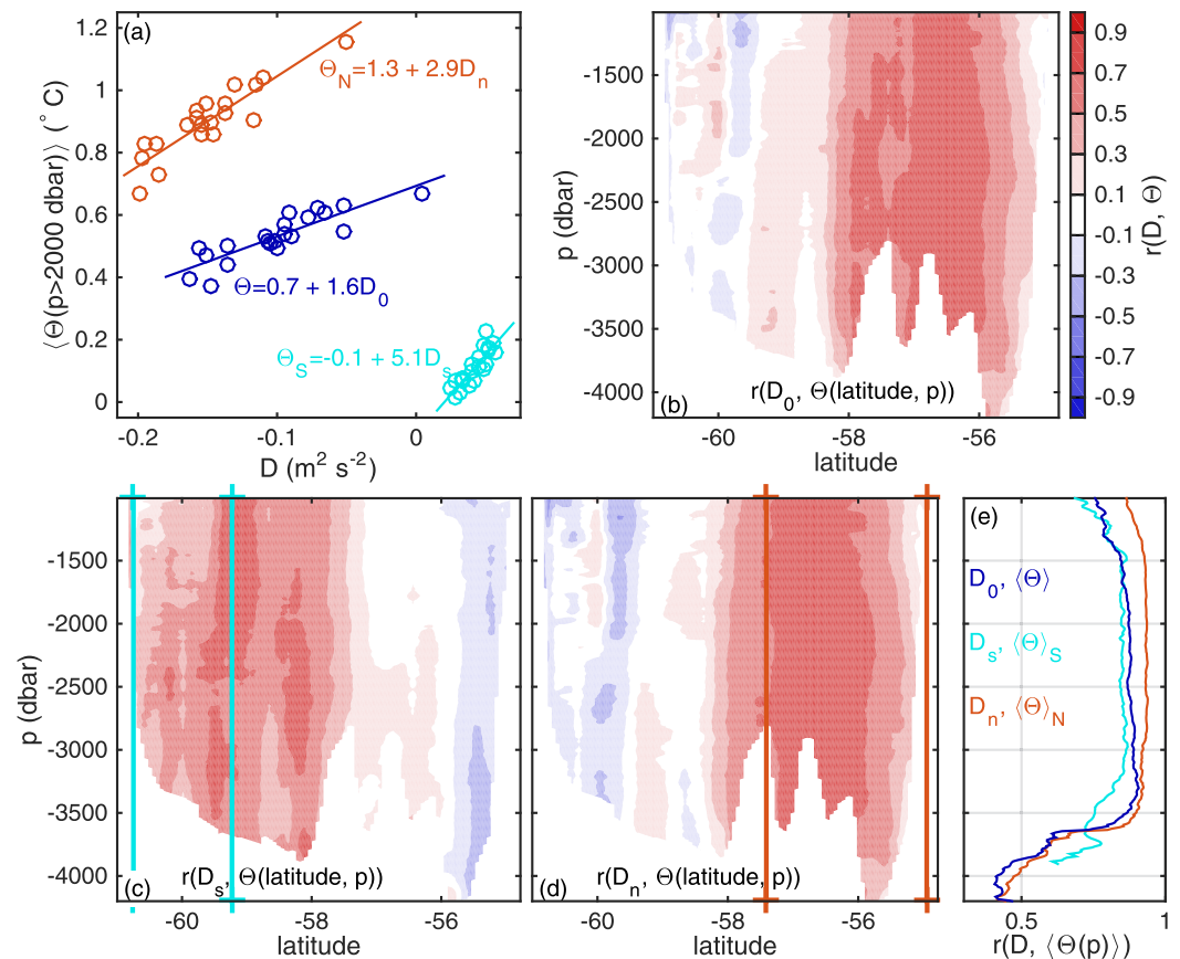
Figure 6. Correlations between \Theta and frontal position proxy D . (a) \Theta deeper than 2000 dbar averaged across the section, plotted against integrated frontal position proxy D_0 (dark blue); \Theta south of 58^{\circ}\text{S} ( \Theta_S ), plotted against southern frontal position proxy D_s (cyan); \Theta north of 58^{\circ}\text{S} ( \Theta_N ), plotted against northern frontal position proxy D_n (orange), with best fit lines as labeled. Correlations between (b) \Theta(y, p, t) and D_0(t) ; (c) \Theta(y, p, t) and D_s(t) ; and (d) \Theta(y, p, t) and D_n(t) . Cyan lines in (c) and orange lines in (d) mark the limits of integration for D_s and D_n , respectively. (e) Profiles of correlations for conservative temperature averaged along pressure surfaces: correlations between \Theta(y, t) and D_0(t) (dark blue); \Theta_S(y, t) and D_s(t) (cyan); and \Theta_N(y, t) and D_n(t) (orange).
