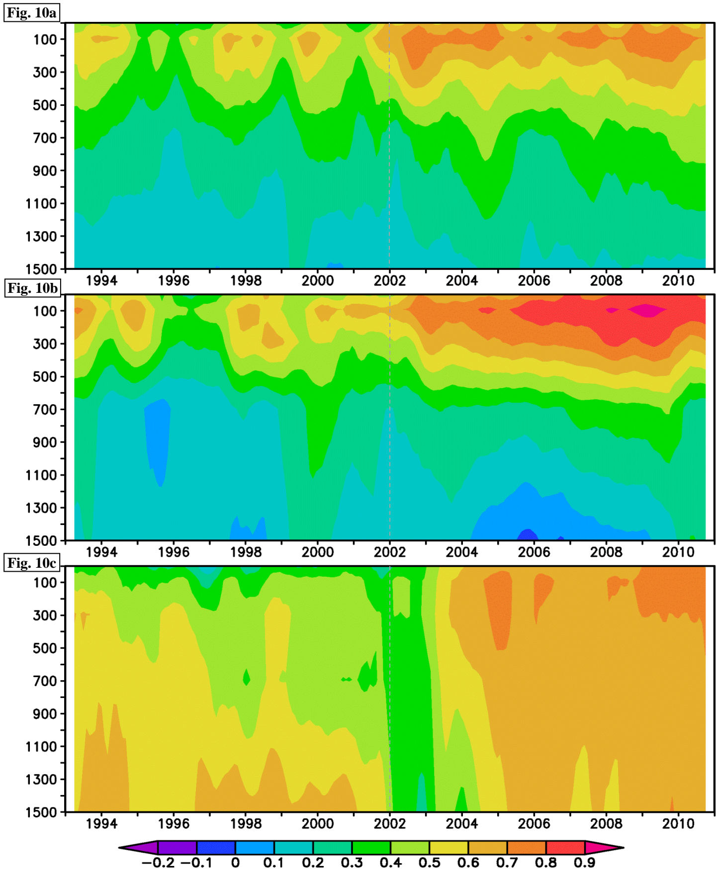
Fig. 10: (a) Centred pattern correlation coefficients (i.e. CPCOR ; calculated over the band area 0-360°E; 30°N-60°N) of salt anomalies between EMORA and EMOO as a function of depth (0-1500m) and time (1993-2010). Prior to plotting a 7-month running mean was applied on the computed correlation coefficients to remove the intra-seasonal variability. The ordinate has units meter (m). (b) Same as in (a), except for the band area 0-360°E; 15°S-15°N. (c) Same as in (a), except for the band area 0-360°E; 60°S-30°S.
