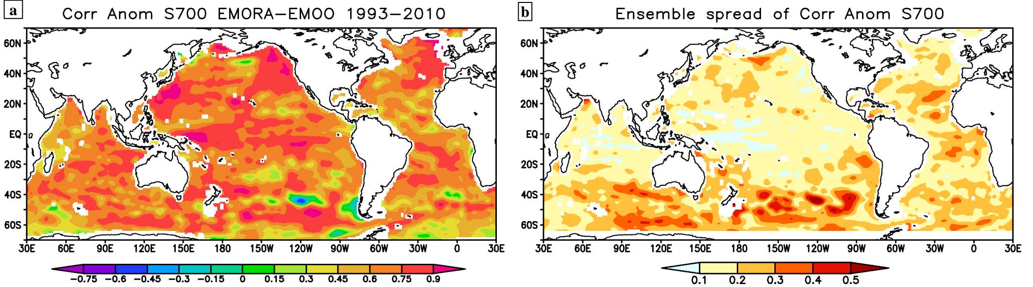
Fig. 6: (a) Temporal correlation coefficients of S700 anomalies between EMORA and EMOO for the period 1993-2010. (b) Ensemble spread (i.e. SPD_{EMORA}^{COR} ) of correlation coefficients of S700 anomalies between individual ORAs and EMOO about their mean correlation coefficients.
