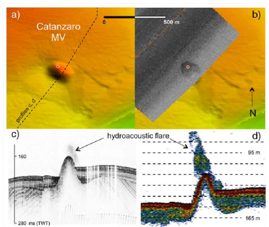
FIG 3. integrated acoustic methods to detect active seepage at the Catanzaro mud volcano (Ionian margin). a) multibeam bathymetry; b) backscatter mosaic superimposed on bathymetry data; c) subbottom data showing an acoustic flare in the water column; d) echo sounder single beam data showing the flare in the water column above the mud volcano. The Catanzaro mud volcano has not
