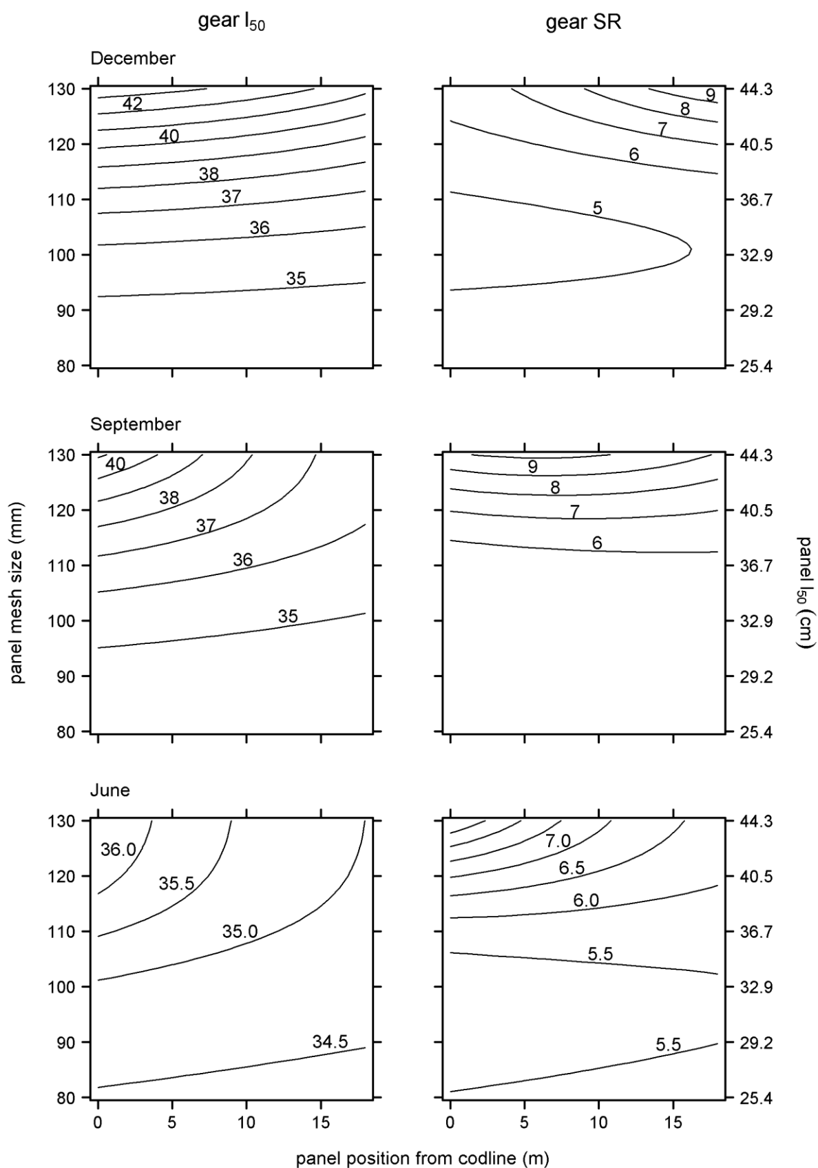
Figure 4.2.2.3 Output from the model of Fryer et al (2016) showing the effect of the square mesh panel mesh size and position on gear L50 (left) and SR (right) for a typical Scottish trawler targeting white fish in December (top), September (middle) and June (bottom)
