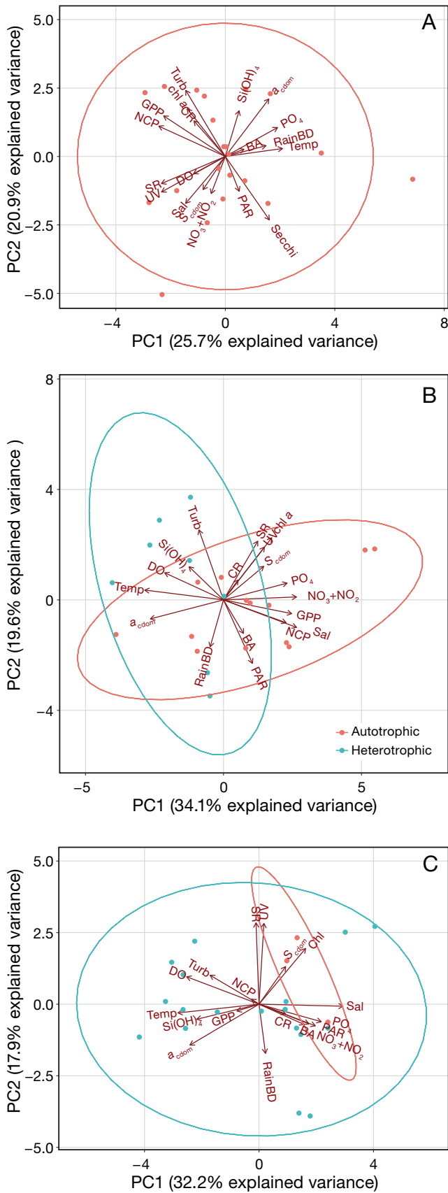
Fig. 4. Biplots of results from principal components analysis (PCA) at (A) 1 m, (B) 7 m and (C) 12 m depth on environmental parameters (seawater temperature [Temp]; salinity [Sal]; cumulative rain the day before the sampling [RainBD]; UV dose [UV]; solar radiation [SR]; photosynthetically active radiation reaching corresponding depth [PAR]; turbidity [Turb]; Secchi depth [Secchi]; nitrate + nitrite concentration [NO 3 +NO 2 ]; phosphate concentration [PO 4 ]; silicate concentration [Si]; dissolved oxygen concentration [DO]; magnitude of coloured dissolved organic matter absorption [a CDOM ]; spectral slope of the a CDOM (λ) spectrum [S CDOM ] and biological parameters (chlorophyll a concentration [chl a]; bacterial abundance [BA]; gross primary production [GPP]; net community production [NCP]; community respiration [CR]). Secchi depth was represented only for surface PCA. When the volumetric NCP rates are <0, the dots are in blue (heterotrophic) and when volumetric NCP rates are >0, the dots are in pink (autotrophic). The blue and pink ellipses encompass 95% of the data that are heterotrophic and autotrophic, respectively
