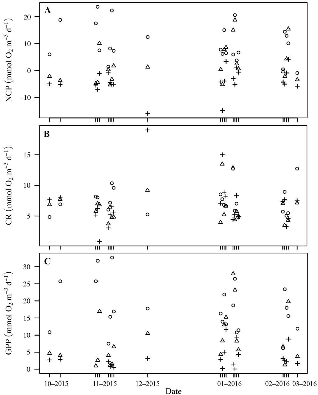
Fig. 3. Variation over sampling time of volumetric (A) net community production (NCP), (B) community respiration (CR) and (C) gross primary production (GPP) for the 3 sampled depths (circles: 1 m; triangles: 7 m; plus signs: 12 m). Each tick mark on x-axis represents a sampling event (e.g. in October 2015, seawater was sampled on 2 days; in November 2015, on 7 days)
