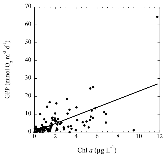
Fig. 7. The relationship between gross primary production (GPP) and chlorophyll a concentration. The solid line shows the fitted regression equation \text{GPP (mmol O}_2 \text{ m}^{-3} \text{ d}^{-1}) = 0.30 + 2.26 (\pm 0.29) \text{ chl } a (\mu\text{g chl } a \text{ L}^{-1}) ( R^2 = 0.38 , p < 0.0001 , N = 98 ).
