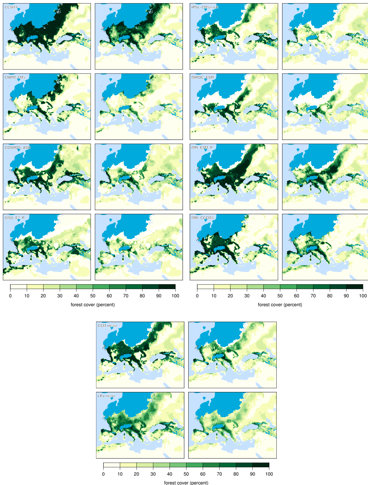
Fig. S1. Tree cover in simulations with and without human burning. Tree cover fraction simulated by LPJ-LMfire using each of the eight GCM LGM climate simulations without human burning ( left panels ) and with human burning ( right panels ). LPJ-LMfire results are also shown for a simulation using the multi-model ensemble mean climate ( GCM mean ), and the mean of all of the individual LPJ-LMfire simulations ( LPJ mean ).
