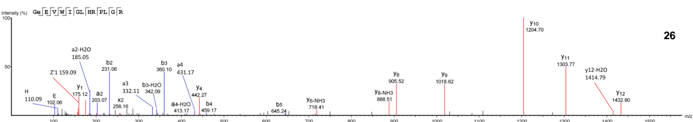
10-26: Product ion spectra (raw spectra manually annotated on the basis of PEAKS assignments) of all the York/Oxford identified sequences (see panel 1).
