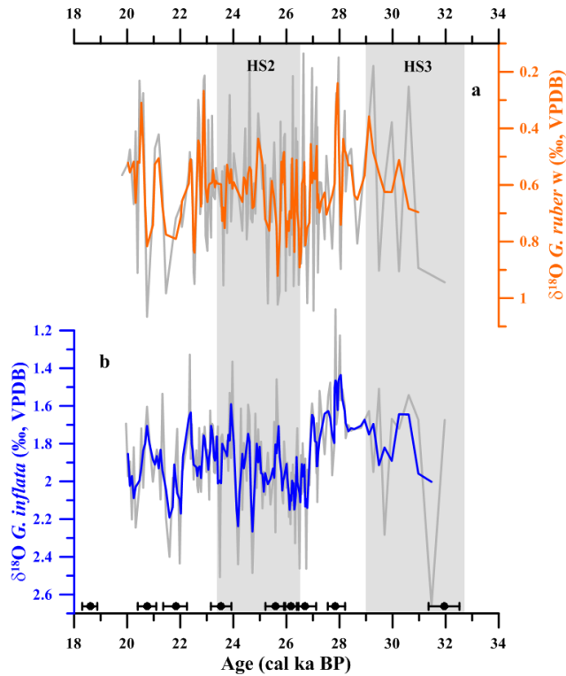
5 Figure 1: Stable oxygen isotopic ( \delta^{18}\text{O} ) records from sediment core GeoB6212-1. (a) Globigerinoides ruber white ( G. ruber w ) \delta^{18}\text{O} and (b) Globorotalia inflata ( G. inflata ) \delta^{18}\text{O} . Orange and blue lines represent three–point running averages for G. ruber w and G. inflata , respectively. Black symbols at the bottom of the panel depict calibrated ages. Grey vertical bars show abrupt millennial–scale climate change events Heinrich Stadial 3 (HS3) and Heinrich Stadial 2 (HS2) (Goni and Harrison, 2010; Sarnthein et al., 2001).
