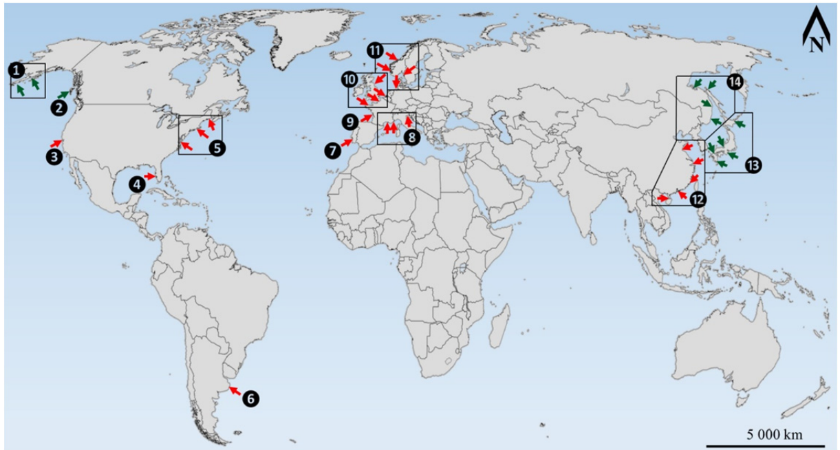
Figure 1. World-wide distribution of Gonionemus vertens from literature (Table S2). Green arrows : native areas. Red arrows : introduced populations. ❶ to ❿❹ : numbered locations.
