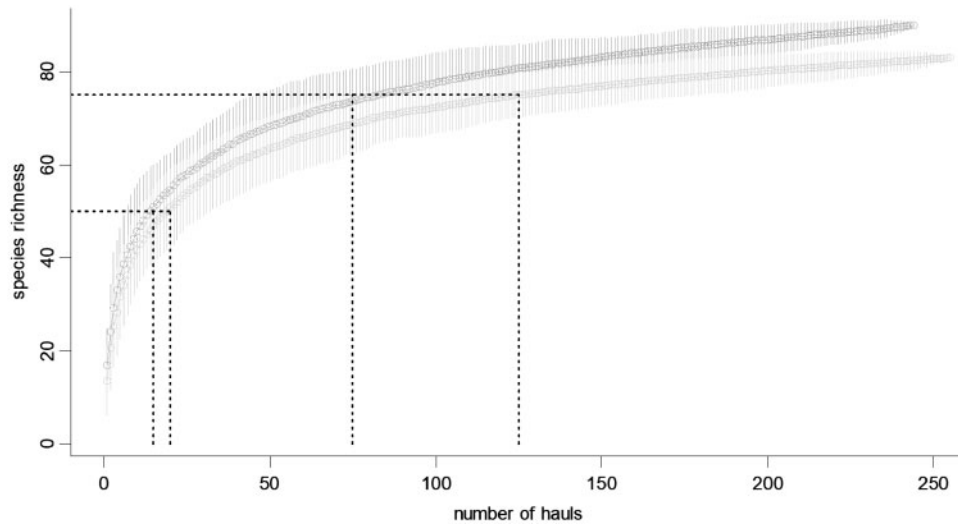
Figure 2. Cumulative species richness curves for long tows in dark grey and short tows in light grey. The black dotted lines show that to reach a species richness of 50 species, ~15 tows in the “long” or 20 tows in the “short” tow category are needed (33% increase in effort). Whereas to reach a species richness of 75 species, using the “long” tow category ~75 tows are needed and using the “short” tow category ~125 tows are needed (67% increase in effort). Vertical lines provide the standard deviation from random permutations of the data.
