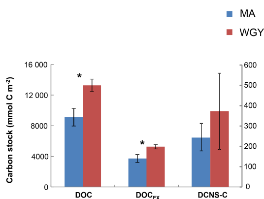
Figure 6. Integrated carbon stocks (mmol C m -2 ) over the euphotic zone carbon in terms of DOC, DOC EX and DCNS-C (secondary axis). * DOC and DOC SL were statistically different between MA and WGY areas (Mann–Whitney test, p < 0.05 ).
