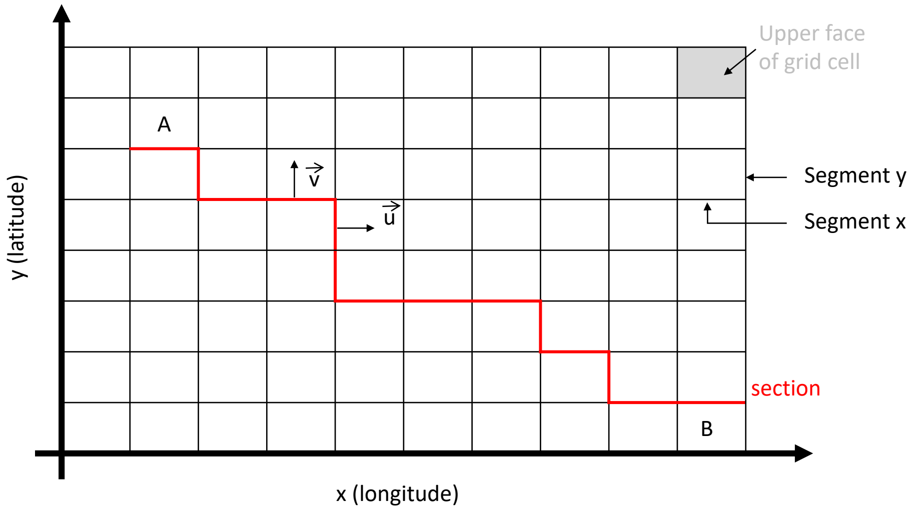
Fig. S1: Schematic representation of the OVIDE section in the model.
