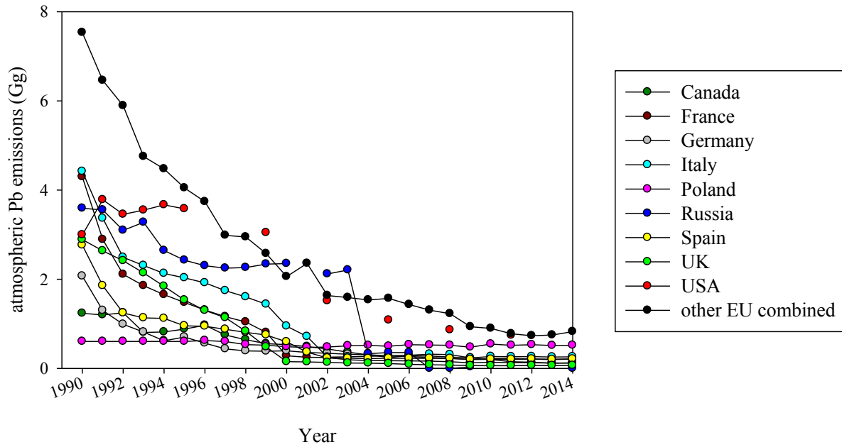
Figure S3: Atmospheric emissions by nation, 1990 – 2014 (EMEP, 2017). Other EU combined nations include: Albania, Armenia, Austria, Azerbaijan, Belarus, Belgium, Bulgaria, Croatia, Cyprus, Czech Republic, Denmark, Estonia, Finland, Georgia, Greece, Hungary, Ireland, Kazakhstan, Kyrgyzstan, Latvia, Liechtenstein, Lithuania, Luxembourg, Malta, Monaco, Montenegro, Netherlands, Norway, Portugal Republic of Moldova, Romania, Serbia, Slovakia, Slovenia, Sweden, Switzerland, the former Yugoslav Republic of Macedonia, Turkey, and Ukraine.
