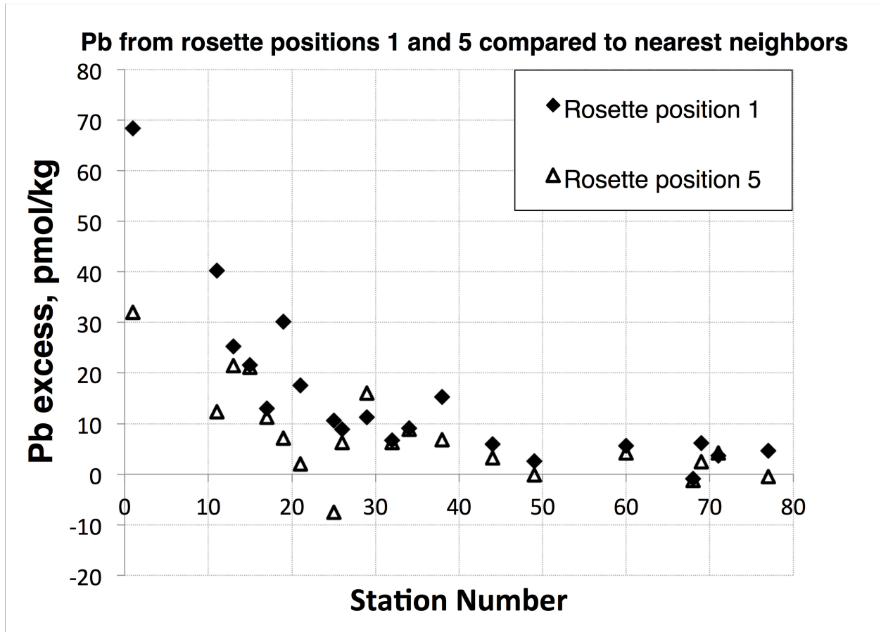
Figure S1: Plot of the difference in Pb concentration between GoFlo bottles 1 and 5 and their nearest respective bottles shows a wash-out effect.
