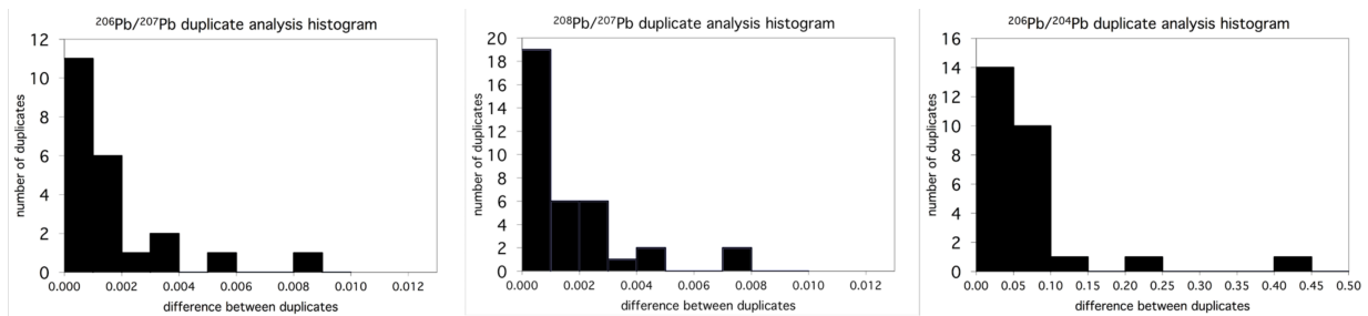
Figure S2: Replicate Pb isotope analyses: histogram of difference between duplicates.
