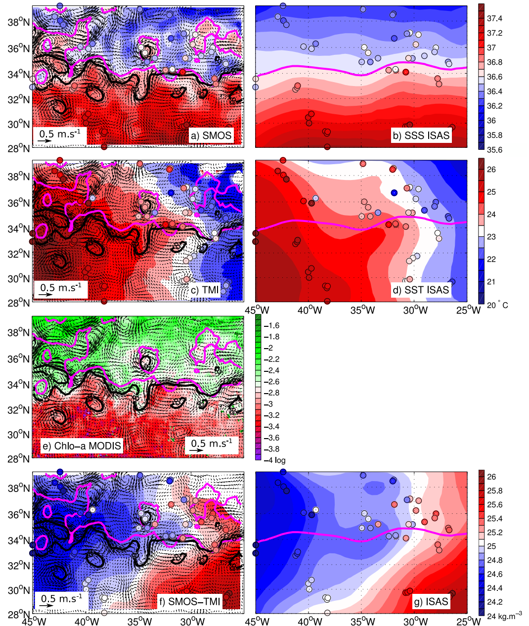
Figure 10. July 2011 monthly mean surface salinity from (a) SMOS and (b) ISAS, surface temperature in ^{\circ}\text{C} from (c) TMI and (d) ISAS, (e) MODIS sea surface chlorophyll-a concentration in \log(\text{kg m}^{-3}) , and surface density in \text{kg m}^{-3} from (f) SMOS/TMI and (g) ISAS. Arrows are the monthly mean geostrophic surface velocities from AVISO (in \text{m s}^{-1} ). Thick black and magenta contours and colored circles are the same as in Figure 7.
