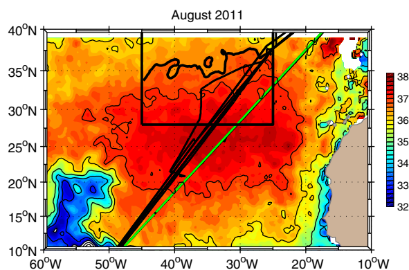
Figure 1. August 2011 SSS map from monthly SMOS smoothed data at 100 \times 100 \text{ km}^2 in the Subtropical-tropical Atlantic. The 14 TSG transects (black tracks) across the SSS maximum from June 2010 and October 2011 and one between 7 and 15 August 2011 (green track). The 28^\circ\text{N}\text{--}40^\circ\text{N}/45^\circ\text{W}\text{--}25^\circ\text{W} box is depicted in a thick black line, and the thick black contour within the box shows the 36.6 isohaline chosen to illustrate the Azores Front/Current. The isohaline contours are shown in thin black line contour. C.I. = 1.
