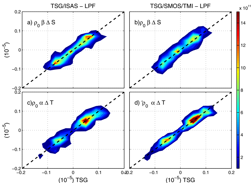
Figure 3. Probability Density Function (PDF; in color) of 500 km Butterworth low-pass filtered (a) TSG SSS gradient versus collocated ISAS SSS gradient; (b) TSG SSS gradient versus collocated SMOS SSS gradient; (c) TSG SST gradient versus collocated ISAS SST gradient; and (d) TSG SST gradient versus collocated TMI SST gradient. The calculation has been done for the 14 TSG transects available between July 2010 and December 2011 listed in the Table 1.
