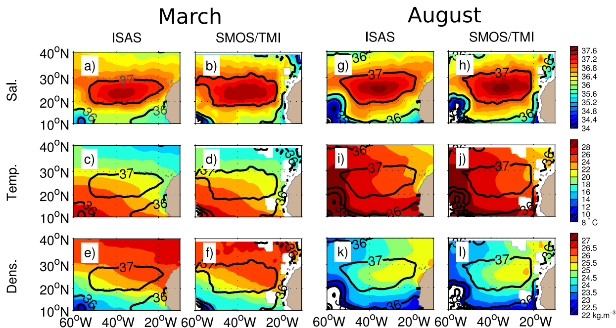
Figure 4. March and August (a, b, g, and h) mean surface salinity, (c, d, i, and j) temperature in °C, (e, f, k, and l) density in \text{kg m}^{-3} computed from (left column) ISAS and (right column) SMOS/TMI products smoothed over 3 \times 3^\circ between July 2010 and December 2012. The black contours represent the mean March (Figures 4a–4f) and August (Figures 4g–4l) salinity. Note that, the white squares of missing data in filtered fields correspond to island contaminations.
