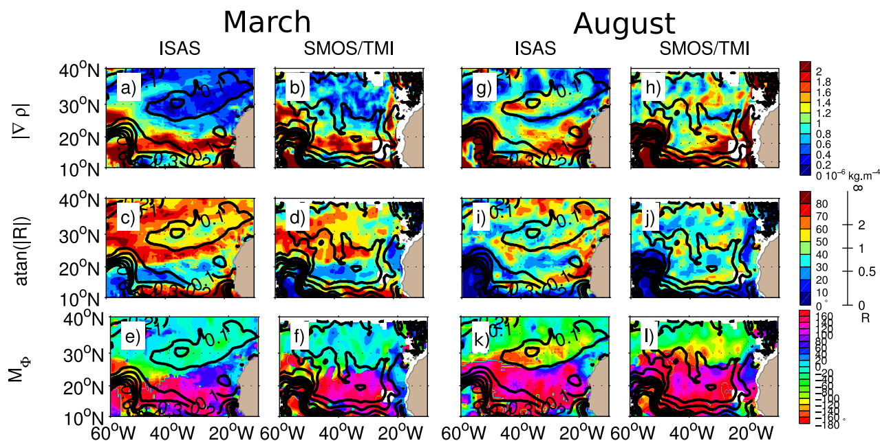
Figure 5. March and August median norm of the (a, b, g, and h) near-surface density gradient in \text{kg m}^{-4} , (c, d, i, and j) density ratio \text{atan}(|R|) in degrees with the corresponding |R| scale, (e, f, k, and l) mean angle M_\phi of thermohaline gradient in degrees between July 2010 and December 2012. The black contours represent the salinity seasonal standard deviation. Note that, the white squares of missing data in filtered fields correspond to island contaminations.
