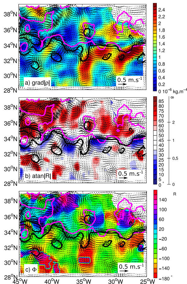
Figure 11. Same as Figure 9, except for July 2011.
