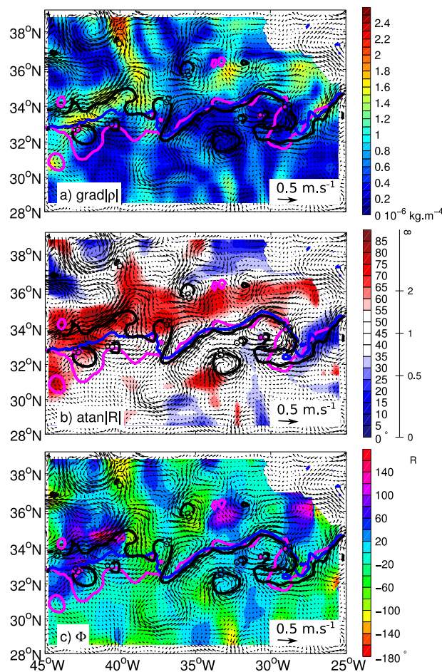
Figure 9. March 2012 monthly SMOS/TMI (a) density gradient surface salinity in \text{kg m}^{-4} , (b) norm of the density ratio \text{atan}|R| in ^\circ , and (c) angle( R ) between temperature and salinity gradient vector in ^\circ . Arrows indicate the monthly mean geostrophic surface velocities from AVISO (in \text{m s}^{-1} ). Thick black, magenta, and blue contours are the same as in Figure 7.
