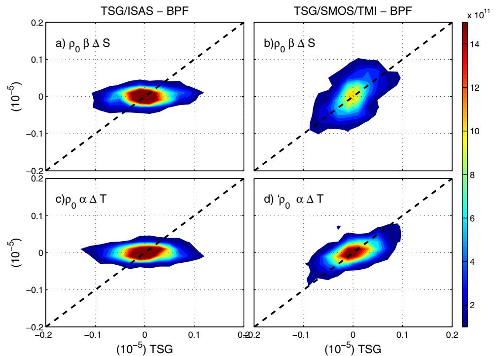
Figure 7. Probability Density Function (PDF; in color) of 200–500 km Butterworth-band pass filtered (a) TSG SSS gradient versus collocated ISAS SSS gradient, (b) TSG SSS gradient versus collocated SMOS SSS gradient, (c) TSG SST gradient versus collocated ISAS SST gradient, and (d) TSG SST gradient versus collocated TMI SST gradient. The calculation was done for the 14 TSG transects available between July 2010 and December 2011 listed in the Table 1.
