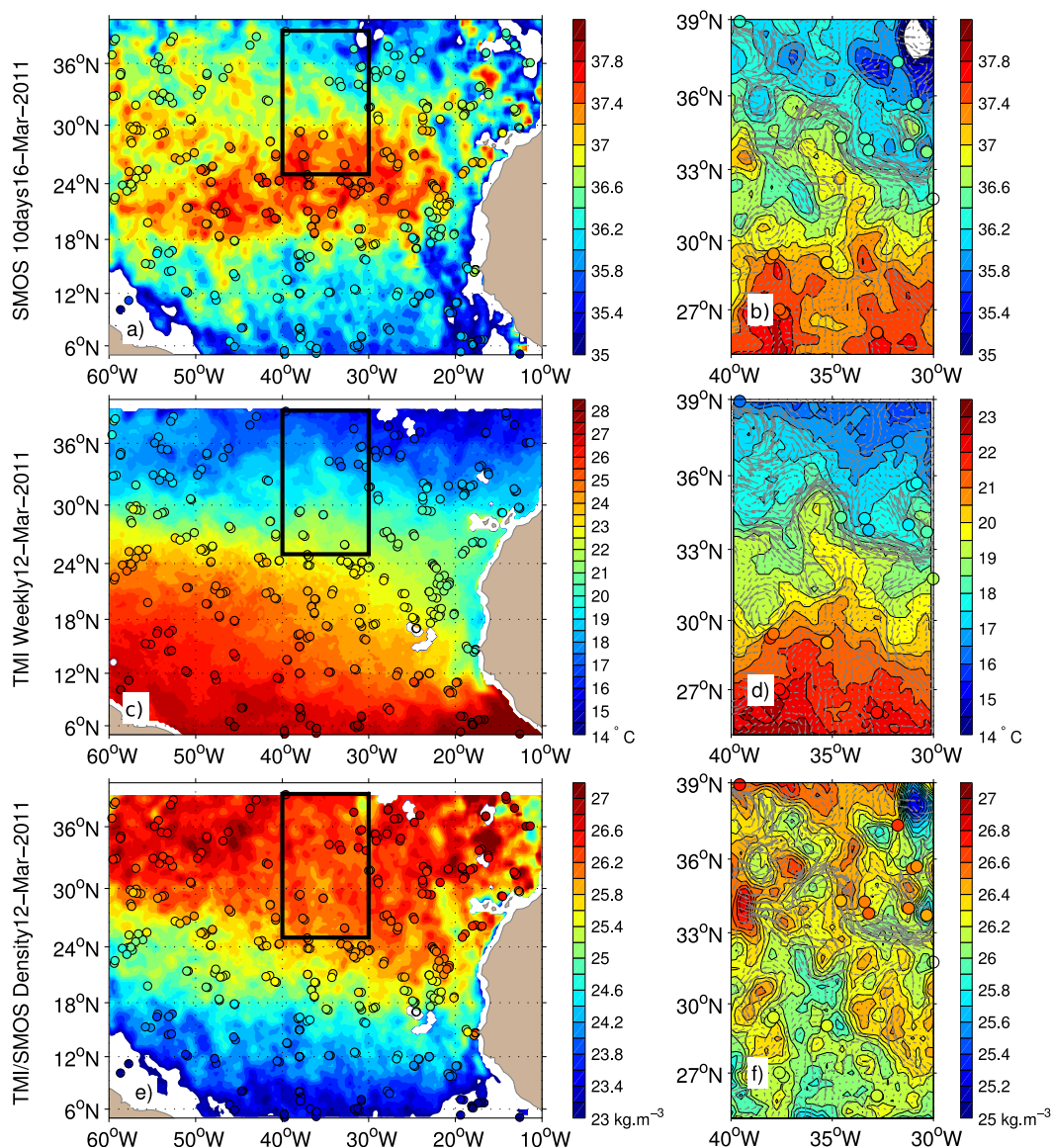
Figure 12. (a and b) SMOS SSS 10 day mean; (c and d) TMI SST weekly mean in °C, and (e and f) density computed from SMOS and TMI in \text{kg m}^{-3} taken from satellite measurements between 11–21 March 2011 and 10–17 March 2011, respectively. The black square delimits the region 25°N–39°N and 40°W–30°W (Figures 12b, 12d, and 12f). The colored circles represent the individual Argo temperature and salinity near-surface measurements taken at about 5 m depth between 11 and 21 March 2011. Gray arrows present the geostrophic surface velocities deduced from AVISO in \text{m s}^{-1} averaged between 11 and 21 March 2011.
