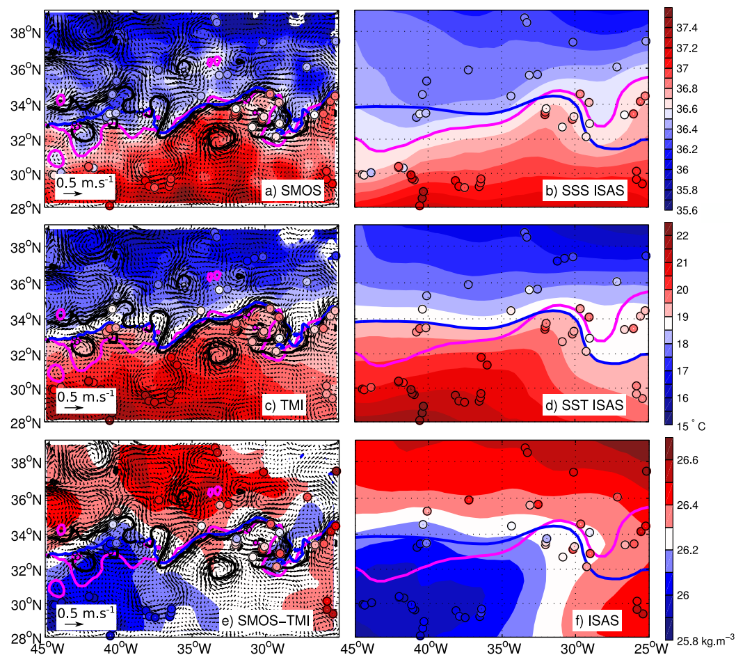
Figure 8. March 2012 monthly mean surface salinity from (a) SMOS and (b) ISAS, surface temperature in °C from (c) TMI (d) ISAS, and surface density in \text{kg m}^{-3} from (e) SMOS/TMI and (f) ISAS. Arrows are monthly mean geostrophic surface velocities (in \text{m s}^{-1} ) from AVISO. The thick black contour corresponding to the 8 \times 10^{-5} \text{ s}^{-2} vorticity isoline identifies the Azores Front/Current ( \text{vort} = f + \zeta ; where f is the planetary vorticity and \zeta is the relative vorticity computed as \zeta = \partial v/\partial x - \partial u/\partial y ). The thick magenta (blue) contours corresponding to the 36.6 isohaline (19°C isotherm) identify the thermohaline front associated with the Azores front. Colored circle are at the Argo float position and the corresponding near-surface (~5 m depth) salinity, temperature, and salinity values.
