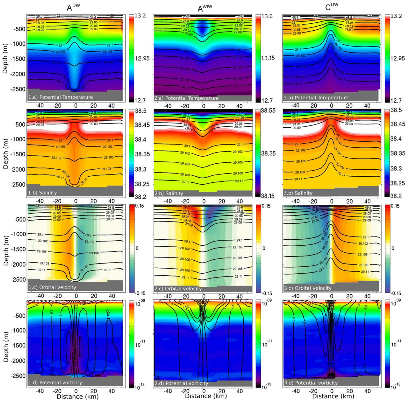
Figure 7. Composite transects of (left column) anticyclone A^{DW} , (middle column) anticyclone A^{WIW} , and (right column) cyclone C^{DW} : (a) potential temperature, (b) salinity, (c) orbital velocities with potential density anomaly contours, and (d) the potential vorticity with orbital velocity contours. The composite images were obtained by averaging west-east and south-north transects crossing the core of each structure at each model output. Color scales are chosen to highlight the hydrographical core of each eddy. The gray shaded area represents the seabed.
