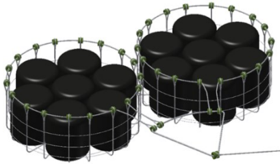
Figure 61 – Anchor bags and fairlead by TTI. ©TTI Ltd.
