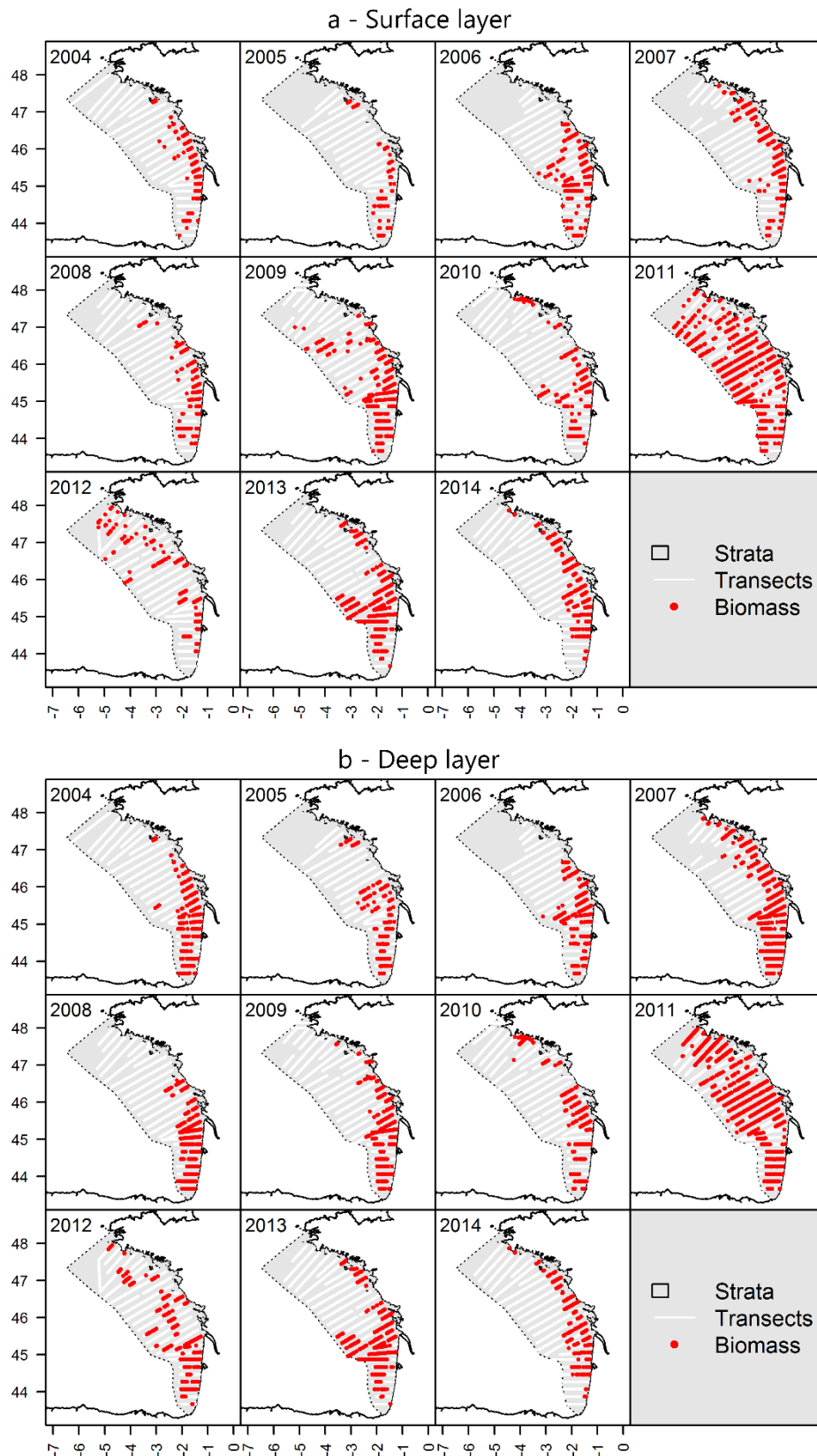
Figure B1 – Distributions of acoustic detections of small pelagic fishes smaller than 10 cm in the surface layer (a) and deep layer (b).
