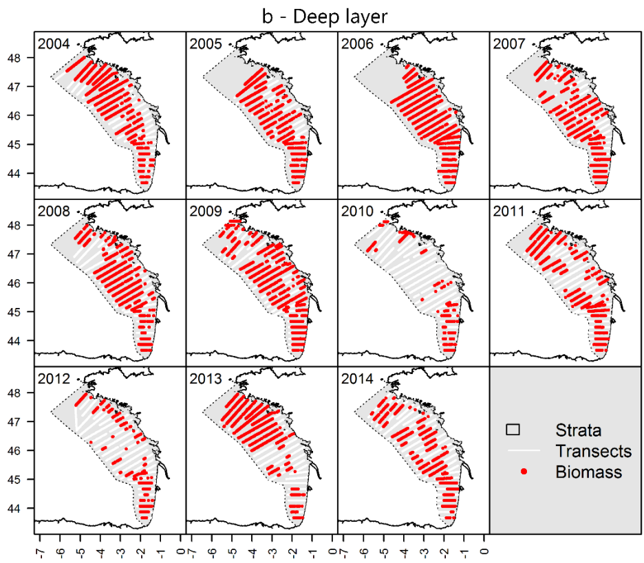
Figure B3 – Distributions of acoustic detections of small pelagic fishes between 20 and 30 cm long in the surface layer (a) and deep layer (b).
