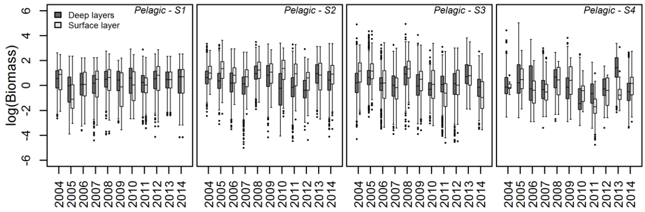
Figure B5 – Biomass (log) of the four size classes of small pelagic fishes (S1: <10 cm; S2: 10-20 cm ; S3: 20-30 cm; S4: >30 cm) detected within the Bay of Biscay between 2004 and 2014 for the surface and deep layers.
