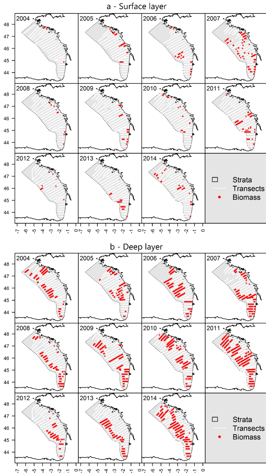
Figure B4 – Distributions of acoustic detections of small pelagic fishes larger than 30 cm in the surface layer (a) and deep layer (b).
