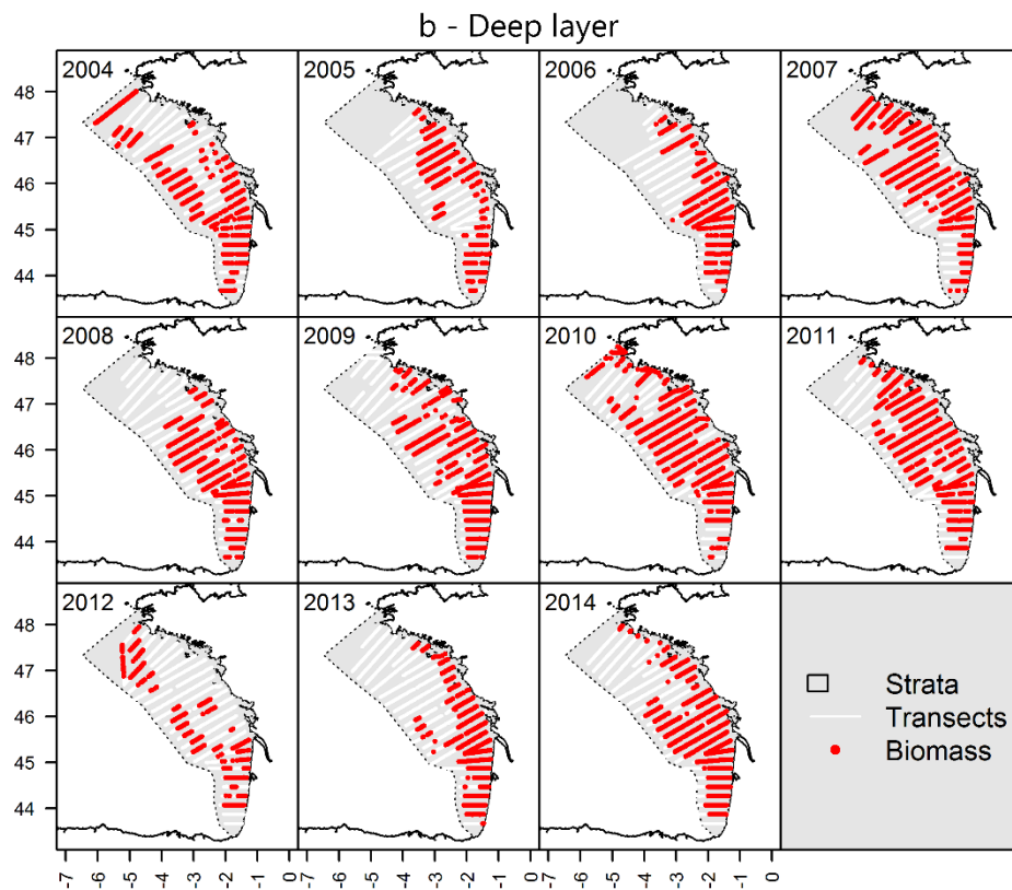
Figure B2 – Distributions of acoustic detections of small pelagic fishes between 10 and 20 cm long in the surface layer (a) and deep layer (b).
