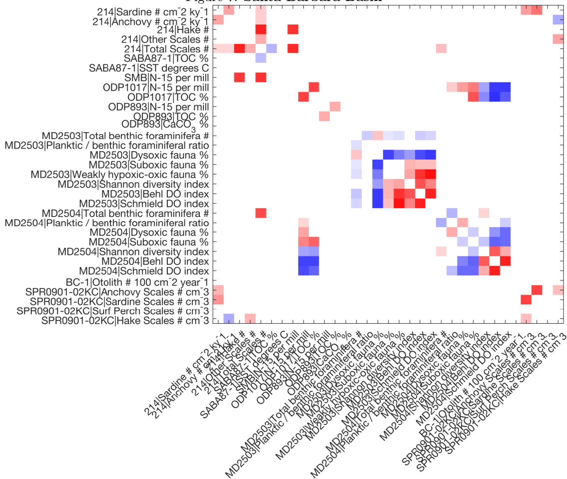
Figure 7: Santa Barbara Basin
