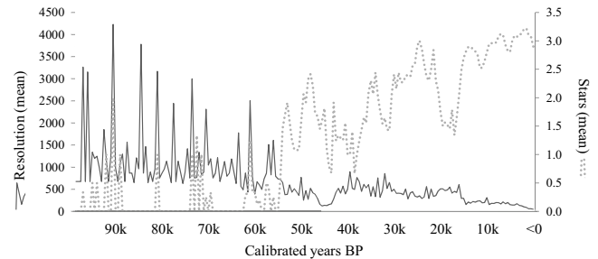
Figure 5. Changing mean sample resolution (left) and mean number of stars (right) of the pollen database of northwest South America during the period 100 kcal to –50 cal yr BP.
