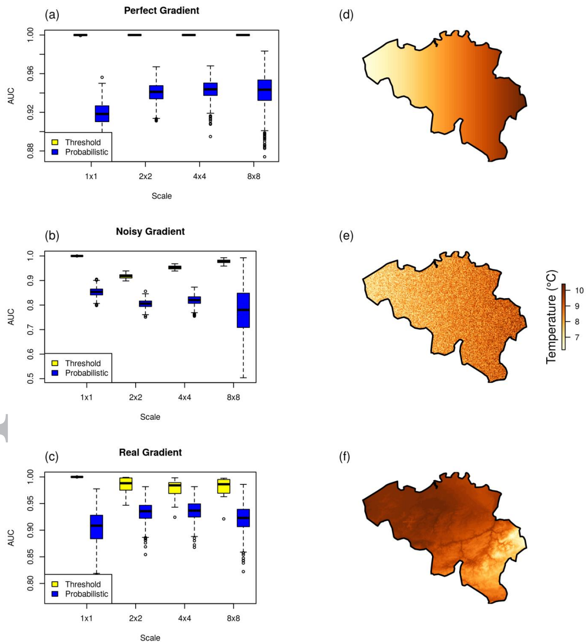
Figure 4: AUC as a function of resolution in an up-scaling VS exercise in (a) a simulated perfect east-to-west gradient of temperature, (b) a gradient with random noise built on top of the east-to-west gradient, and (c) a real gradient corresponding to mean annual temperature in Belgium. The corresponding maps of each gradients are represented in (d), (e) and (f). Boxplots represent results of a threshold simulation approach in yellow, and a probabilistic simulation approach in blue.
