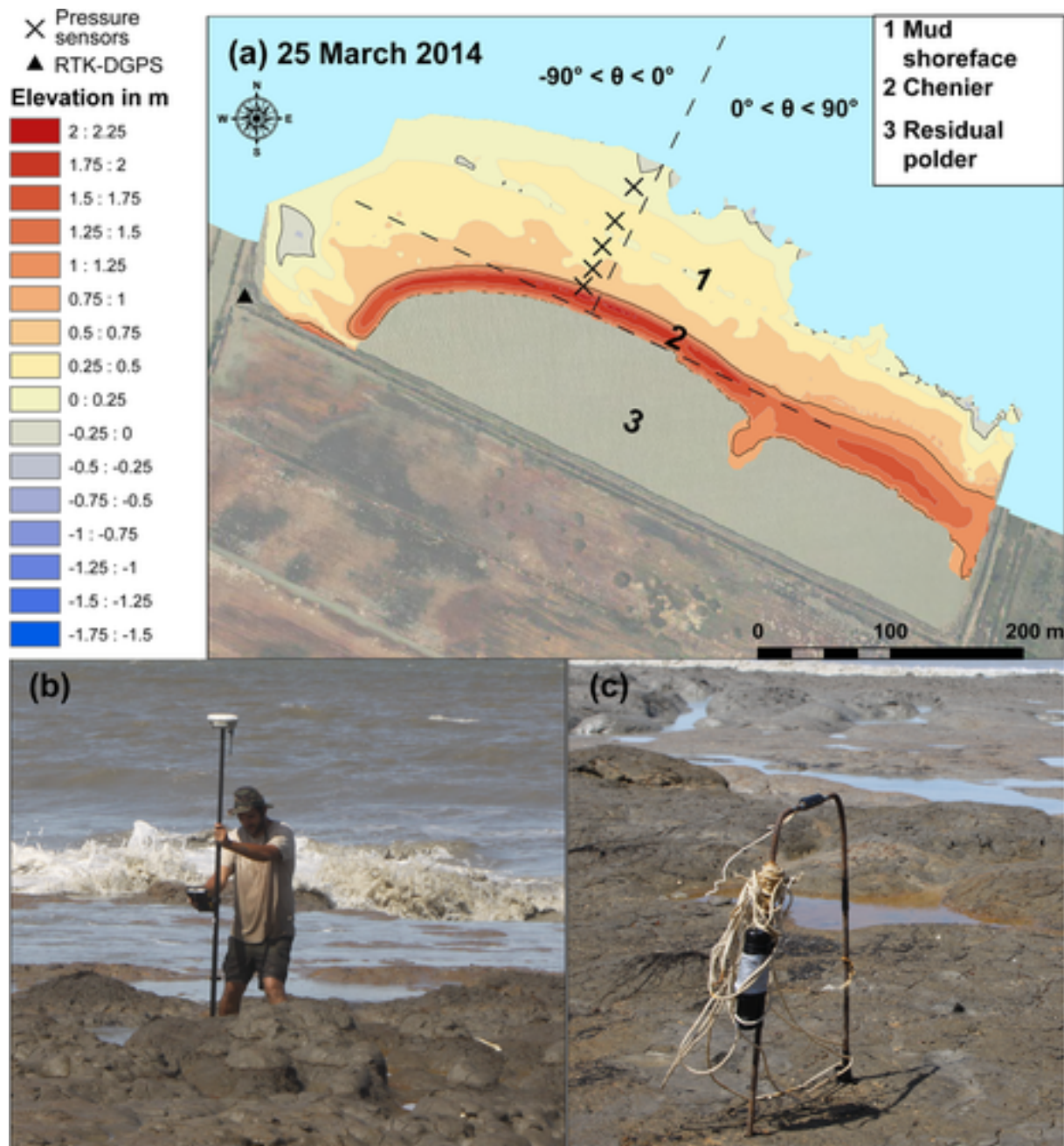
Figure 3 Field survey methods: (a) example of a DEM produced from field surveys using RTK-DGPS (b). The cross-shore profile shown was used to determine the wave incidence \theta from wave direction. Pressure sensors (c) were deployed along a cross-shore transect on the mud foreshore subject to wave attack.
